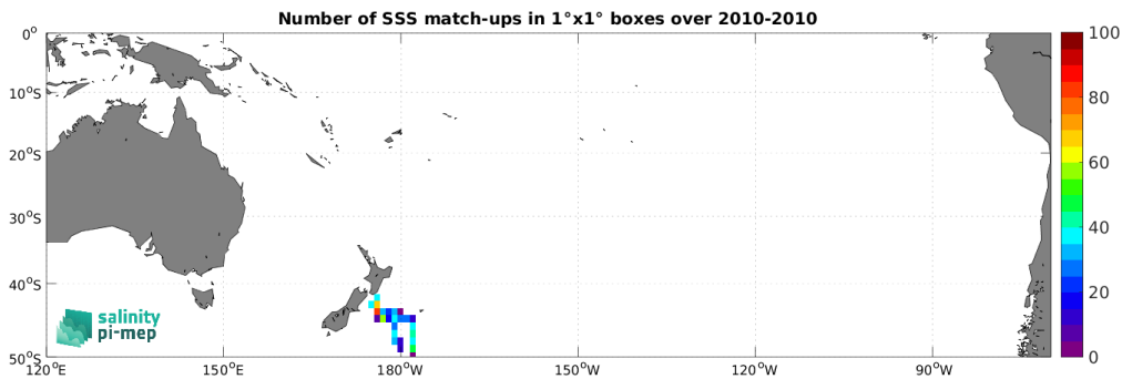
Figure 4: Number of SSS match-ups between TSG (Polarstern) SSS and the SMOS SSS L3 v9 - 18 Days (CATDS-CEC-LOCEAN) SSS product for the South Pacific Ocean Pi-MEP region over 1^\circ \times 1^\circ boxes and for the full satellite product period.
