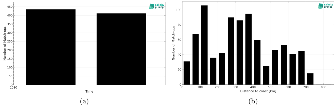
Figure 1: Number of match-ups between TSG (Polarstern) and SMOS SSS L3 v9 - 18 Days (CATDS-CEC-LOCEAN) SSS as a function of time (a) and as function of the distance to coast (b) over the South Pacific Ocean Pi-MEP region and for the full satellite product period.
