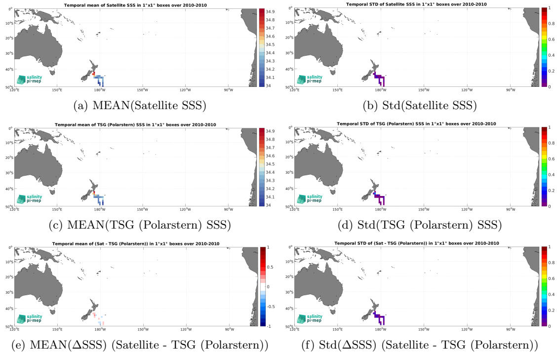
Figure 6: Temporal mean (left) and Std (right) of SSS from SMOS SSS L3 v9 - 18 Days (CATDS-CEC-LOCEAN) (top), TSG (Polarstern) (middle), and of \Delta SSS (Satellite - TSG (Polarstern)). Only match-up pairs are used to generate these maps.
