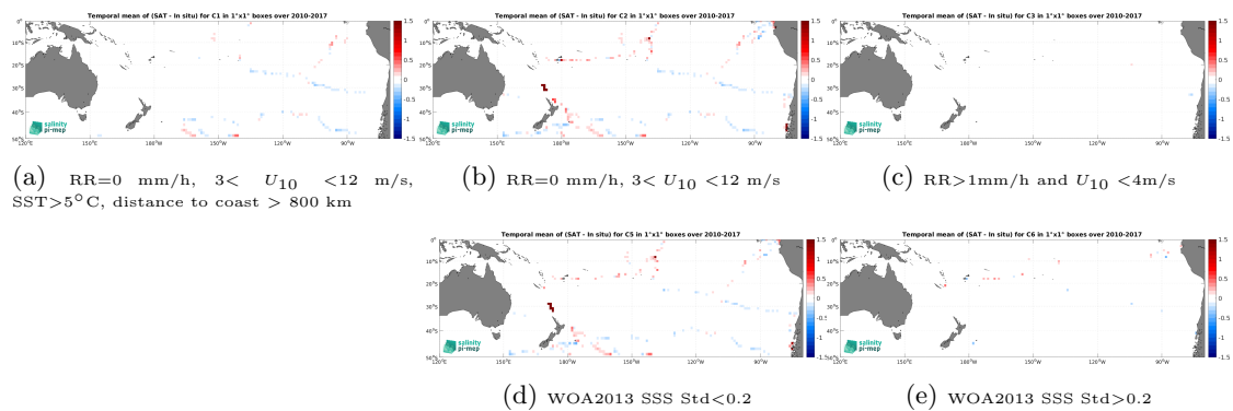
Figure 14: Temporal mean gridded over spatial boxes of size 1^\circ \times 1^\circ of \Delta\text{SSS} (SMOS SSS L3 v9 - 18 Days (CATDS-CEC-LOCEAN) - TSG (GOSUD-Sailing-ship)) for 5 different subdatasets corresponding to:RR=0 mm/h, 3 < U_{10} < 12 m/s, SST >5^\circ\text{C} , distance to coast > 800 km (a), RR=0 mm/h, 3 < U_{10} < 12 m/s (b), RR >1 mm/h and U_{10} < 4 m/s (c), WOA2013 SSS Std <0.2 (d), WOA2013 SSS Std >0.2 (e).
