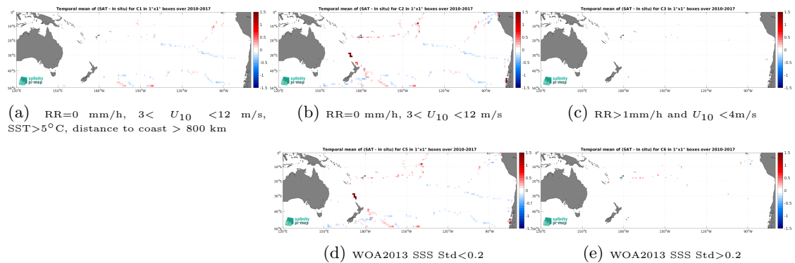
Figure 14: Temporal mean gridded over spatial boxes of size 1^\circ \times 1^\circ of \Delta SSS (SMOS SSS L3 v9 - 18 Days (CATDS-CEC-LOCEAN) - TSG (GOSUD-Sailing-ship)) for 5 different subdatasets corresponding to:RR=0 mm/h, 3 < U_{10} < 12 m/s, SST >5^\circ C, distance to coast > 800 km (a), RR=0 mm/h, 3 < U_{10} < 12 m/s (b), RR >1 mm/h and U_{10} < 4 m/s (c), WOA2013 SSS Std <0.2 (d), WOA2013 SSS Std >0.2 (e).
