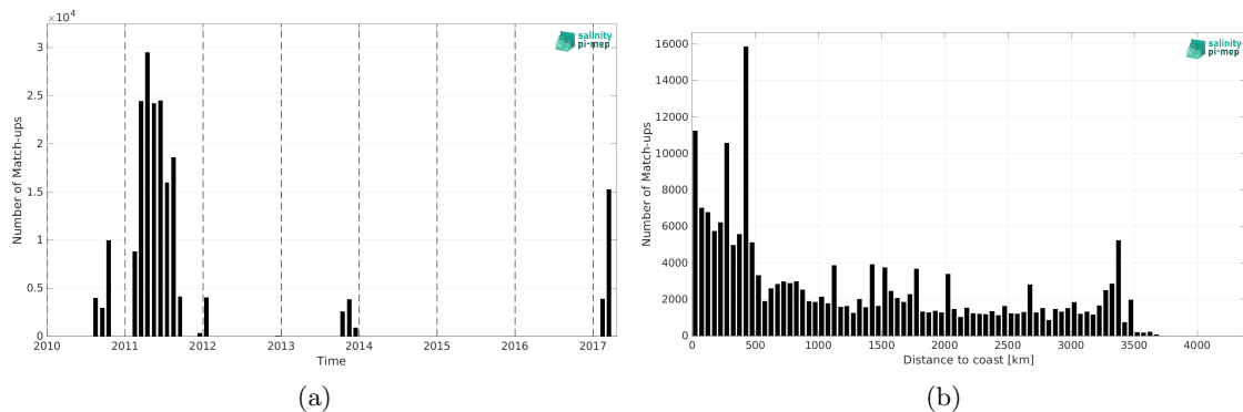
Figure 2: Number of match-ups between TSG (GOSUD-Sailing-ship) and SMOS SSS L3 v9 - 18 Days (CATDS-CEC-LOCEAN) SSS as a function of time (a) and as function of the distance to coast (b) over the South Pacific Ocean Pi-MEP region and for the full satellite product period.
