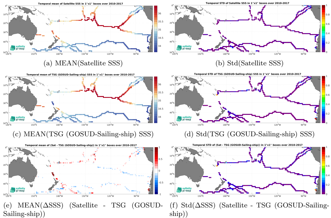
Figure 7: Temporal mean (left) and Std (right) of SSS from SMOS SSS L3 v9 - 18 Days (CATDS-CEC-LOCEAN) (top), TSG (GOSUD-Sailing-ship) (middle), and of \Delta SSS (Satellite - TSG (GOSUD-Sailing-ship)). Only match-up pairs are used to generate these maps.
