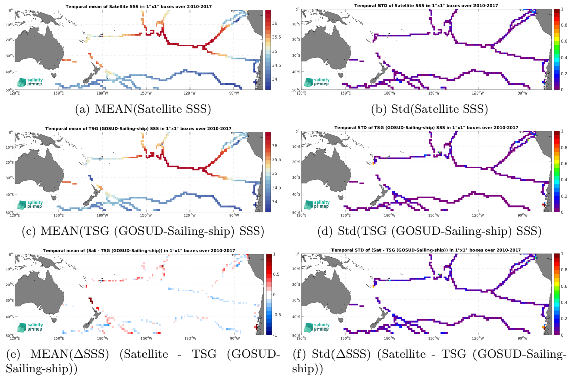
Figure 6: Temporal mean (left) and Std (right) of SSS from SMOS SSS L3 v9 - 18 Days (CATDS-CEC-LOCEAN) (top), TSG (GOSUD-Sailing-ship) (middle), and of \Delta SSS (Satellite - TSG (GOSUD-Sailing-ship)). Only match-up pairs are used to generate these maps.
