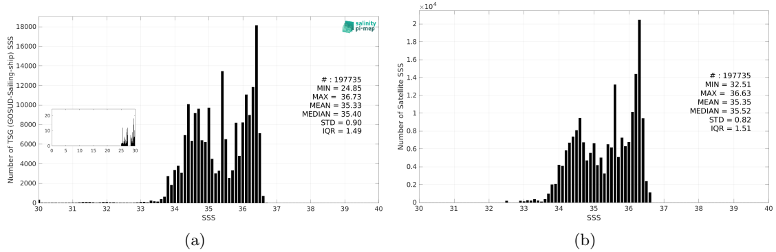
Figure 2: Histograms of SSS from TSG (GOSUD-Sailing-ship) (a) and SMOS SSS L3 v9 - 18 Days (CATDS-CEC-LOCEAN) (b) considering all match-up pairs per bins of 0.1 over the South Pacific Ocean Pi-MEP region and for the full satellite product period.
