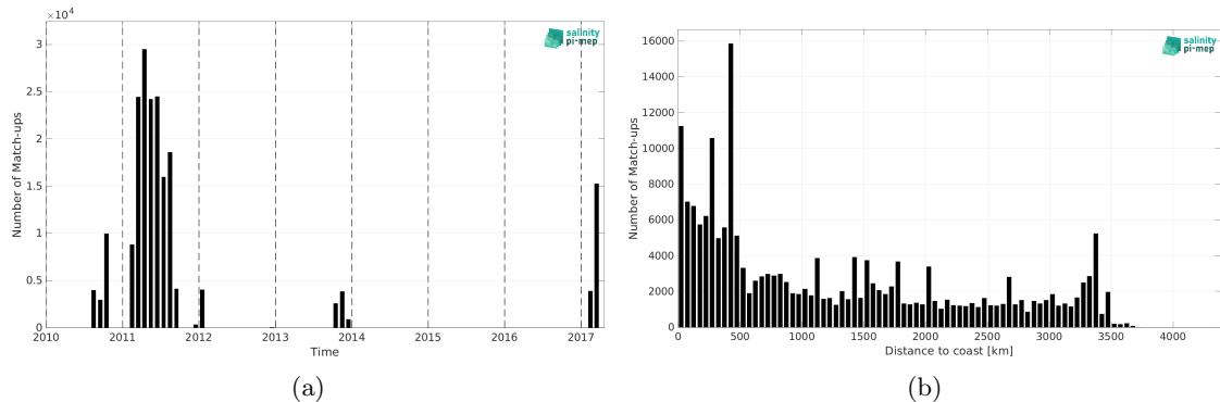
Figure 1: Number of match-ups between TSG (GOSUD-Sailing-ship) and SMOS SSS L3 v9 - 18 Days (CATDS-CEC-LOCEAN) SSS as a function of time (a) and as function of the distance to coast (b) over the South Pacific Ocean Pi-MEP region and for the full satellite product period.
