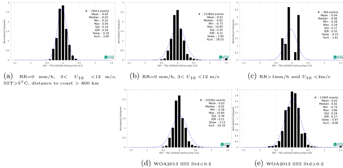
Figure 13: Normalized histogram of \Delta\text{SSS} (SMOS SSS L3 v9 - 18 Days (CATDS-CEC-LOCEAN) - TSG (GOSUD-Sailing-ship)) for 5 different subdatasets corresponding to: RR=0 mm/h, 3 < U_{10} < 12 m/s, SST>5°C, distance to coast > 800 km (a), RR=0 mm/h, 3 < U_{10} < 12 m/s (b), RR>1mm/h and U_{10} < 4 m/s (c), WOA2013 SSS Std<0.2 (d), WOA2013 SSS Std>0.2 (e).
