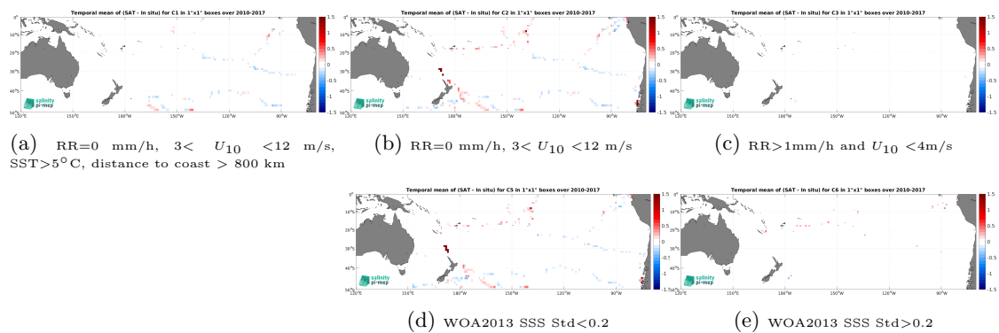
Figure 12: Temporal mean gridded over spatial boxes of size 1^\circ \times 1^\circ of \Delta\text{SSS} (SMOS SSS L3 v9 - 18 Days (CATDS-CEC-LOCEAN) - TSG (GOSUD-Sailing-ship)) for 5 different subdatasets corresponding to:RR=0 mm/h, 3 < U_{10} < 12 m/s, SST >5^\circ\text{C} , distance to coast > 800 km (a), RR=0 mm/h, 3 < U_{10} < 12 m/s (b), RR >1 mm/h and U_{10} < 4 m/s (c), WOA2013 SSS Std <0.2 (d), WOA2013 SSS Std >0.2 (e).
