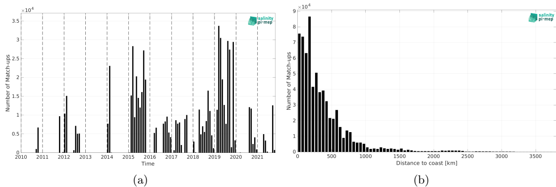
Figure 1: Number of match-ups between TSG (GOSUD-Research-vessel) and SMOS SSS L3 v9 - 18 Days (CATDS-CEC-LOCEAN) SSS as a function of time (a) and as function of the distance to coast (b) over the South Pacific Ocean Pi-MEP region and for the full satellite product period.
