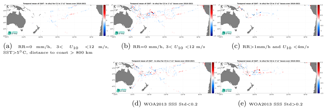
Figure 12: Temporal mean gridded over spatial boxes of size 1^\circ \times 1^\circ of \Delta SSS (SMOS SSS L3 v9 - 18 Days (CATDS-CEC-LOCEAN) - TSG (GOSUD-Research-vessel)) for 5 different subdatasets corresponding to:RR=0 mm/h, 3 < U_{10} < 12 m/s, SST >5^\circ\text{C} , distance to coast > 800 km (a), RR=0 mm/h, 3 < U_{10} < 12 m/s (b), RR >1 mm/h and U_{10} < 4 m/s (c), WOA2013 SSS Std <0.2 (d), WOA2013 SSS Std >0.2 (e).
