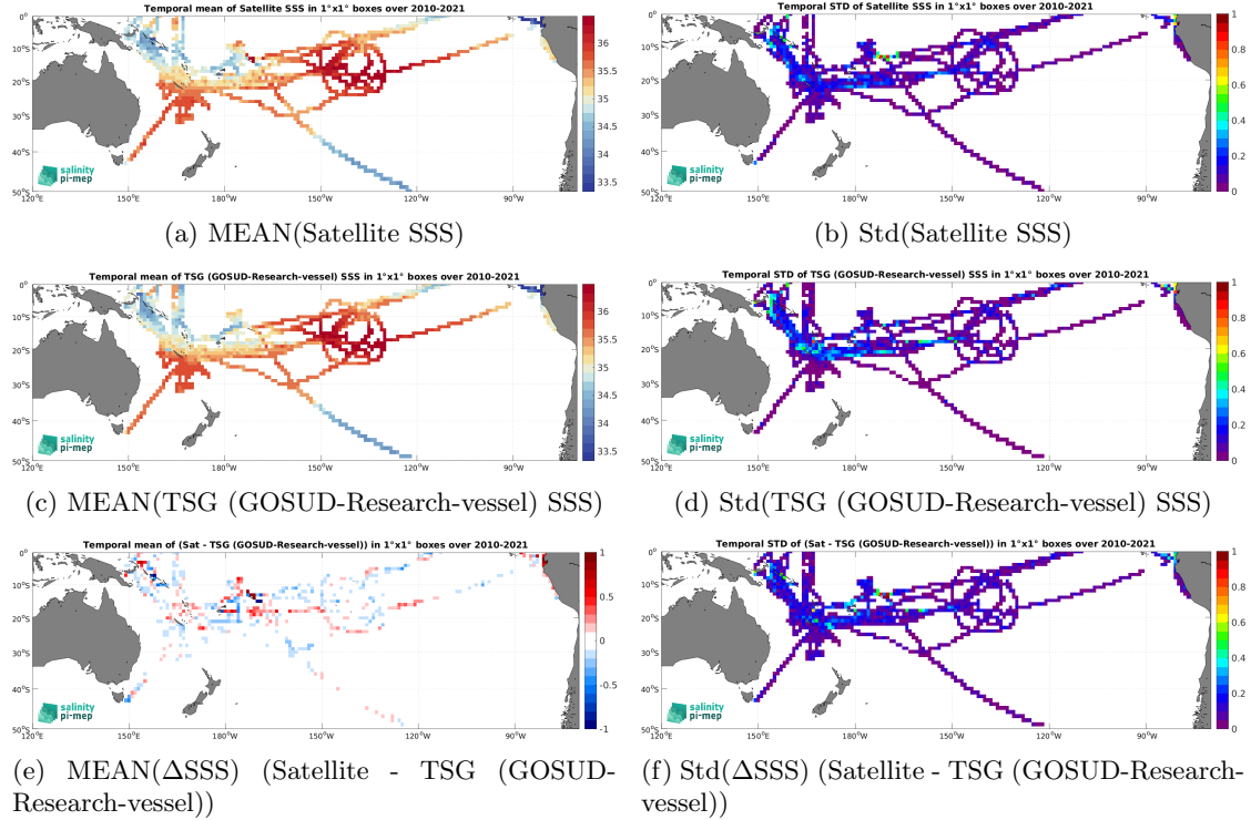
Figure 6: Temporal mean (left) and Std (right) of SSS from SMOS SSS L3 v9 - 18 Days (CATDS-CEC-LOCEAN) (top), TSG (GOSUD-Research-vessel) (middle), and of \Delta SSS (Satellite - TSG (GOSUD-Research-vessel)). Only match-up pairs are used to generate these maps.
