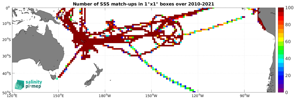
Figure 4: Number of SSS match-ups between TSG (GOSUD-Research-vessel) SSS and the SMOS SSS L3 v9 - 18 Days (CATDS-CEC-LOCEAN) SSS product for the South Pacific Ocean Pi-MEP region over 1^\circ \times 1^\circ boxes and for the full satellite product period.
