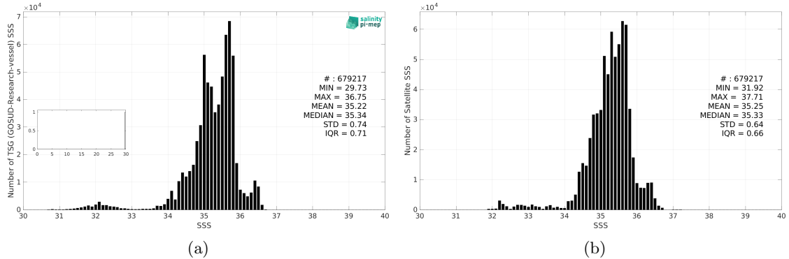
Figure 2: Histograms of SSS from TSG (GOSUD-Research-vessel) (a) and SMOS SSS L3 v9 - 18 Days (CATDS-CEC-LOCEAN) (b) considering all match-up pairs per bins of 0.1 over the South Pacific Ocean Pi-MEP region and for the full satellite product period.
