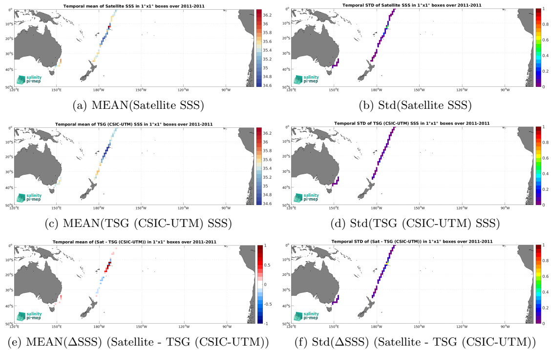
Figure 7: Temporal mean (left) and Std (right) of SSS from SMOS SSS L3 v9 - 18 Days (CATDS-CEC-LOCEAN) (top), TSG (CSIC-UTM) (middle), and of \Delta SSS (Satellite - TSG (CSIC-UTM)). Only match-up pairs are used to generate these maps.
