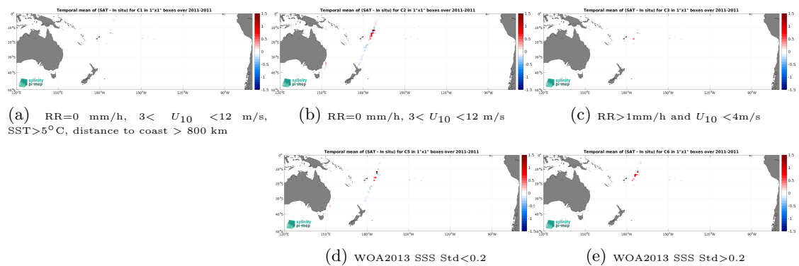
Figure 14: Temporal mean gridded over spatial boxes of size 1^\circ \times 1^\circ of \Delta SSS (SMOS SSS L3 v9 - 18 Days (CATDS-CEC-LOCEAN) - TSG (CSIC-UTM)) for 5 different subdatasets corresponding to:RR=0 mm/h, 3 < U_{10} < 12 m/s, SST>5°C, distance to coast > 800 km (a), RR=0 mm/h, 3 < U_{10} < 12 m/s (b), RR>1mm/h and U_{10} < 4 m/s (c), WOA2013 SSS Std<0.2 (d), WOA2013 SSS Std>0.2 (e).
