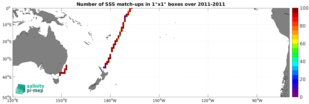
Figure 5: Number of SSS match-ups between TSG (CSIC-UTM) SSS and the SMOS SSS L3 v9 - 18 Days (CATDS-CEC-LOCEAN) SSS product for the South Pacific Ocean Pi-MEP region over 1^\circ \times 1^\circ boxes and for the full satellite product period.
