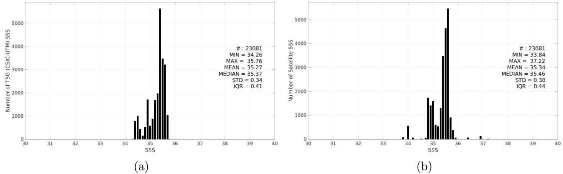
Figure 3: Histograms of SSS from TSG (CSIC-UTM) (a) and SMOS SSS L3 v9 - 18 Days (CATDS-CEC-LOCEAN) (b) considering all match-up pairs per bins of 0.1 over the South Pacific Ocean Pi-MEP region and for the full satellite product period.
