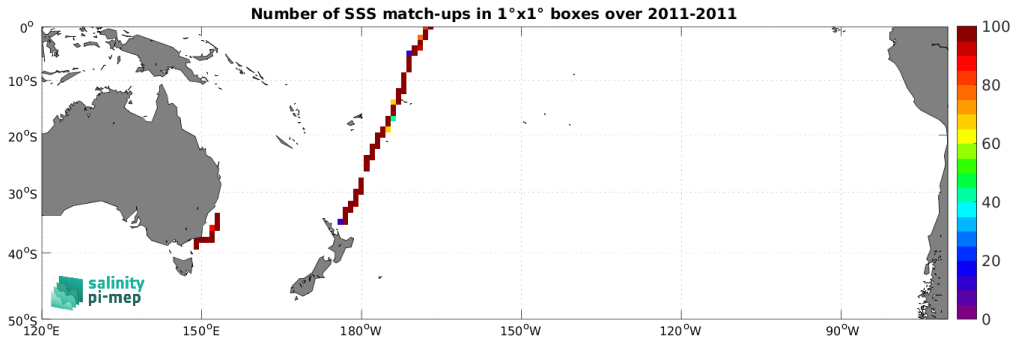
Figure 4: Number of SSS match-ups between TSG (CSIC-UTM) SSS and the SMOS SSS L3 v9 - 18 Days (CATDS-CEC-LOCEAN) SSS product for the South Pacific Ocean Pi-MEP region over 1^\circ \times 1^\circ boxes and for the full satellite product period.
