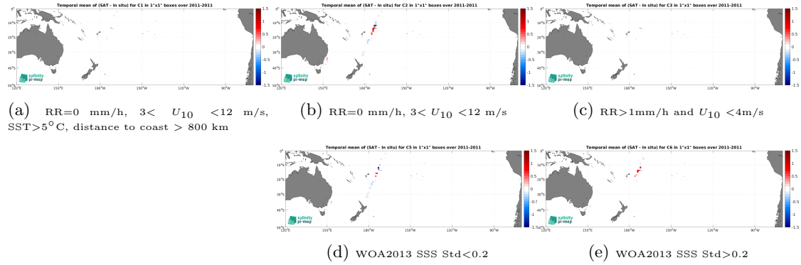
Figure 12: Temporal mean gridded over spatial boxes of size 1^{\circ}\times 1^{\circ} of \Delta\text{SSS} (SMOS SSS L3 v9 - 18 Days (CATDS-CEC-LOCEAN) - TSG (CSIC-UTM)) for 5 different subdatasets corresponding to:RR=0 mm/h, 3 < U_{10} < 12 m/s, SST > 5^{\circ}\text{C} , distance to coast > 800 km (a), RR=0 mm/h, 3 < U_{10} < 12 m/s (b), RR > 1 mm/h and U_{10} < 4 m/s (c), WOA2013 SSS Std < 0.2 (d), WOA2013 SSS Std > 0.2 (e).
