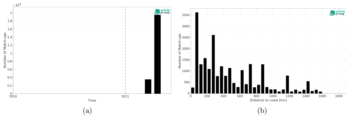
Figure 1: Number of match-ups between TSG (CSIC-UTM) and SMOS SSS L3 v9 - 18 Days (CATDS-CEC-LOCEAN) SSS as a function of time (a) and as function of the distance to coast (b) over the South Pacific Ocean Pi-MEP region and for the full satellite product period.
