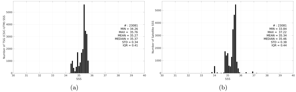
Figure 2: Histograms of SSS from TSG (CSIC-UTM) (a) and SMOS SSS L3 v9 - 18 Days (CATDS-CEC-LOCEAN) (b) considering all match-up pairs per bins of 0.1 over the South Pacific Ocean Pi-MEP region and for the full satellite product period.
