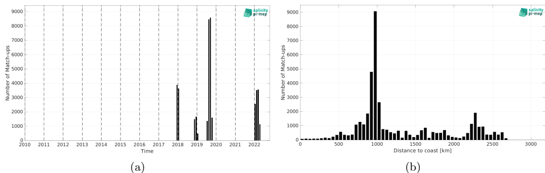
Figure 2: Number of match-ups between Saildrone and SMOS SSS L3 v9 - 18 Days (CATDS-CEC-LOCEAN) SSS as a function of time (a) and as function of the distance to coast (b) over the South Pacific Ocean Pi-MEP region and for the full satellite product period.
