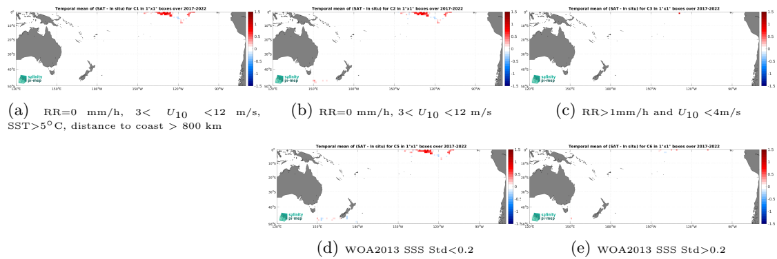
Figure 14: Temporal mean gridded over spatial boxes of size 1^\circ \times 1^\circ of \Delta\text{SSS} (SMOS SSS L3 v9 - 18 Days (CATDS-CEC-LOCEAN) - Sairdrone) for 5 different subdatasets corresponding to:RR=0 mm/h, 3 < U_{10} < 12 m/s, SST>5°C, distance to coast > 800 km (a), RR=0 mm/h, 3 < U_{10} < 12 m/s (b), RR>1mm/h and U_{10} < 4 m/s (c), WOA2013 SSS Std<0.2 (d), WOA2013 SSS Std>0.2 (e).
