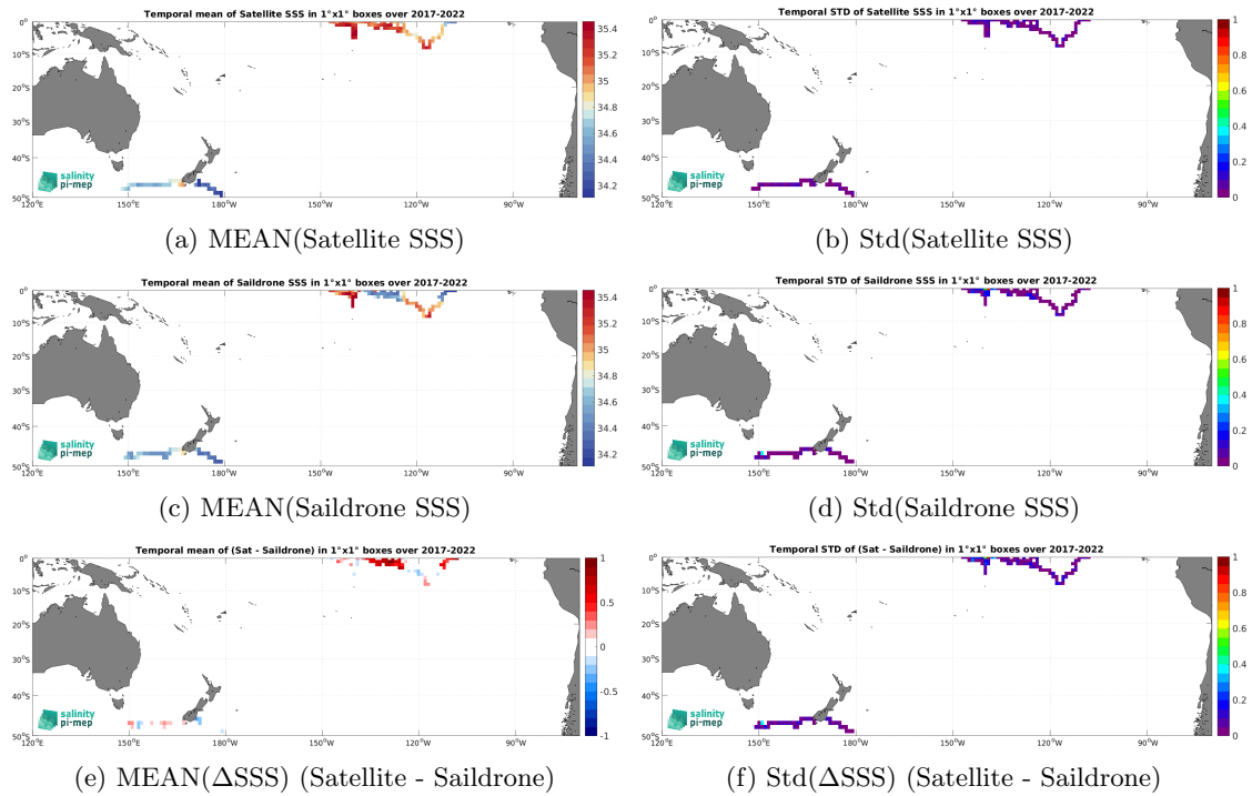
Figure 7: Temporal mean (left) and Std (right) of SSS from SMOS SSS L3 v9 - 18 Days (CATDS-CEC-LOCEAN) (top), Saildrone (middle), and of \Delta SSS (Satellite - Saildrone). Only match-up pairs are used to generate these maps.
