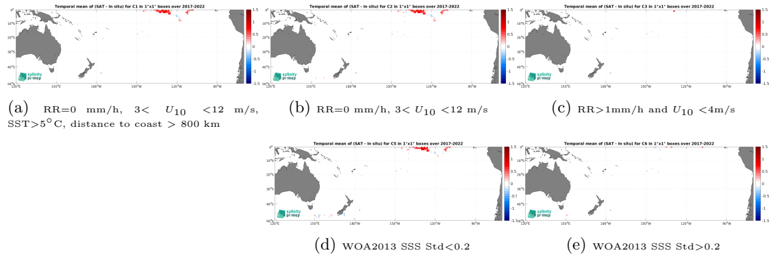
Figure 12: Temporal mean gridded over spatial boxes of size 1^\circ \times 1^\circ of \Delta SSS (SMOS SSS L3 v9 - 18 Days (CATDS-CEC-LOCEAN) - Sairdrone) for 5 different subdatasets corresponding to:RR=0 mm/h, 3 < U_{10} < 12 m/s, SST >5^\circ\text{C} , distance to coast > 800 km (a), RR=0 mm/h, 3 < U_{10} < 12 m/s (b), RR >1 mm/h and U_{10} < 4 m/s (c), WOA2013 SSS Std <0.2 (d), WOA2013 SSS Std >0.2 (e).
