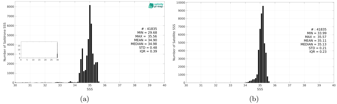
Figure 2: Histograms of SSS from Saildrone (a) and SMOS SSS L3 v9 - 18 Days (CATDS-CEC-LOCEAN) (b) considering all match-up pairs per bins of 0.1 over the South Pacific Ocean Pi-MEP region and for the full satellite product period.
