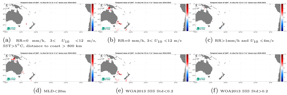
Figure 14: Temporal mean gridded over spatial boxes of size 1^\circ \times 1^\circ of \Delta SSS (SMOS SSS L3 v9 - 18 Days (CATDS-CEC-LOCEAN) - Marine mammals) for 6 different subdatasets corresponding to:RR=0 mm/h, 3 < U_{10} < 12 m/s, SST >5^\circ C, distance to coast > 800 km (a), RR=0 mm/h, 3 < U_{10} < 12 m/s (b), RR >1 mm/h and U_{10} < 4 m/s (c),MLD <20 m (d),WOA2013 SSS Std <0.2 (e),WOA2013 SSS Std >0.2 (f).
