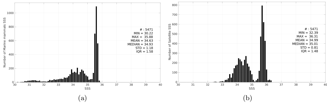
Figure 3: Histograms of SSS from Marine mammals (a) and SMOS SSS L3 v9 - 18 Days (CATDS-CEC-LOCEAN) (b) considering all match-up pairs per bins of 0.1 over the South Pacific Ocean Pi-MEP region and for the full satellite product period.
