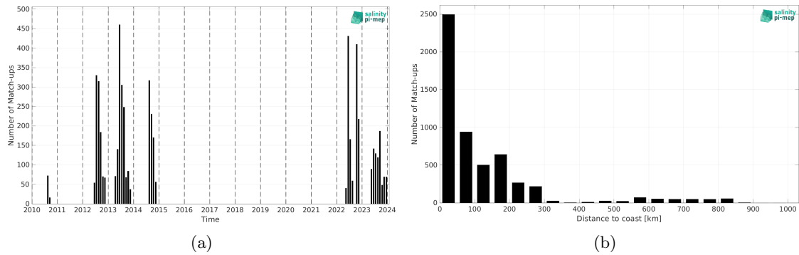
Figure 2: Number of match-ups between Marine mammals and SMOS SSS L3 v9 - 18 Days (CATDS-CEC-LOCEAN) SSS as a function of time (a) and as function of the distance to coast (b) over the South Pacific Ocean Pi-MEP region and for the full satellite product period.
