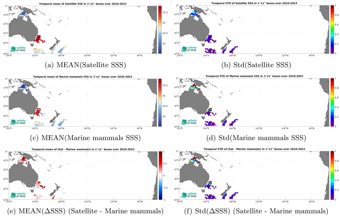
Figure 7: Temporal mean (left) and Std (right) of SSS from SMOS SSS L3 v9 - 18 Days (CATDS-CEC-LOCEAN) (top), Marine mammals (middle), and of \Delta SSS (Satellite - Marine mammals). Only match-up pairs are used to generate these maps.
