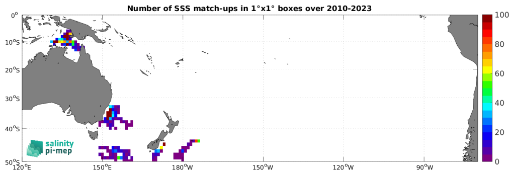
Figure 5: Number of SSS match-ups between Marine mammals SSS and the SMOS SSS L3 v9 - 18 Days (CATDS-CEC-LOCEAN) SSS product for the South Pacific Ocean Pi-MEP region over 1^\circ \times 1^\circ boxes and for the full satellite product period.
