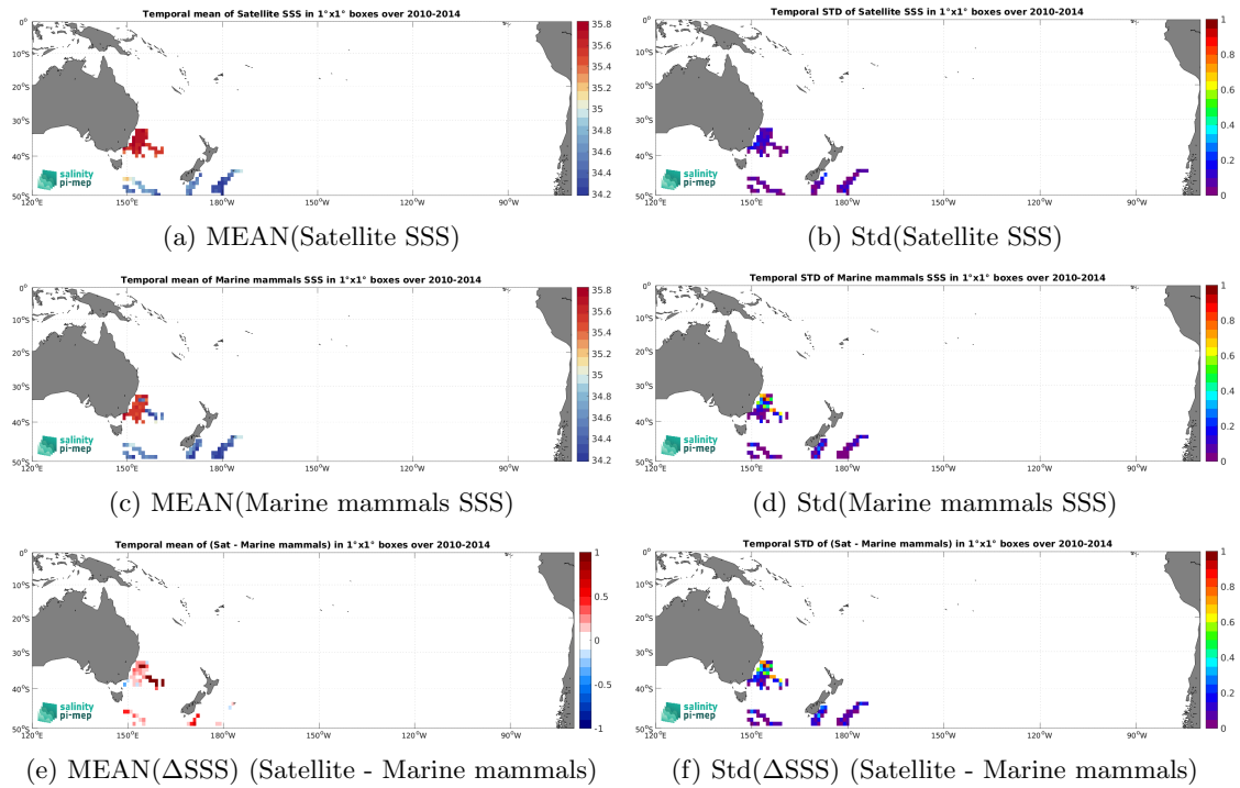
Figure 6: Temporal mean (left) and Std (right) of SSS from SMOS SSS L3 v9 - 18 Days (CATDS-CEC-LOCEAN) (top), Marine mammals (middle), and of \Delta SSS (Satellite - Marine mammals). Only match-up pairs are used to generate these maps.
