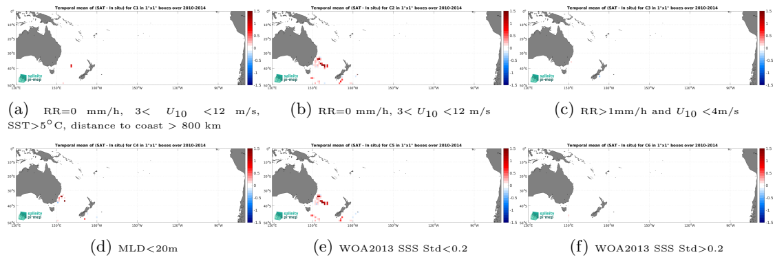
Figure 12: Temporal mean gridded over spatial boxes of size 1^{\circ}\times 1^{\circ} of \Delta\text{SSS} (SMOS SSS L3 v9 - 18 Days (CATDS-CEC-LOCEAN) - Marine mammals) for 6 different subdatasets corresponding to: RR=0 mm/h, 3 < U_{10} < 12 m/s, SST > 5^{\circ}\text{C} , distance to coast > 800 km (a), RR=0 mm/h, 3 < U_{10} < 12 m/s (b), RR > 1 mm/h and U_{10} < 4 m/s (c), MLD < 20\text{m} (d), WOA2013 SSS Std < 0.2 (e), WOA2013 SSS Std > 0.2 (f).
