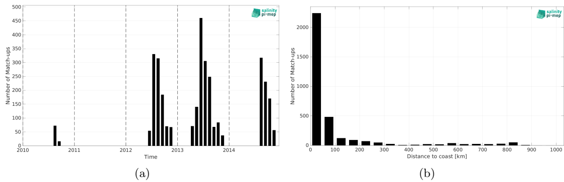
Figure 1: Number of match-ups between Marine mammals and SMOS SSS L3 v9 - 18 Days (CATDS-CEC-LOCEAN) SSS as a function of time (a) and as function of the distance to coast (b) over the South Pacific Ocean Pi-MEP region and for the full satellite product period.
