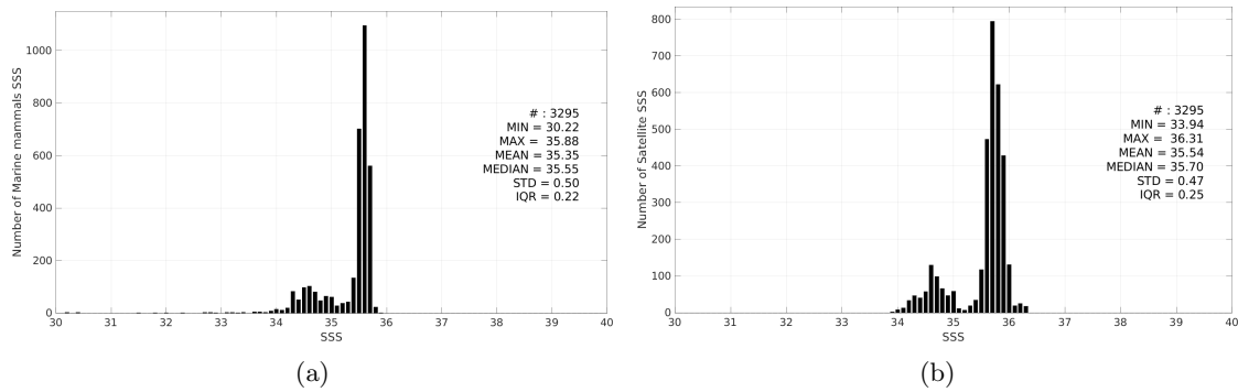
Figure 2: Histograms of SSS from Marine mammals (a) and SMOS SSS L3 v9 - 18 Days (CATDS-CEC-LOCEAN) (b) considering all match-up pairs per bins of 0.1 over the South Pacific Ocean Pi-MEP region and for the full satellite product period.
