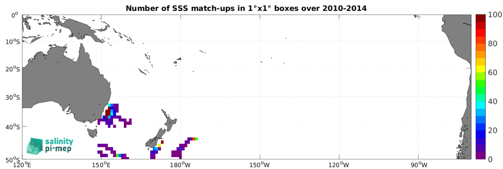
Figure 4: Number of SSS match-ups between Marine mammals SSS and the SMOS SSS L3 v9 - 18 Days (CATDS-CEC-LOCEAN) SSS product for the South Pacific Ocean Pi-MEP region over 1^\circ \times 1^\circ boxes and for the full satellite product period.
