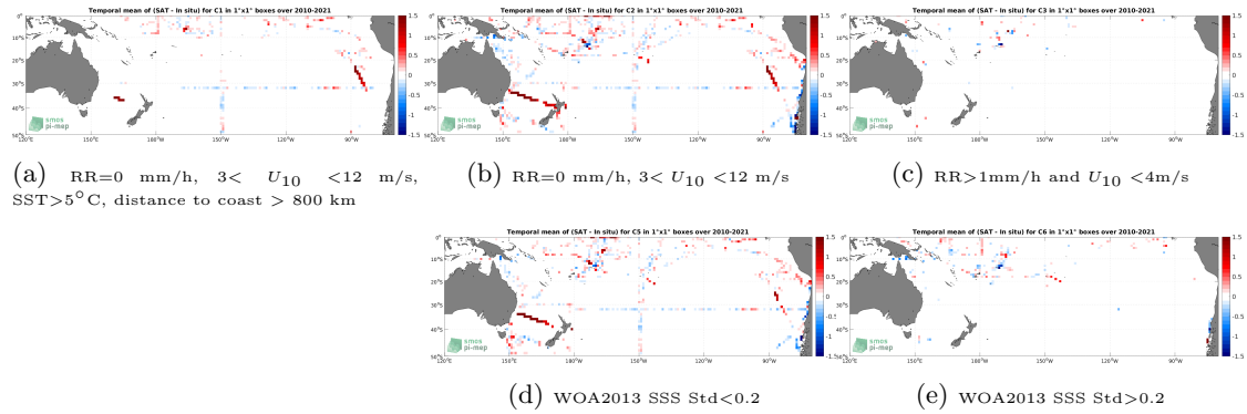
Figure 12: Temporal mean gridded over spatial boxes of size 1^\circ \times 1^\circ of \Delta SSS (SMOS SSS L3 v8 - 9 Days (CATDS-CECOS-LOCEAN) - TSG (SAMOS)) for 5 different subdatasets corresponding to:RR=0 mm/h, 3 < U_{10} < 12 m/s, SST >5^\circ C, distance to coast > 800 km (a), RR=0 mm/h, 3 < U_{10} < 12 m/s (b), RR >1 mm/h and U_{10} < 4 m/s (c), WOA2013 SSS Std <0.2 (d), WOA2013 SSS Std >0.2 (e).
