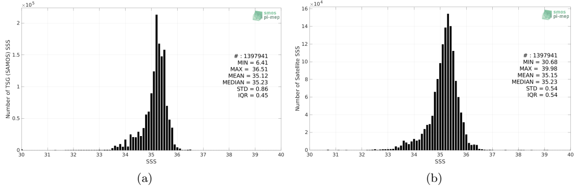
Figure 2: Histograms of SSS from TSG (SAMOS) (a) and SMOS SSS L3 v8 - 9 Days (CATDS-CECOS-LOCEAN) (b) considering all match-up pairs per bins of 0.1 over the South Pacific Ocean Pi-MEP region and for the full satellite product period.
