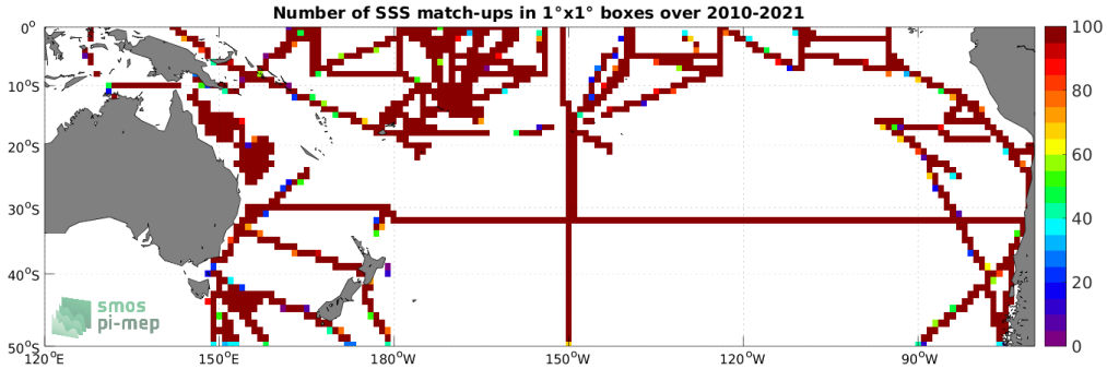
Figure 4: Number of SSS match-ups between TSG (SAMOS) SSS and the SMOS SSS L3 v8 - 9 Days (CATDS-CECOS-LOCEAN) SSS product for the South Pacific Ocean Pi-MEP region over 1^\circ \times 1^\circ boxes and for the full satellite product period.
