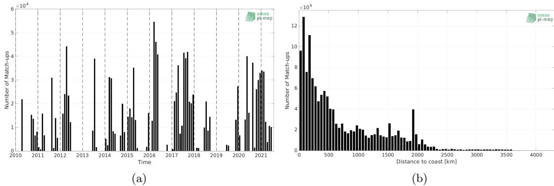
Figure 1: Number of match-ups between TSG (SAMOS) and SMOS SSS L3 v8 - 9 Days (CATDS-CECOS-LOCEAN) SSS as a function of time (a) and as function of the distance to coast (b) over the South Pacific Ocean Pi-MEP region and for the full satellite product period.
