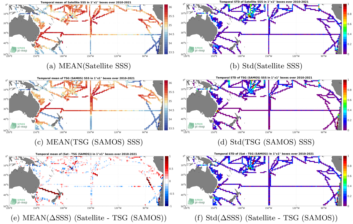
Figure 6: Temporal mean (left) and Std (right) of SSS from SMOS SSS L3 v8 - 9 Days (CATDS-CECOS-LOCEAN) (top), TSG (SAMOS) (middle), and of \Delta SSS (Satellite - TSG (SAMOS)). Only match-up pairs are used to generate these maps.
