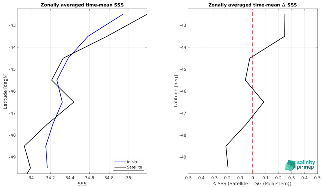
Figure 8: Left panel: Zonal mean SSS from SMOS SSS L3 v8 - 9 Days (CATDS-CEC-LOCEAN) satellite product (black) and from TSG (Polarstern) (blue). Right panel: Zonal mean of \Delta SSS (Satellite - TSG (Polarstern)) for all the collected Pi-MEP match-up pairs estimated over the full satellite product period.
