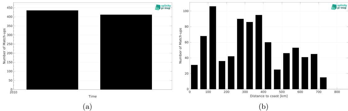
Figure 1: Number of match-ups between TSG (Polarstern) and SMOS SSS L3 v8 - 9 Days (CATDS-CEC-LOCEAN) SSS as a function of time (a) and as function of the distance to coast (b) over the South Pacific Ocean Pi-MEP region and for the full satellite product period.
