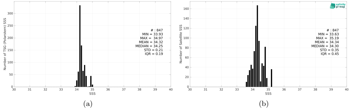
Figure 2: Histograms of SSS from TSG (Polarstern) (a) and SMOS SSS L3 v8 - 9 Days (CATDS-CEC-LOCEAN) (b) considering all match-up pairs per bins of 0.1 over the South Pacific Ocean Pi-MEP region and for the full satellite product period.
