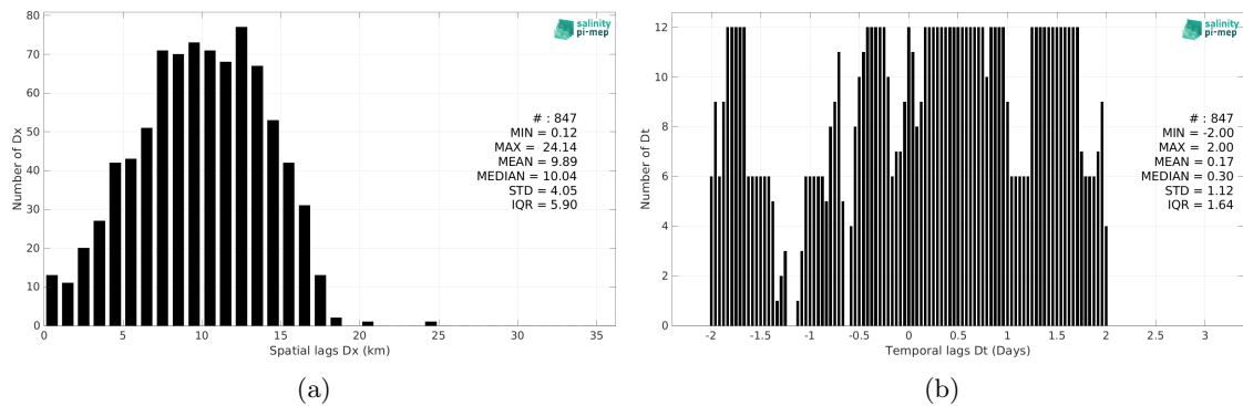
Figure 5: Histograms of the spatial (a) and temporal (b) lags between the location/time of the TSG (Polarstern) measurement and the date of the corresponding SMOS SSS L3 v8 - 9 Days (CATDS-CEC-LOCEAN) SSS pixel.
