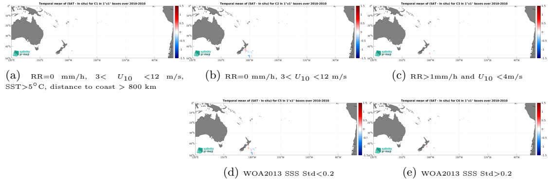
Figure 12: Temporal mean gridded over spatial boxes of size 1^{\circ}\times 1^{\circ} of \Delta\text{SSS} (SMOS SSS L3 v8 - 9 Days (CATDS-CEC-LOCEAN) - TSG (Polarstern)) for 5 different subdatasets corresponding to: RR=0 mm/h, 3 < U_{10} < 12 m/s, SST > 5^{\circ}\text{C} , distance to coast > 800 km (a), RR=0 mm/h, 3 < U_{10} < 12 m/s (b), RR > 1 mm/h and U_{10} < 4 m/s (c), WOA2013 SSS Std < 0.2 (d), WOA2013 SSS Std > 0.2 (e).
