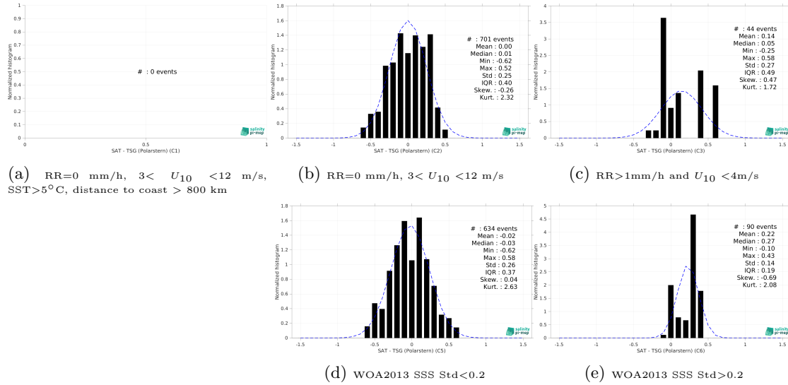
Figure 13: Normalized histogram of \Delta SSS (SMOS SSS L3 v8 - 9 Days (CATDS-CEC-LOCEAN) - TSG (Polarstern)) for 5 different subdatasets corresponding to: RR=0 mm/h, 3 < U_{10} < 12 m/s, SST>5°C, distance to coast > 800 km (a), RR=0 mm/h, 3 < U_{10} < 12 m/s (b), RR>1mm/h and U_{10} < 4 m/s (c), WOA2013 SSS Std<0.2 (d), WOA2013 SSS Std>0.2 (e).
