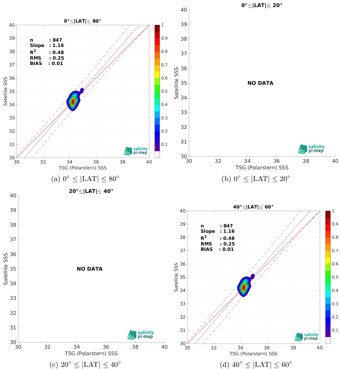
Figure 9: Contour maps of the concentration of SMOS SSS L3 v8 - 9 Days (CATDS-CEC-LOCEAN) SSS (y-axis) versus TSG (Polarstern) SSS (x-axis) at match-up pairs for different latitude bands. For each plot, the red line shows x=y . The black thin and dashed lines indicate a linear fit through the data cloud and the \pm 95\% confidence levels, respectively. The number match-up pairs n , the slope and R^2 coefficient of the linear fit, the root mean square (RMS) and the mean bias between satellite and in situ data are indicated for each latitude band in each plots.
