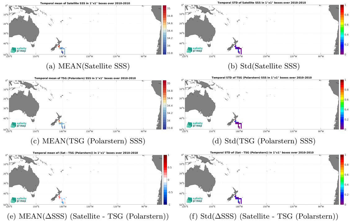
Figure 6: Temporal mean (left) and Std (right) of SSS from SMOS SSS L3 v8 - 9 Days (CATDS-CEC-LOCEAN) (top), TSG (Polarstern) (middle), and of \Delta SSS (Satellite - TSG (Polarstern)). Only match-up pairs are used to generate these maps.
