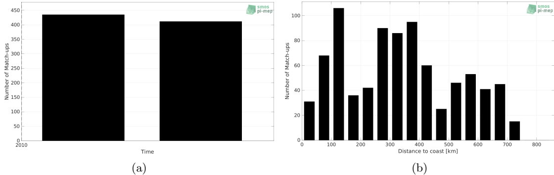
Figure 1: Number of match-ups between TSG (Polarstern) and SMOS SSS L3 v8 - 9 Days (CATDS-CECOS-LOCEAN) SSS as a function of time (a) and as function of the distance to coast (b) over the South Pacific Ocean Pi-MEP region and for the full satellite product period.
