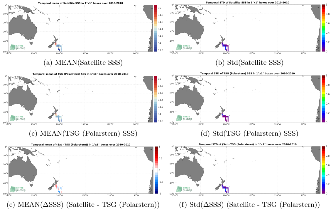
Figure 6: Temporal mean (left) and Std (right) of SSS from SMOS SSS L3 v8 - 9 Days (CATDS-CECOS-LOCEAN) (top), TSG (Polarstern) (middle), and of \Delta SSS (Satellite - TSG (Polarstern)). Only match-up pairs are used to generate these maps.
