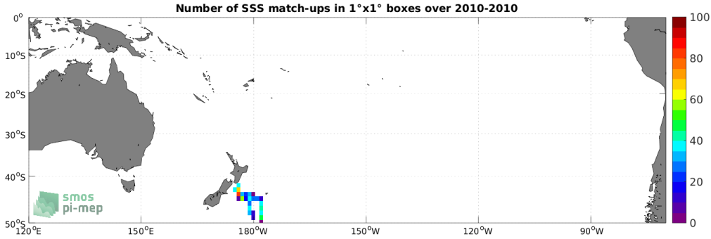
Figure 4: Number of SSS match-ups between TSG (Polarstern) SSS and the SMOS SSS L3 v8 - 9 Days (CATDS-CECOS-LOCEAN) SSS product for the South Pacific Ocean Pi-MEP region over 1^\circ \times 1^\circ boxes and for the full satellite product period.
