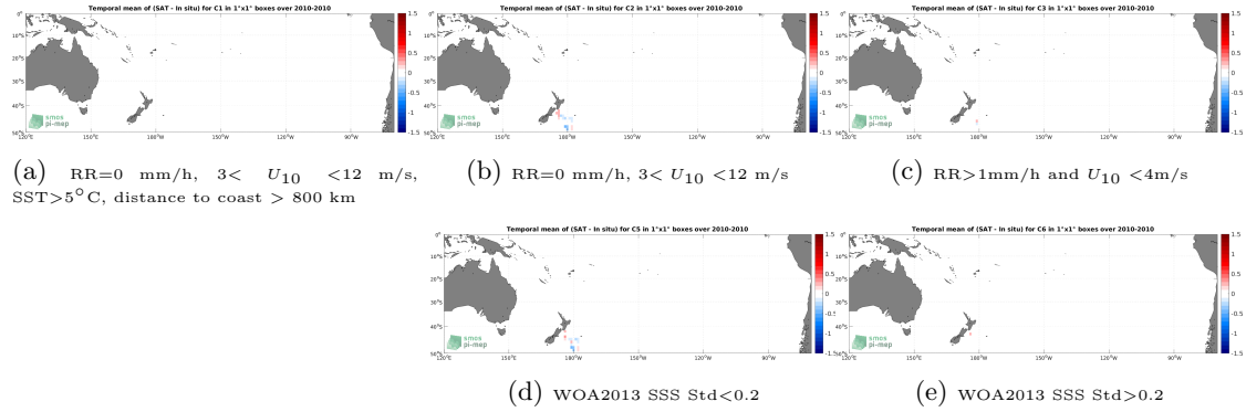
Figure 12: Temporal mean gridded over spatial boxes of size 1^{\circ}\times 1^{\circ} of \Delta\text{SSS} (SMOS SSS L3 v8 - 9 Days (CATDS-CECOS-LOCEAN) - TSG (Polarstern)) for 5 different subdatasets corresponding to:RR=0 mm/h, 3 < U_{10} < 12 m/s, SST >5^{\circ}\text{C} , distance to coast > 800 km (a), RR=0 mm/h, 3 < U_{10} < 12 m/s (b), RR >1 mm/h and U_{10} < 4 m/s (c), WOA2013 SSS Std <0.2 (d), WOA2013 SSS Std >0.2 (e).
