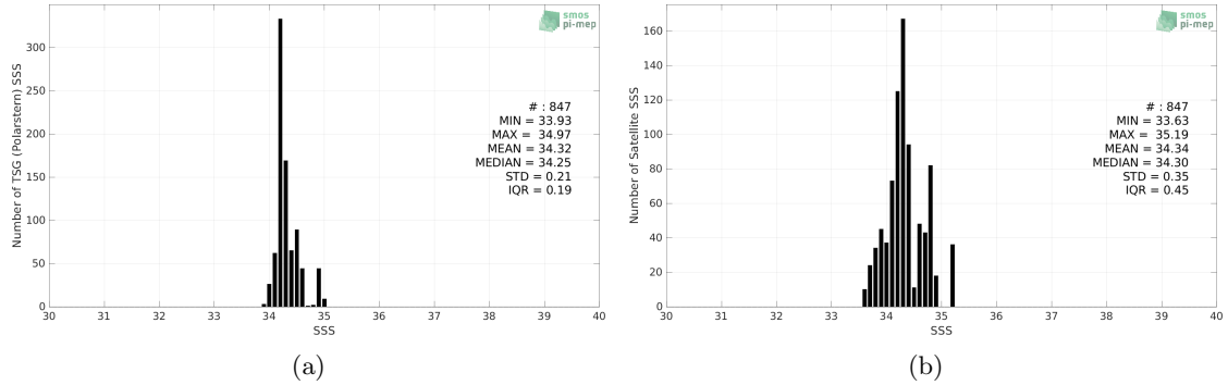
Figure 2: Histograms of SSS from TSG (Polarstern) (a) and SMOS SSS L3 v8 - 9 Days (CATDS-CECOS-LOCEAN) (b) considering all match-up pairs per bins of 0.1 over the South Pacific Ocean Pi-MEP region and for the full satellite product period.
