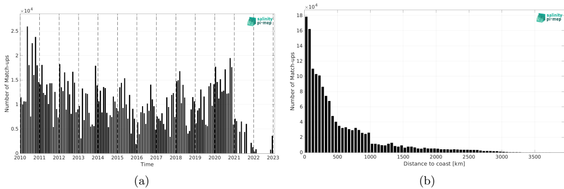
Figure 1: Number of match-ups between TSG (LEGOS-DM) and SMOS SSS L3 v8 - 9 Days (CATDS-CEC-LOCEAN) SSS as a function of time (a) and as function of the distance to coast (b) over the South Pacific Ocean Pi-MEP region and for the full satellite product period.
