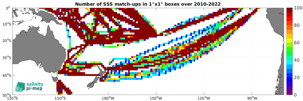
Figure 4: Number of SSS match-ups between TSG (LEGOS-DM) SSS and the SMOS SSS L3 v8 - 9 Days (CATDS-CEC-LOCEAN) SSS product for the South Pacific Ocean Pi-MEP region over 1^\circ \times 1^\circ boxes and for the full satellite product period.
