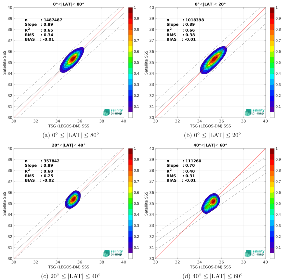
Figure 9: Contour maps of the concentration of SMOS SSS L3 v8 - 9 Days (CATDS-CEC-LOCEAN) SSS ( y -axis) versus TSG (LEGOS-DM) SSS ( x -axis) at match-up pairs for different latitude bands. For each plot, the red line shows x=y . The black thin and dashed lines indicate a linear fit through the data cloud and the \pm 95\% confidence levels, respectively. The number match-up pairs n , the slope and R^2 coefficient of the linear fit, the root mean square (RMS) and the mean bias between satellite and in situ data are indicated for each latitude band in each plots.
