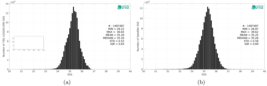
Figure 2: Histograms of SSS from TSG (LEGOS-DM) (a) and SMOS SSS L3 v8 - 9 Days (CATDS-CEC-LOCEAN) (b) considering all match-up pairs per bins of 0.1 over the South Pacific Ocean Pi-MEP region and for the full satellite product period.
