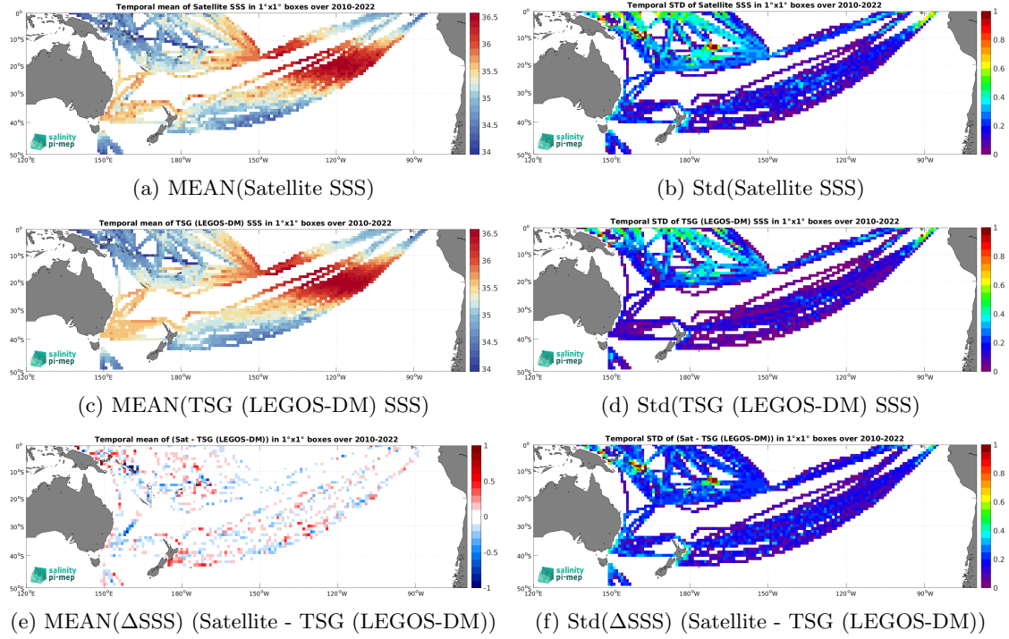
Figure 6: Temporal mean (left) and Std (right) of SSS from SMOS SSS L3 v8 - 9 Days (CATDS-CEC-LOCEAN) (top), TSG (LEGOS-DM) (middle), and of \Delta SSS (Satellite - TSG (LEGOS-DM)). Only match-up pairs are used to generate these maps.
