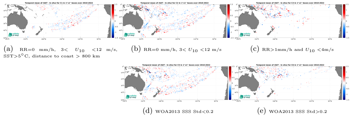
Figure 12: Temporal mean gridded over spatial boxes of size 1^\circ \times 1^\circ of \Delta\text{SSS} (SMOS SSS L3 v8 - 9 Days (CATDS-CEC-LOCEAN) - TSG (LEGOS-DM)) for 5 different subdatasets corresponding to:RR=0 mm/h, 3 < U_{10} < 12 m/s, SST >5^\circ\text{C} , distance to coast > 800 km (a), RR=0 mm/h, 3 < U_{10} < 12 m/s (b), RR >1 mm/h and U_{10} < 4 m/s (c), WOA2013 SSS Std <0.2 (d), WOA2013 SSS Std >0.2 (e).
