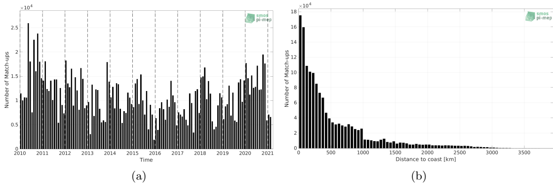
Figure 1: Number of match-ups between TSG (LEGOS-DM) and SMOS SSS L3 v8 - 9 Days (CATDS-CECOS-LOCEAN) SSS as a function of time (a) and as function of the distance to coast (b) over the South Pacific Ocean Pi-MEP region and for the full satellite product period.
