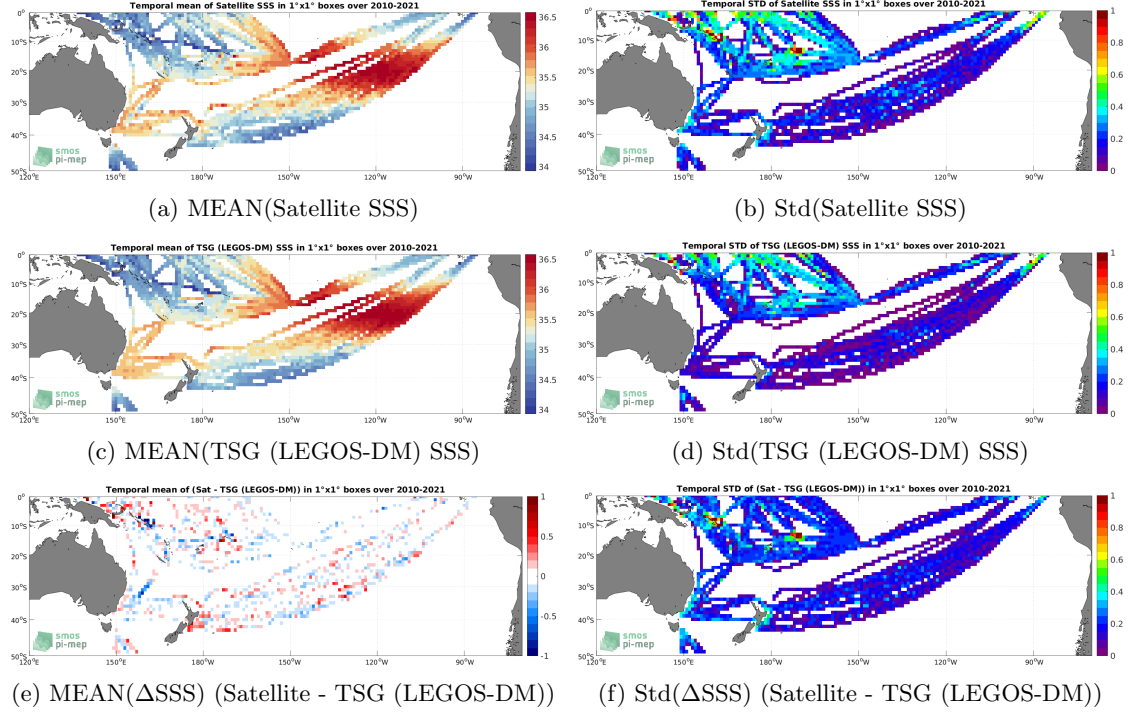
Figure 6: Temporal mean (left) and Std (right) of SSS from SMOS SSS L3 v8 - 9 Days (CATDS-CECOS-LOCEAN) (top), TSG (LEGOS-DM) ( in situ ) dataset (middle), and of \Delta SSS (Satellite - TSG (LEGOS-DM)). Only match-up pairs are used to generate these maps.
