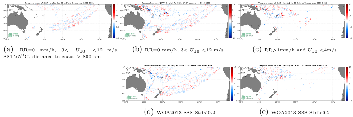
Figure 12: Temporal mean gridded over spatial boxes of size 1^\circ \times 1^\circ of \Delta SSS (SMOS SSS L3 v8 - 9 Days (CATDS-CECOS-LOCEAN) - TSG (LEGOS-DM)) for 5 different subdatasets corresponding to:RR=0 mm/h, 3 < U_{10} < 12 m/s, SST >5^\circ C, distance to coast > 800 km (a), RR=0 mm/h, 3 < U_{10} < 12 m/s (b), RR >1 mm/h and U_{10} < 4 m/s (c), WOA2013 SSS Std <0.2 (d), WOA2013 SSS Std >0.2 (e).
