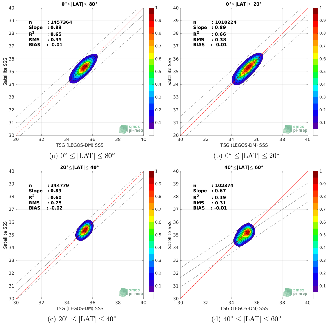
Figure 9: Contour maps of the concentration of SMOS SSS L3 v8 - 9 Days (CATDS-CECOS-LOCEAN) SSS ( y -axis) versus TSG (LEGOS-DM) SSS ( x -axis) at match-up pairs for different latitude bands. For each plot, the red line shows x=y . The black thin and dashed lines indicate a linear fit through the data cloud and the \pm 95\% confidence levels, respectively. The number match-up pairs n , the slope and R^2 coefficient of the linear fit, the root mean square (RMS) and the mean bias between satellite and in situ data are indicated for each latitude band in each plots.
