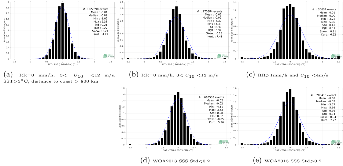
Figure 13: Normalized histogram of \Delta\text{SSS} (SMOS SSS L3 v8 - 9 Days (CATDS-CECOS-LOCEAN) - TSG (LEGOS-DM)) for 5 different subdatasets corresponding to: RR=0 mm/h, 3 < U_{10} < 12 m/s, SST > 5^\circ\text{C} , distance to coast > 800 km (a), RR=0 mm/h, 3 < U_{10} < 12 m/s (b), RR > 1 mm/h and U_{10} < 4 m/s (c), WOA2013 SSS Std < 0.2 (d), WOA2013 SSS Std > 0.2 (e).
