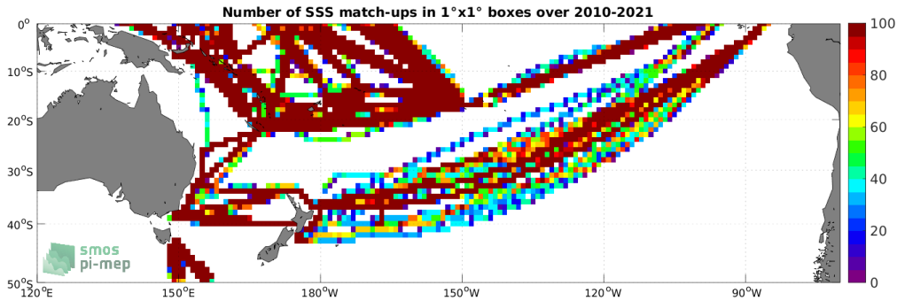
Figure 4: Number of SSS match-ups between TSG (LEGOS-DM) SSS and the SMOS SSS L3 v8 - 9 Days (CATDS-CECOS-LOCEAN) SSS product for the South Pacific Ocean Pi-MEP region over 1^\circ \times 1^\circ boxes and for the full satellite product period.
