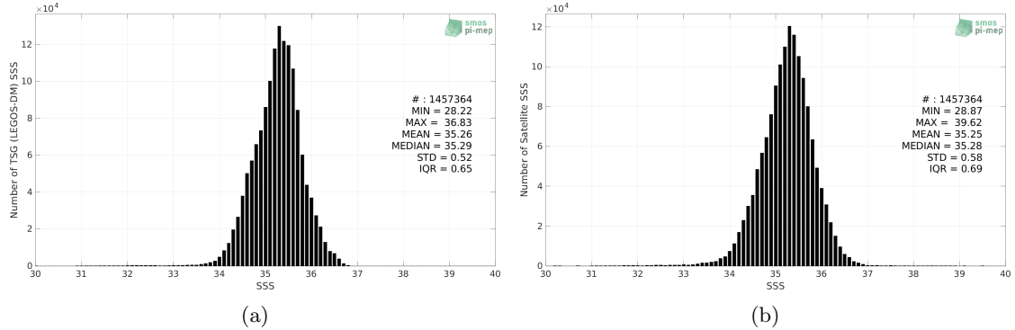
Figure 2: Histograms of SSS from TSG (LEGOS-DM) (a) and SMOS SSS L3 v8 - 9 Days (CATDS-CECOS-LOCEAN) (b) considering all match-up pairs per bins of 0.1 over the South Pacific Ocean Pi-MEP region and for the full satellite product period.
