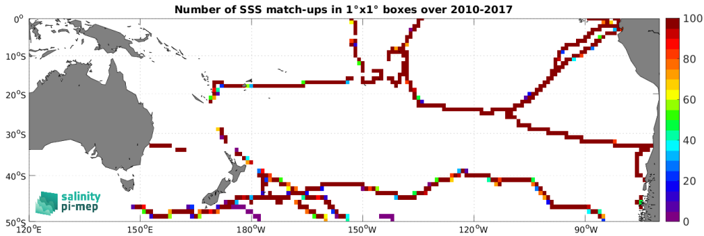
Figure 4: Number of SSS match-ups between TSG (GOSUD-Sailing-ship) SSS and the SMOS SSS L3 v8 - 9 Days (CATDS-CEC-LOCEAN) SSS product for the South Pacific Ocean Pi-MEP region over 1^\circ \times 1^\circ boxes and for the full satellite product period.
