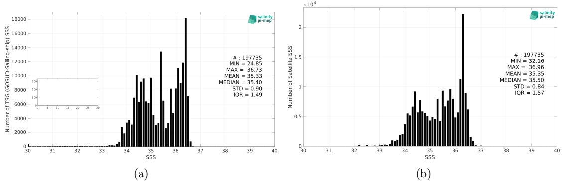
Figure 2: Histograms of SSS from TSG (GOSUD-Sailing-ship) (a) and SMOS SSS L3 v8 - 9 Days (CATDS-CEC-LOCEAN) (b) considering all match-up pairs per bins of 0.1 over the South Pacific Ocean Pi-MEP region and for the full satellite product period.
