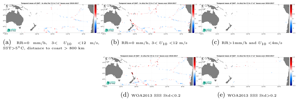
Figure 12: Temporal mean gridded over spatial boxes of size 1^\circ \times 1^\circ of \Delta\text{SSS} (SMOS SSS L3 v8 - 9 Days (CATDS-CEC-LOCEAN) - TSG (GOSUD-Sailing-ship)) for 5 different subdatasets corresponding to:RR=0 mm/h, 3 < U_{10} < 12 m/s, SST>5°C, distance to coast > 800 km (a), RR=0 mm/h, 3 < U_{10} < 12 m/s (b), RR>1mm/h and U_{10} < 4 m/s (c), WOA2013 SSS Std<0.2 (d), WOA2013 SSS Std>0.2 (e).
