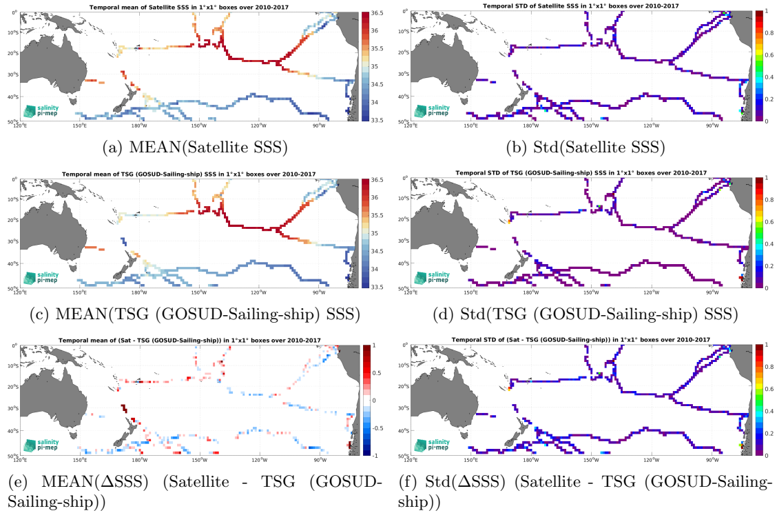
Figure 6: Temporal mean (left) and Std (right) of SSS from SMOS SSS L3 v8 - 9 Days (CATDS-CEC-LOCEAN) (top), TSG (GOSUD-Sailing-ship) (middle), and of \Delta SSS (Satellite - TSG (GOSUD-Sailing-ship)). Only match-up pairs are used to generate these maps.
