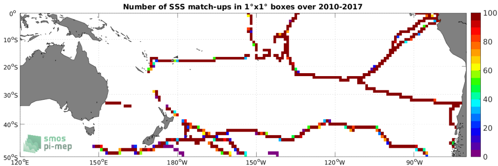
Figure 4: Number of SSS match-ups between TSG (GOSUD-Sailing-ship) SSS and the SMOS SSS L3 v8 - 9 Days (CATDS-CECOS-LOCEAN) SSS product for the South Pacific Ocean Pi-MEP region over 1^\circ \times 1^\circ boxes and for the full satellite product period.
