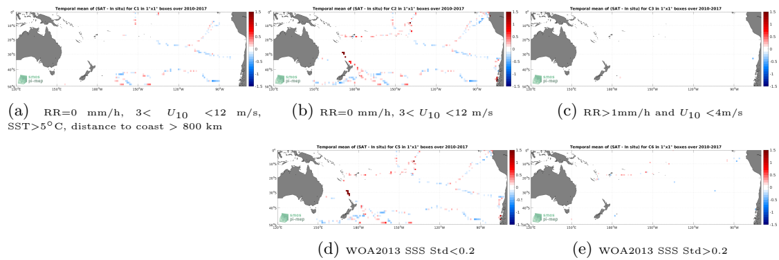
Figure 12: Temporal mean gridded over spatial boxes of size 1^\circ \times 1^\circ of \Delta SSS (SMOS SSS L3 v8 - 9 Days (CATDS-CECOS-LOCEAN) - TSG (GOSUD-Sailing-ship)) for 5 different subdatasets corresponding to:RR=0 mm/h, 3 < U_{10} < 12 m/s, SST >5^\circ\text{C} , distance to coast > 800 km (a), RR=0 mm/h, 3 < U_{10} < 12 m/s (b), RR >1 mm/h and U_{10} < 4 m/s (c), WOA2013 SSS Std <0.2 (d), WOA2013 SSS Std >0.2 (e).
