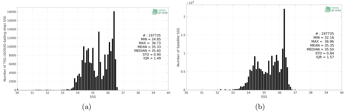
Figure 2: Histograms of SSS from TSG (GOSUD-Sailing-ship) (a) and SMOS SSS L3 v8 - 9 Days (CATDS-CECOS-LOCEAN) (b) considering all match-up pairs per bins of 0.1 over the South Pacific Ocean Pi-MEP region and for the full satellite product period.
