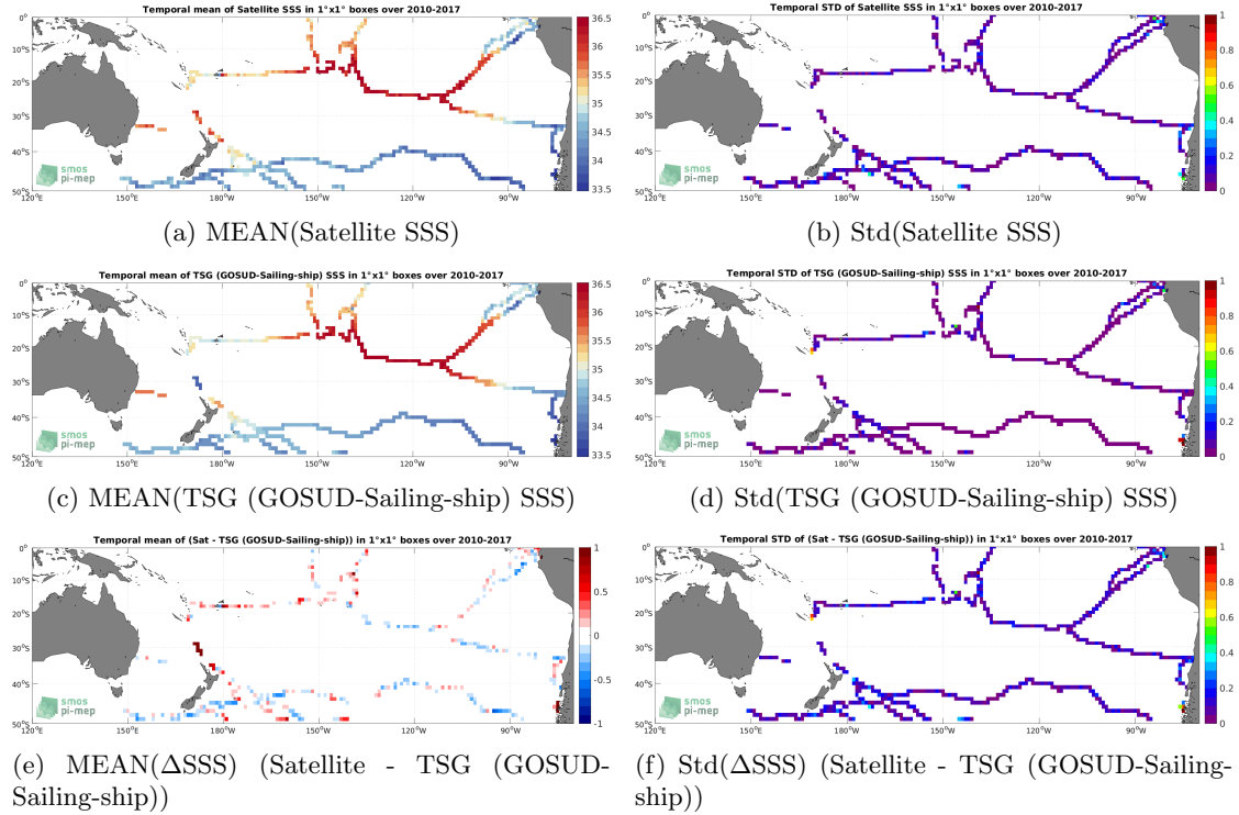
Figure 6: Temporal mean (left) and Std (right) of SSS from SMOS SSS L3 v8 - 9 Days (CATDS-CECOS-LOCEAN) (top), TSG (GOSUD-Sailing-ship) (middle), and of \Delta SSS (Satellite - TSG (GOSUD-Sailing-ship)). Only match-up pairs are used to generate these maps.
