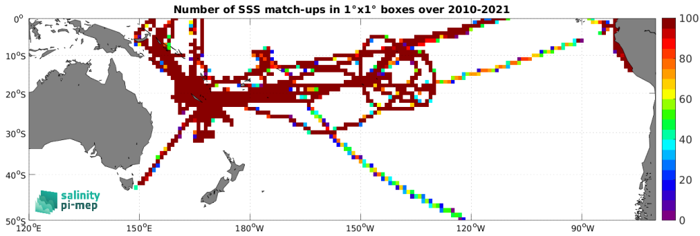
Figure 4: Number of SSS match-ups between TSG (GOSUD-Research-vessel) SSS and the SMOS SSS L3 v8 - 9 Days (CATDS-CEC-LOCEAN) SSS product for the South Pacific Ocean Pi-MEP region over 1^\circ \times 1^\circ boxes and for the full satellite product period.
