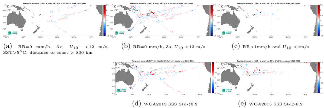
Figure 12: Temporal mean gridded over spatial boxes of size 1^\circ \times 1^\circ of \Delta SSS (SMOS SSS L3 v8 - 9 Days (CATDS-CEC-LOCEAN) - TSG (GOSUD-Research-vessel)) for 5 different subdatasets corresponding to:RR=0 mm/h, 3 < U_{10} < 12 m/s, SST >5^\circ C, distance to coast > 800 km (a), RR=0 mm/h, 3 < U_{10} < 12 m/s (b), RR >1 mm/h and U_{10} < 4 m/s (c), WOA2013 SSS Std <0.2 (d), WOA2013 SSS Std >0.2 (e).
