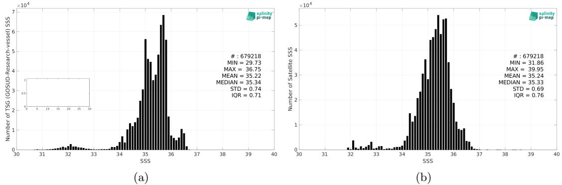
Figure 2: Histograms of SSS from TSG (GOSUD-Research-vessel) (a) and SMOS SSS L3 v8 - 9 Days (CATDS-CEC-LOCEAN) (b) considering all match-up pairs per bins of 0.1 over the South Pacific Ocean Pi-MEP region and for the full satellite product period.
