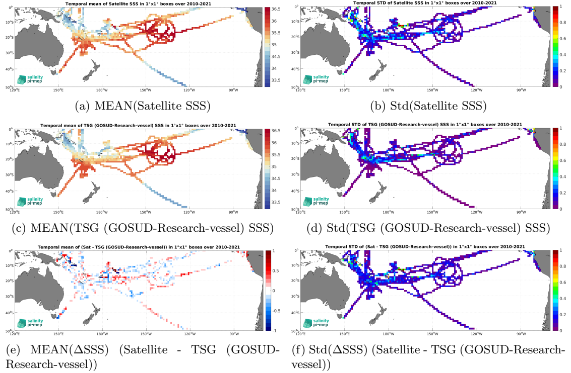
Figure 6: Temporal mean (left) and Std (right) of SSS from SMOS SSS L3 v8 - 9 Days (CATDS-CEC-LOCEAN) (top), TSG (GOSUD-Research-vessel) (middle), and of \Delta SSS (Satellite - TSG (GOSUD-Research-vessel)). Only match-up pairs are used to generate these maps.
