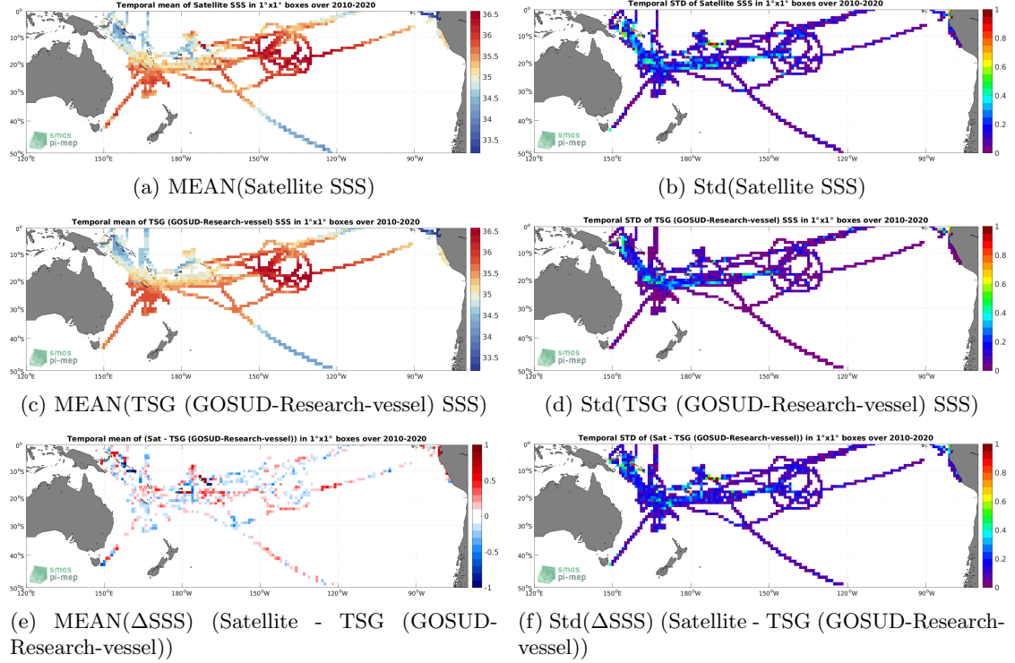
Figure 6: Temporal mean (left) and Std (right) of SSS from SMOS SSS L3 v8 - 9 Days (CATDS-CECOS-LOCEAN) (top), TSG (GOSUD-Research-vessel) (middle), and of \Delta SSS (Satellite - TSG (GOSUD-Research-vessel)). Only match-up pairs are used to generate these maps.
