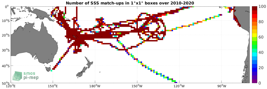
Figure 4: Number of SSS match-ups between TSG (GOSUD-Research-vessel) SSS and the SMOS SSS L3 v8 - 9 Days (CATDS-CECOS-LOCEAN) SSS product for the South Pacific Ocean Pi-MEP region over 1^\circ \times 1^\circ boxes and for the full satellite product period.
