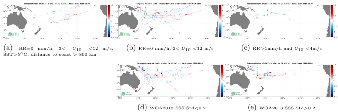
Figure 12: Temporal mean gridded over spatial boxes of size 1^\circ \times 1^\circ of \Delta SSS (SMOS SSS L3 v8 - 9 Days (CATDS-CECOS-LOCEAN) - TSG (GOSUD-Research-vessel)) for 5 different subdatasets corresponding to:RR=0 mm/h, 3 < U_{10} < 12 m/s, SST>5°C, distance to coast > 800 km (a), RR=0 mm/h, 3 < U_{10} < 12 m/s (b), RR>1mm/h and U_{10} < 4 m/s (c), WOA2013 SSS Std<0.2 (d), WOA2013 SSS Std>0.2 (e).
