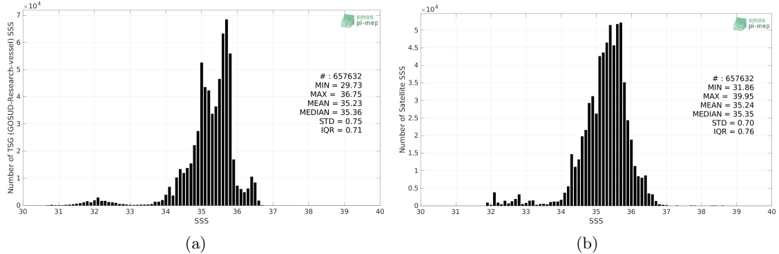
Figure 2: Histograms of SSS from TSG (GOSUD-Research-vessel) (a) and SMOS SSS L3 v8 - 9 Days (CATDS-CECOS-LOCEAN) (b) considering all match-up pairs per bins of 0.1 over the South Pacific Ocean Pi-MEP region and for the full satellite product period.
