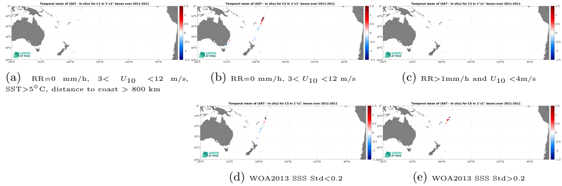
Figure 12: Temporal mean gridded over spatial boxes of size 1^{\circ}\times 1^{\circ} of \Delta\text{SSS} (SMOS SSS L3 v8 - 9 Days (CATDS-CEC-LOCEAN) - TSG (CSIC-UTM)) for 5 different subdatasets corresponding to:RR=0 mm/h, 3 < U_{10} < 12 m/s, SST > 5^{\circ}\text{C} , distance to coast > 800 km (a), RR=0 mm/h, 3 < U_{10} < 12 m/s (b), RR > 1 mm/h and U_{10} < 4 m/s (c), WOA2013 SSS Std < 0.2 (d), WOA2013 SSS Std > 0.2 (e).
