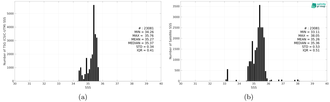
Figure 2: Histograms of SSS from TSG (CSIC-UTM) (a) and SMOS SSS L3 v8 - 9 Days (CATDS-CEC-LOCEAN) (b) considering all match-up pairs per bins of 0.1 over the South Pacific Ocean Pi-MEP region and for the full satellite product period.
