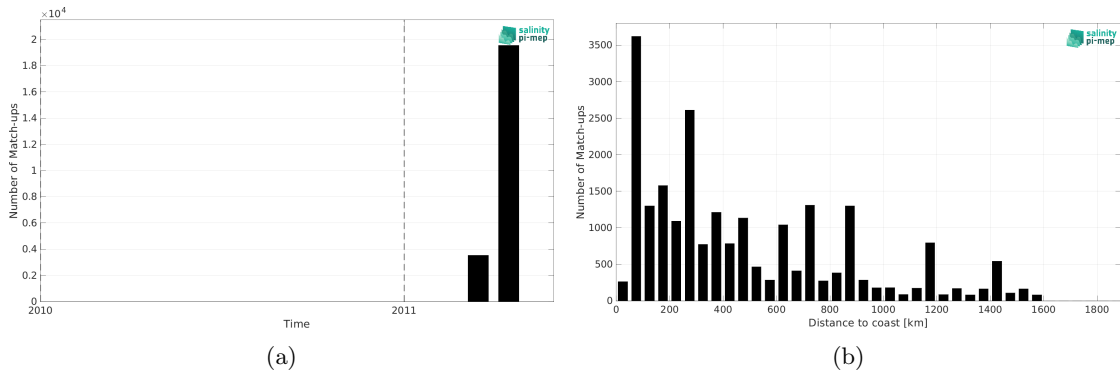
Figure 1: Number of match-ups between TSG (CSIC-UTM) and SMOS SSS L3 v8 - 9 Days (CATDS-CEC-LOCEAN) SSS as a function of time (a) and as function of the distance to coast (b) over the South Pacific Ocean Pi-MEP region and for the full satellite product period.
