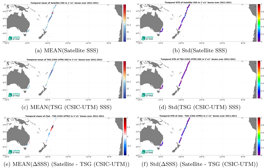
Figure 6: Temporal mean (left) and Std (right) of SSS from SMOS SSS L3 v8 - 9 Days (CATDS-CEC-LOCEAN) (top), TSG (CSIC-UTM) (middle), and of \Delta SSS (Satellite - TSG (CSIC-UTM)). Only match-up pairs are used to generate these maps.
