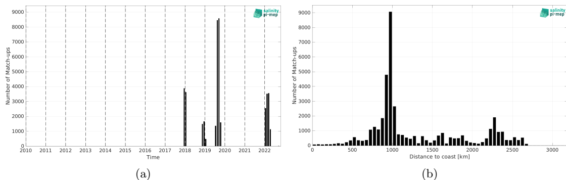
Figure 1: Number of match-ups between Saildrone and SMOS SSS L3 v8 - 9 Days (CATDS-CEC-LOCEAN) SSS as a function of time (a) and as function of the distance to coast (b) over the South Pacific Ocean Pi-MEP region and for the full satellite product period.
