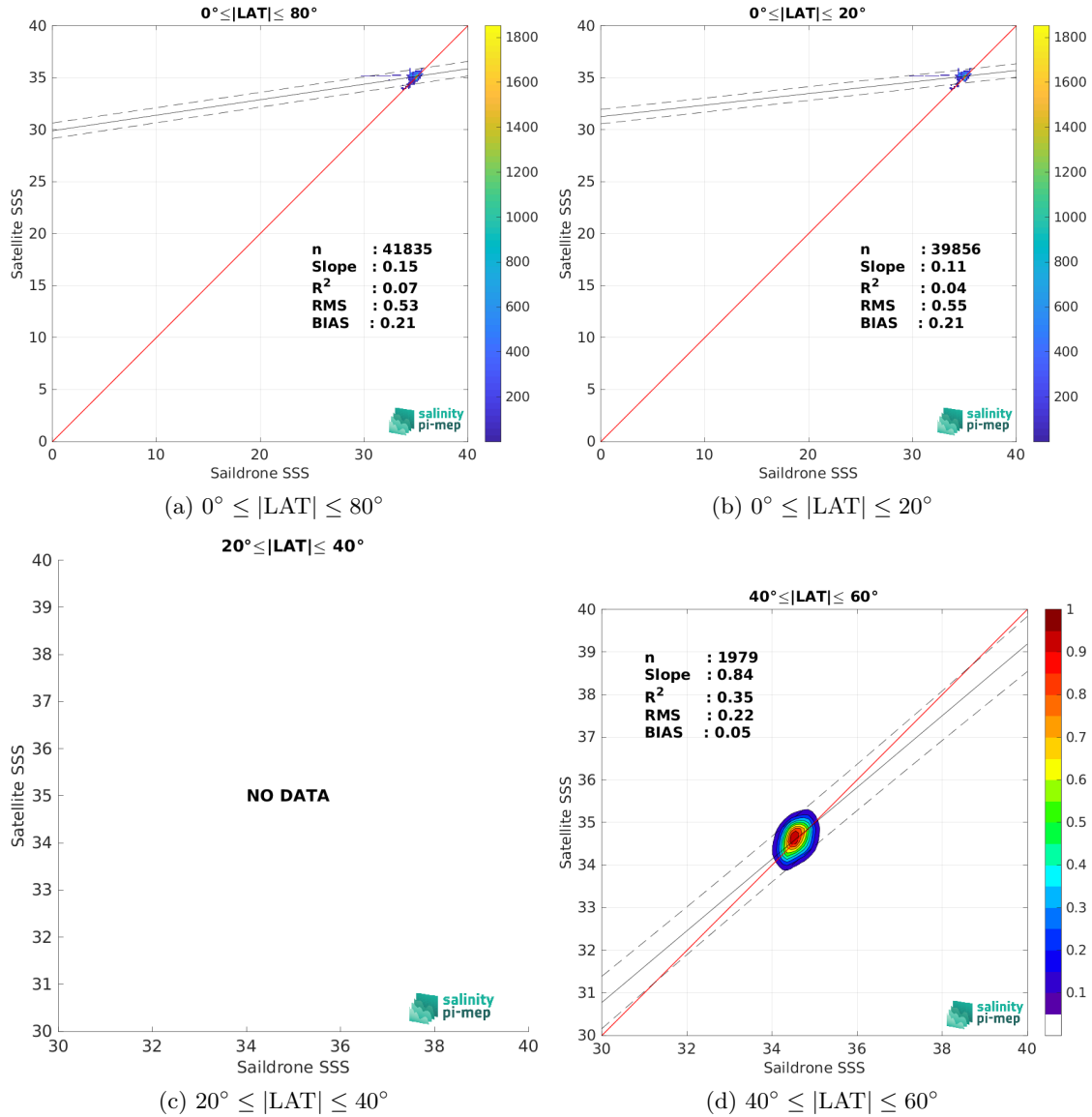
Figure 9: Contour maps of the concentration of SMOS SSS L3 v8 - 9 Days (CATDS-CEC-LOCEAN) SSS (y-axis) versus Sairdron SSS (x-axis) at match-up pairs for different latitude bands. For each plot, the red line shows x=y . The black thin and dashed lines indicate a linear fit through the data cloud and the \pm 95\% confidence levels, respectively. The number match-up pairs n , the slope and R^2 coefficient of the linear fit, the root mean square (RMS) and the mean bias between satellite and in situ data are indicated for each latitude band in each plots.
