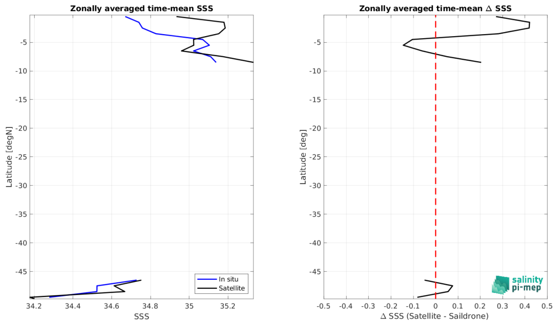
Figure 8: Left panel: Zonal mean SSS from SMOS SSS L3 v8 - 9 Days (CATDS-CEC-LOCEAN) satellite product (black) and from Sairdron (blue). Right panel: Zonal mean of \Delta SSS (Satellite - Sairdron) for all the collected Pi-MEP match-up pairs estimated over the full satellite product period.
