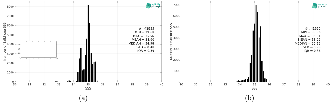
Figure 2: Histograms of SSS from Saildrone (a) and SMOS SSS L3 v8 - 9 Days (CATDS-CEC-LOCEAN) (b) considering all match-up pairs per bins of 0.1 over the South Pacific Ocean Pi-MEP region and for the full satellite product period.
