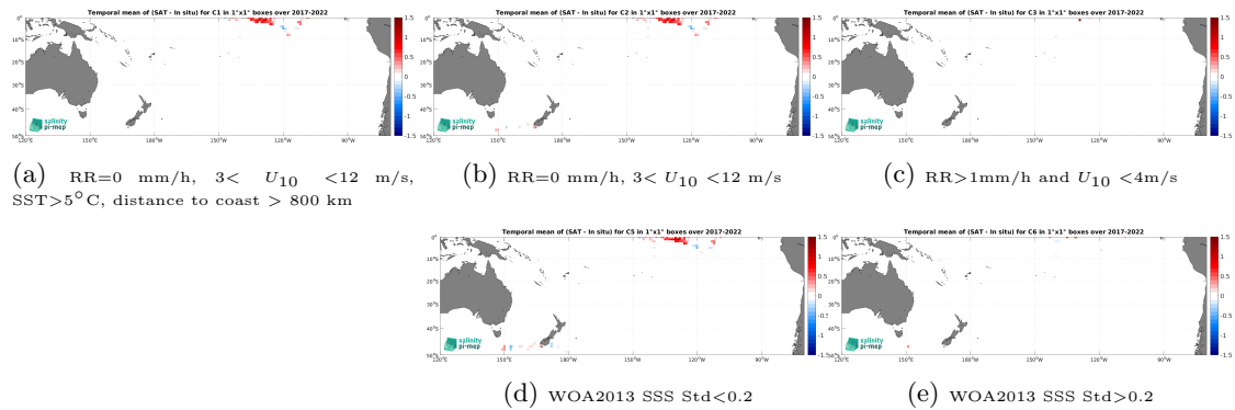
Figure 12: Temporal mean gridded over spatial boxes of size 1^\circ \times 1^\circ of \Delta SSS (SMOS SSS L3 v8 - 9 Days (CATDS-CEC-LOCEAN) - Saildrone) for 5 different subdatasets corresponding to:RR=0 mm/h, 3 < U_{10} < 12 m/s, SST >5^\circ\text{C} , distance to coast > 800 km (a), RR=0 mm/h, 3 < U_{10} < 12 m/s (b), RR >1 mm/h and U_{10} < 4 m/s (c), WOA2013 SSS Std <0.2 (d), WOA2013 SSS Std >0.2 (e).
