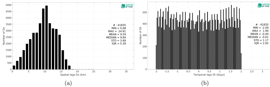
Figure 5: Histograms of the spatial (a) and temporal (b) lags between the location/time of the Saildrone measurement and the date of the corresponding SMOS SSS L3 v8 - 9 Days (CATDS-CEC-LOCEAN) SSS pixel.
