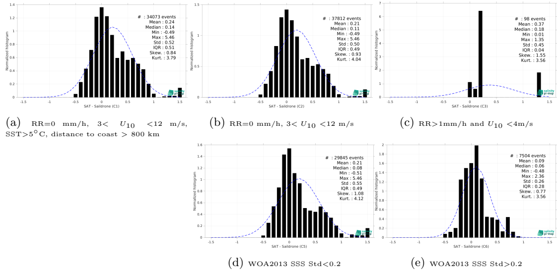
Figure 13: Normalized histogram of \Delta SSS (SMOS SSS L3 v8 - 9 Days (CATDS-CEC-LOCEAN) - Saildrone) for 5 different subdatasets corresponding to: RR=0 mm/h, 3 < U_{10} < 12 m/s, SST > 5°C, distance to coast > 800 km (a), RR=0 mm/h, 3 < U_{10} < 12 m/s (b), RR > 1mm/h and U_{10} < 4 m/s (c), WOA2013 SSS Std < 0.2 (d), WOA2013 SSS Std > 0.2 (e).
