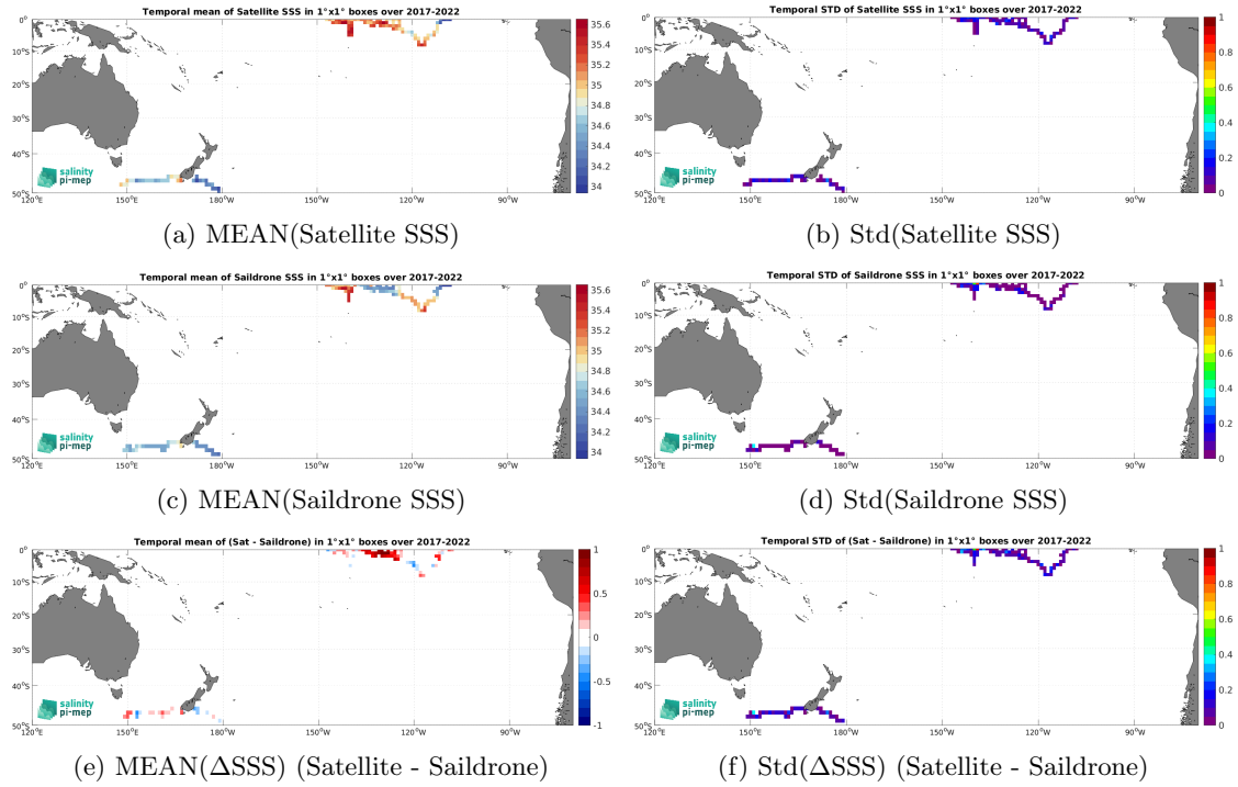
Figure 6: Temporal mean (left) and Std (right) of SSS from SMOS SSS L3 v8 - 9 Days (CATDS-CEC-LOCEAN) (top), Saildrone (middle), and of \Delta SSS (Satellite - Saildrone). Only match-up pairs are used to generate these maps.
