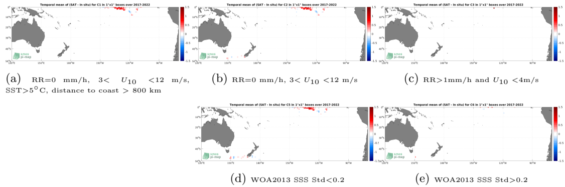
Figure 12: Temporal mean gridded over spatial boxes of size 1^\circ \times 1^\circ of \Delta SSS (SMOS SSS L3 v8 - 9 Days (CATDS-CECOS-LOCEAN) - Saildrone) for 5 different subdatasets corresponding to:RR=0 mm/h, 3 < U_{10} < 12 m/s, SST >5^\circ C, distance to coast > 800 km (a), RR=0 mm/h, 3 < U_{10} < 12 m/s (b), RR >1 mm/h and U_{10} < 4 m/s (c), WOA2013 SSS Std <0.2 (d), WOA2013 SSS Std >0.2 (e).
