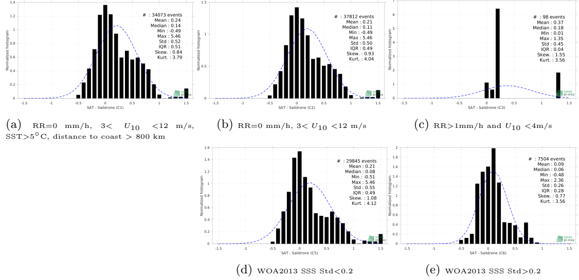
Figure 13: Normalized histogram of \Delta SSS (SMOS SSS L3 v8 - 9 Days (CATDS-CECOS-LOCEAN) - Saildrone) for 5 different subdatasets corresponding to: RR=0 mm/h, 3 < U_{10} < 12 m/s, SST > 5°C, distance to coast > 800 km (a), RR=0 mm/h, 3 < U_{10} < 12 m/s (b), RR > 1mm/h and U_{10} < 4 m/s (c), WOA2013 SSS Std < 0.2 (d), WOA2013 SSS Std > 0.2 (e).
