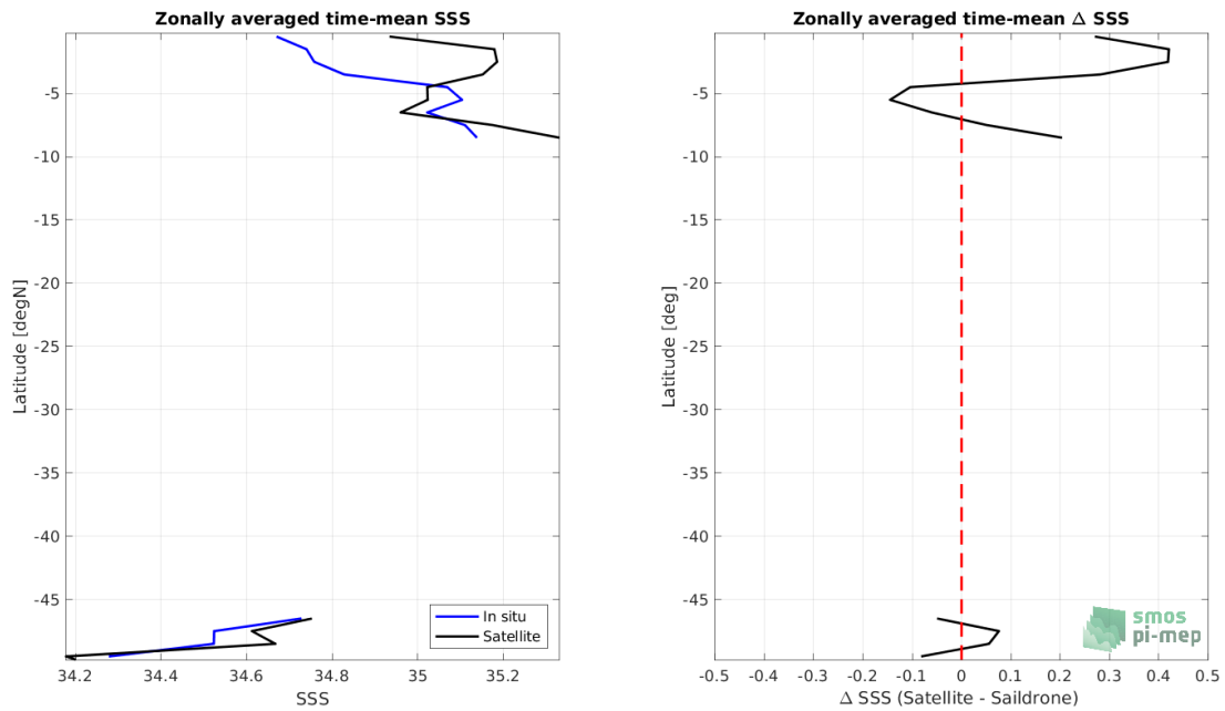
Figure 8: Left panel: Zonal mean SSS from SMOS SSS L3 v8 - 9 Days (CATDS-CECOS-LOCEAN) satellite product (black) and from Sairdrone (blue). Right panel: Zonal mean of \Delta SSS (Satellite - Sairdrone) for all the collected Pi-MEP match-up pairs estimated over the full satellite product period.
