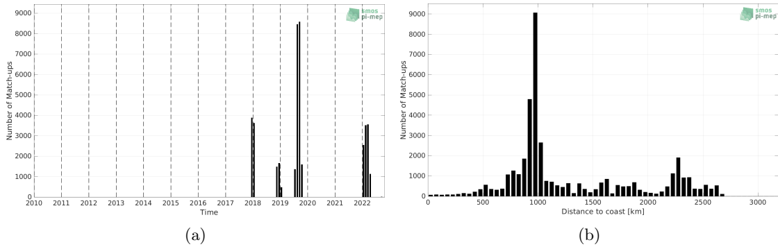
Figure 1: Number of match-ups between Saildrone and SMOS SSS L3 v8 - 9 Days (CATDS-CECOS-LOCEAN) SSS as a function of time (a) and as function of the distance to coast (b) over the South Pacific Ocean Pi-MEP region and for the full satellite product period.
