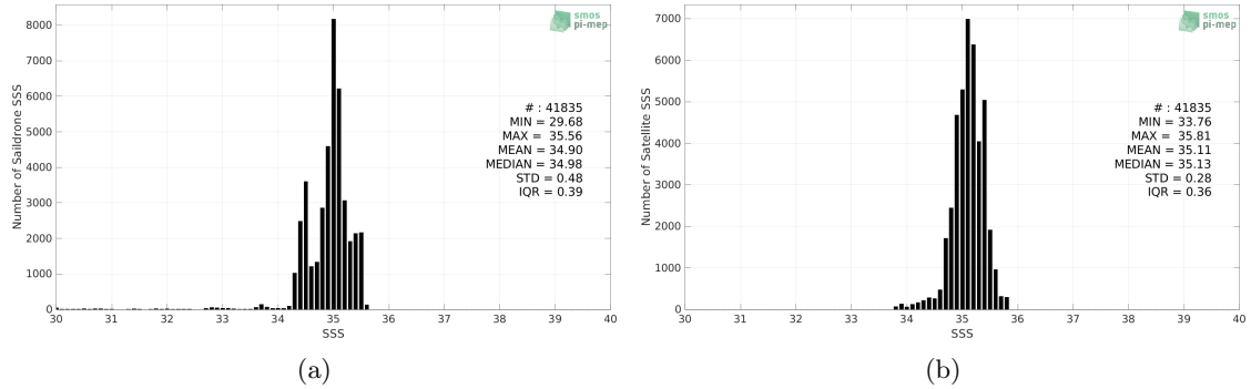
Figure 2: Histograms of SSS from Saildrone (a) and SMOS SSS L3 v8 - 9 Days (CATDS-CECOS-LOCEAN) (b) considering all match-up pairs per bins of 0.1 over the South Pacific Ocean Pi-MEP region and for the full satellite product period.
