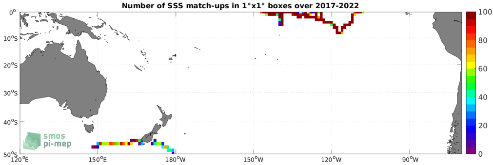
Figure 4: Number of SSS match-ups between Saildrone SSS and the SMOS SSS L3 v8 - 9 Days (CATDS-CECOS-LOCEAN) SSS product for the South Pacific Ocean Pi-MEP region over 1^\circ \times 1^\circ boxes and for the full satellite product period.
