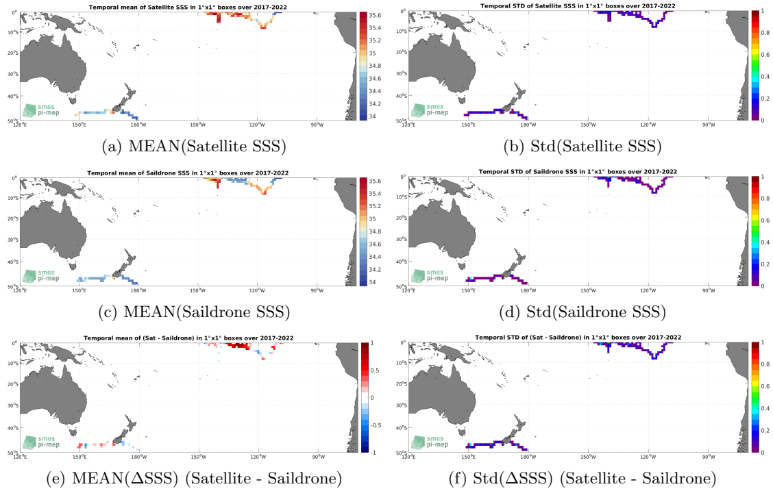
Figure 6: Temporal mean (left) and Std (right) of SSS from SMOS SSS L3 v8 - 9 Days (CATDS-CECOS-LOCEAN) (top), Saildrone (middle), and of \Delta SSS (Satellite - Saildrone). Only match-up pairs are used to generate these maps.
