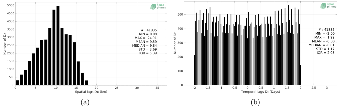
Figure 5: Histograms of the spatial (a) and temporal (b) lags between the location/time of the Saildrone measurement and the date of the corresponding SMOS SSS L3 v8 - 9 Days (CATDS-CECOS-LOCEAN) SSS pixel.
