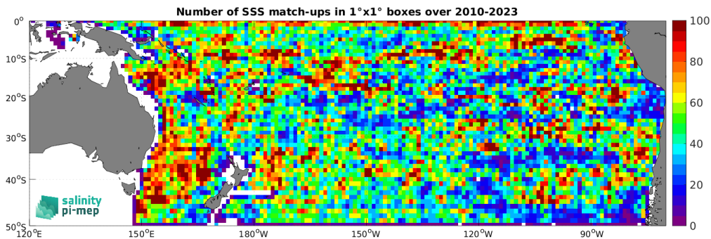
Figure 4: Number of SSS match-ups between Argo SSS and the SMOS SSS L3 v8 - 9 Days (CATDS-CEC-LOCEAN) SSS product for the South Pacific Ocean Pi-MEP region over 1^\circ \times 1^\circ boxes and for the full satellite product period.
