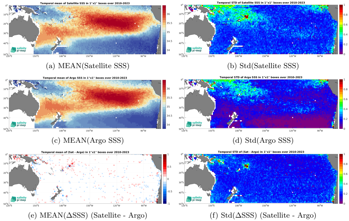
Figure 6: Temporal mean (left) and Std (right) of SSS from SMOS SSS L3 v8 - 9 Days (CATDS-CEC-LOCEAN) (top), Argo (middle), and of \Delta SSS (Satellite - Argo). Only match-up pairs are used to generate these maps.
