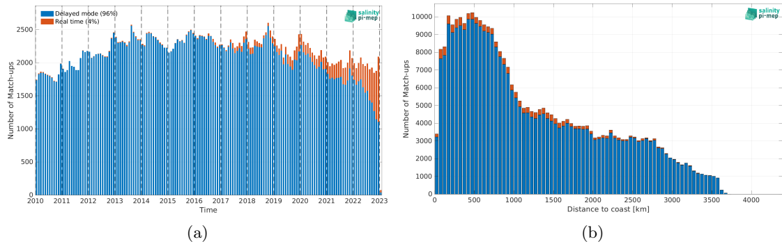
Figure 1: Number of match-ups between Argo and SMOS SSS L3 v8 - 9 Days (CATDS-CEC-LOCEAN) SSS as a function of time (a) and as function of the distance to coast (b) over the South Pacific Ocean Pi-MEP region and for the full satellite product period.
