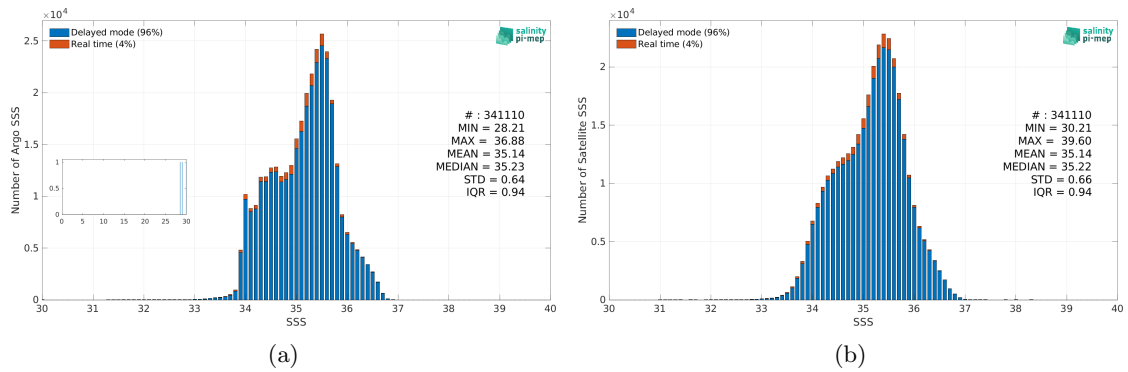
Figure 2: Histograms of SSS from Argo (a) and SMOS SSS L3 v8 - 9 Days (CATDS-CEC-LOCEAN) (b) considering all match-up pairs per bins of 0.1 over the South Pacific Ocean Pi-MEP region and for the full satellite product period.
