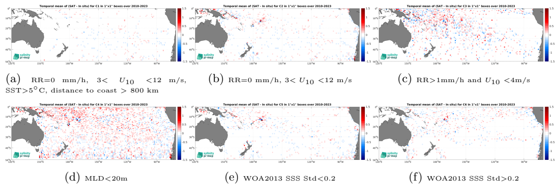
Figure 12: Temporal mean gridded over spatial boxes of size 1^\circ \times 1^\circ of \Delta SSS (SMOS SSS L3 v8 - 9 Days (CATDS-CEC-LOCEAN) - Argo) for 6 different subdatasets corresponding to:RR=0 mm/h, 3 < U_{10} < 12 m/s, SST >5^\circ C, distance to coast > 800 km (a), RR=0 mm/h, 3 < U_{10} < 12 m/s (b), RR >1 mm/h and U_{10} < 4 m/s (c),MLD <20 m (d),WOA2013 SSS Std <0.2 (e),WOA2013 SSS Std >0.2 (f).
