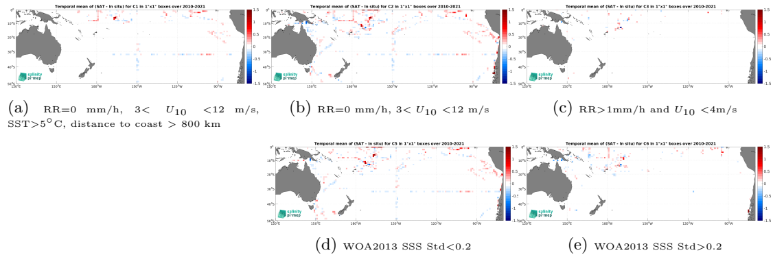
Figure 12: Temporal mean gridded over spatial boxes of size 1^\circ \times 1^\circ of \Delta SSS (SMOS SSS L3 v8 - 18 Days (CATDS-CEC-LOCEAN) - TSG (SAMOS)) for 5 different subdatasets corresponding to:RR=0 mm/h, 3 < U_{10} < 12 m/s, SST >5^\circ C, distance to coast > 800 km (a), RR=0 mm/h, 3 < U_{10} < 12 m/s (b), RR >1 mm/h and U_{10} < 4 m/s (c), WOA2013 SSS Std <0.2 (d), WOA2013 SSS Std >0.2 (e).
