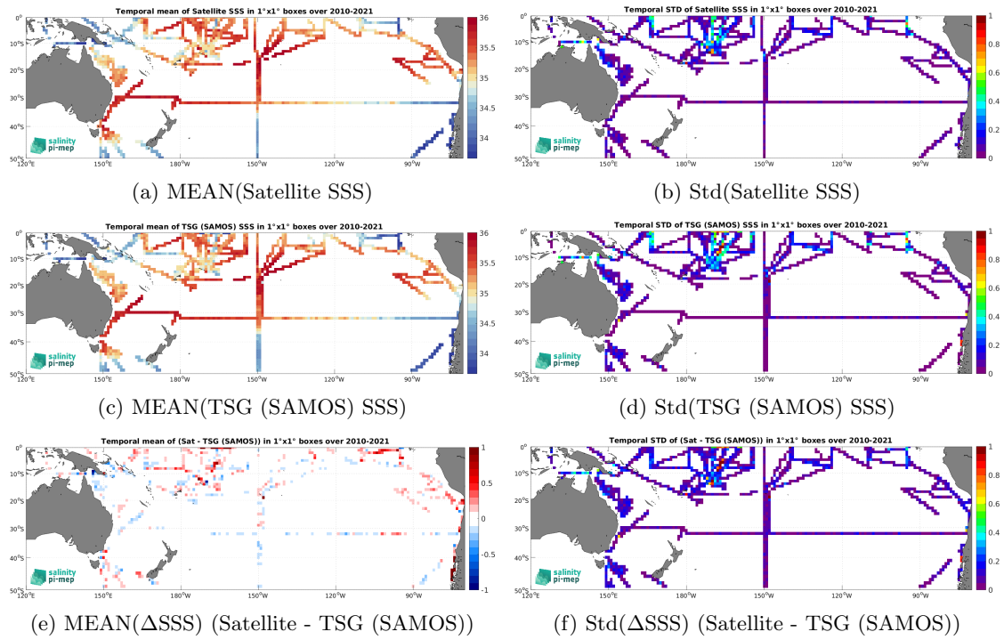
Figure 6: Temporal mean (left) and Std (right) of SSS from SMOS SSS L3 v8 - 18 Days (CATDS-CEC-LOCEAN) (top), TSG (SAMOS) (middle), and of \Delta SSS (Satellite - TSG (SAMOS)). Only match-up pairs are used to generate these maps.
