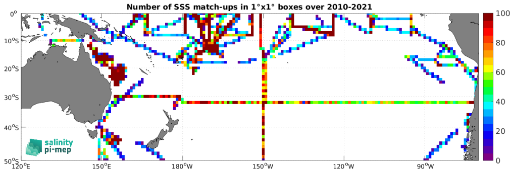
Figure 4: Number of SSS match-ups between TSG (SAMOS) SSS and the SMOS SSS L3 v8 - 18 Days (CATDS-CEC-LOCEAN) SSS product for the South Pacific Ocean Pi-MEP region over 1^\circ \times 1^\circ boxes and for the full satellite product period.
