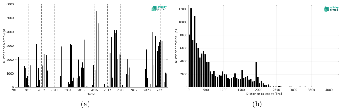
Figure 1: Number of match-ups between TSG (SAMOS) and SMOS SSS L3 v8 - 18 Days (CATDS-CEC-LOCEAN) SSS as a function of time (a) and as function of the distance to coast (b) over the South Pacific Ocean Pi-MEP region and for the full satellite product period.
