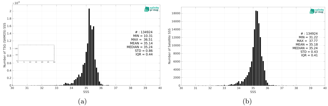
Figure 2: Histograms of SSS from TSG (SAMOS) (a) and SMOS SSS L3 v8 - 18 Days (CATDS-CEC-LOCEAN) (b) considering all match-up pairs per bins of 0.1 over the South Pacific Ocean Pi-MEP region and for the full satellite product period.
