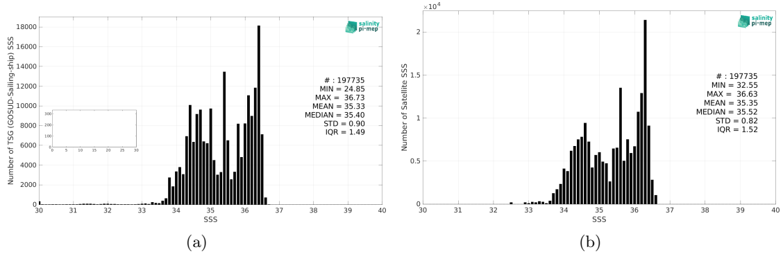
Figure 2: Histograms of SSS from TSG (GOSUD-Sailing-ship) (a) and SMOS SSS L3 v8 - 18 Days (CATDS-CEC-LOCEAN) (b) considering all match-up pairs per bins of 0.1 over the South Pacific Ocean Pi-MEP region and for the full satellite product period.
