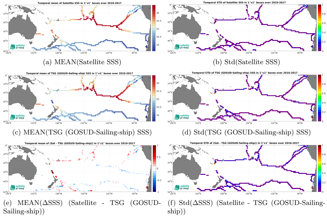
Figure 6: Temporal mean (left) and Std (right) of SSS from SMOS SSS L3 v8 - 18 Days (CATDS-CEC-LOCEAN) (top), TSG (GOSUD-Sailing-ship) (middle), and of \Delta SSS (Satellite - TSG (GOSUD-Sailing-ship)). Only match-up pairs are used to generate these maps.
