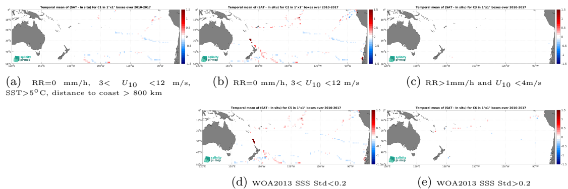
Figure 12: Temporal mean gridded over spatial boxes of size 1^\circ \times 1^\circ of \Delta\text{SSS} (SMOS SSS L3 v8 - 18 Days (CATDS-CEC-LOCEAN) - TSG (GOSUD-Sailing-ship)) for 5 different subdatasets corresponding to:RR=0 mm/h, 3 < U_{10} < 12 m/s, SST>5°C, distance to coast > 800 km (a), RR=0 mm/h, 3 < U_{10} < 12 m/s (b), RR>1mm/h and U_{10} < 4 m/s (c), WOA2013 SSS Std<0.2 (d), WOA2013 SSS Std>0.2 (e).
