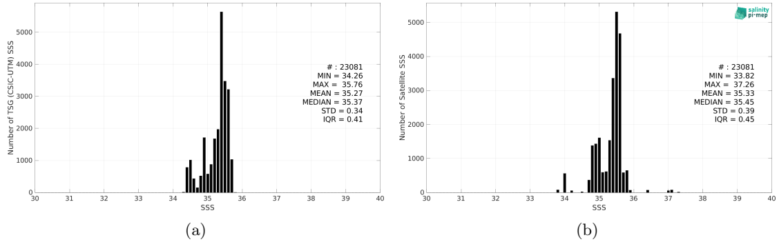
Figure 2: Histograms of SSS from TSG (CSIC-UTM) (a) and SMOS SSS L3 v8 - 18 Days (CATDS-CEC-LOCEAN) (b) considering all match-up pairs per bins of 0.1 over the South Pacific Ocean Pi-MEP region and for the full satellite product period.
