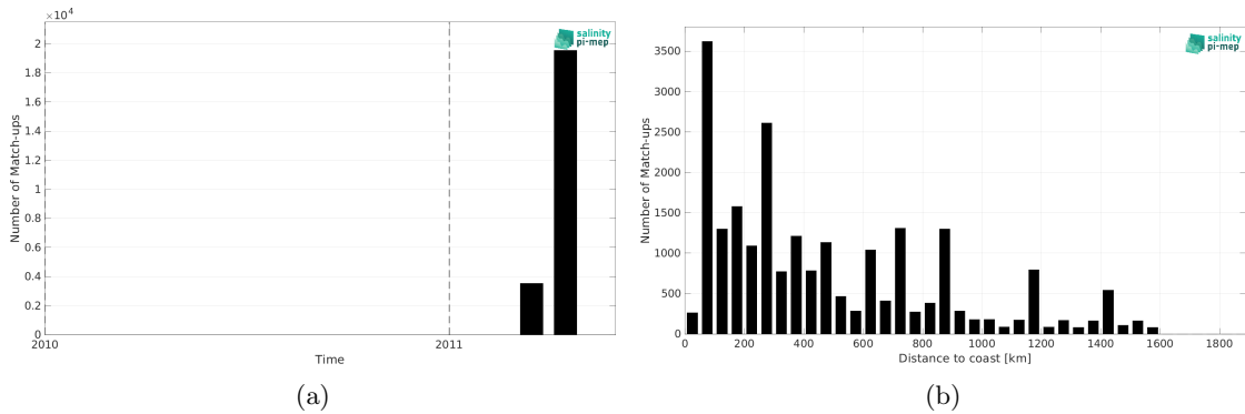
Figure 1: Number of match-ups between TSG (CSIC-UTM) and SMOS SSS L3 v8 - 18 Days (CATDS-CEC-LOCEAN) SSS as a function of time (a) and as function of the distance to coast (b) over the South Pacific Ocean Pi-MEP region and for the full satellite product period.
