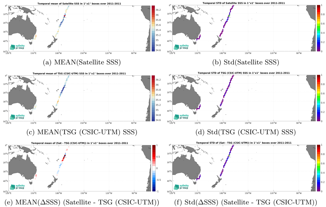
Figure 6: Temporal mean (left) and Std (right) of SSS from SMOS SSS L3 v8 - 18 Days (CATDS-CEC-LOCEAN) (top), TSG (CSIC-UTM) (middle), and of \Delta SSS (Satellite - TSG (CSIC-UTM)). Only match-up pairs are used to generate these maps.
