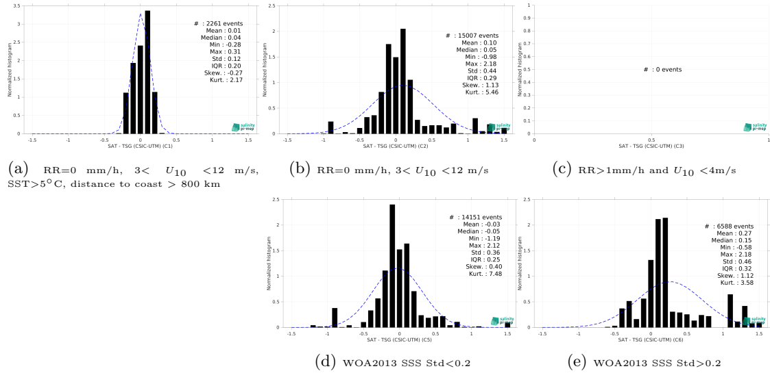
Figure 13: Normalized histogram of \Delta SSS (SMOS SSS L3 v8 - 18 Days (CATDS-CEC-LOCEAN) - TSG (CSIC-UTM)) for 5 different subdatasets corresponding to: RR=0 mm/h, 3 < U_{10} < 12 m/s, SST>5°C, distance to coast > 800 km (a), RR=0 mm/h, 3 < U_{10} < 12 m/s (b), RR>1mm/h and U_{10} < 4 m/s (c), WOA2013 SSS Std<0.2 (d), WOA2013 SSS Std>0.2 (e).
