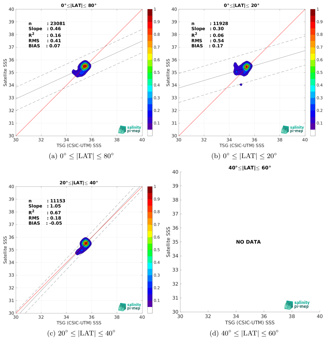
Figure 9: Contour maps of the concentration of SMOS SSS L3 v8 - 18 Days (CATDS-CEC-LOCEAN) SSS (y-axis) versus TSG (CSIC-UTM) SSS (x-axis) at match-up pairs for different latitude bands. For each plot, the red line shows x=y . The black thin and dashed lines indicate a linear fit through the data cloud and the \pm 95\% confidence levels, respectively. The number match-up pairs n , the slope and R^2 coefficient of the linear fit, the root mean square (RMS) and the mean bias between satellite and in situ data are indicated for each latitude band in each plots.
