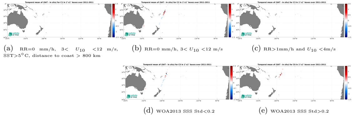
Figure 12: Temporal mean gridded over spatial boxes of size 1^{\circ}\times 1^{\circ} of \Delta\text{SSS} (SMOS SSS L3 v8 - 18 Days (CATDS-CEC-LOCEAN) - TSG (CSIC-UTM)) for 5 different subdatasets corresponding to: RR=0 mm/h, 3 < U_{10} < 12 m/s, SST > 5^{\circ}\text{C} , distance to coast > 800 km (a), RR=0 mm/h, 3 < U_{10} < 12 m/s (b), RR > 1 mm/h and U_{10} < 4 m/s (c), WOA2013 SSS Std < 0.2 (d), WOA2013 SSS Std > 0.2 (e).
