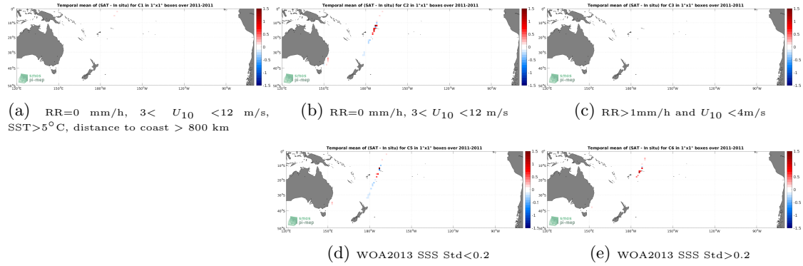
Figure 12: Temporal mean gridded over spatial boxes of size 1^{\circ}\times 1^{\circ} of \Delta\text{SSS} (SMOS SSS L3 v8 - 18 Days (CATDS-CECOS-LOCEAN) - TSG (CSIC-UTM)) for 5 different subdatasets corresponding to:RR=0 mm/h, 3 < U_{10} < 12 m/s, SST >5^{\circ}\text{C} , distance to coast > 800 km (a), RR=0 mm/h, 3 < U_{10} < 12 m/s (b), RR >1 mm/h and U_{10} < 4 m/s (c), WOA2013 SSS Std <0.2 (d), WOA2013 SSS Std >0.2 (e).
