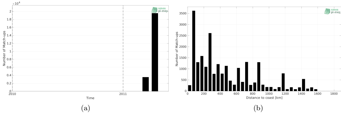
Figure 1: Number of match-ups between TSG (CSIC-UTM) and SMOS SSS L3 v8 - 18 Days (CATDS-CECOS-LOCEAN) SSS as a function of time (a) and as function of the distance to coast (b) over the South Pacific Ocean Pi-MEP region and for the full satellite product period.
