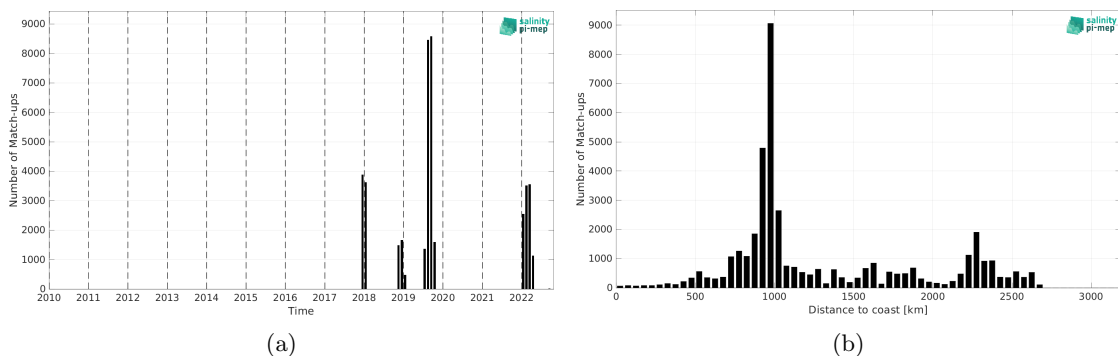
Figure 1: Number of match-ups between Saildrone and SMOS SSS L3 v8 - 18 Days (CATDS-CEC-LOCEAN) SSS as a function of time (a) and as function of the distance to coast (b) over the South Pacific Ocean Pi-MEP region and for the full satellite product period.
