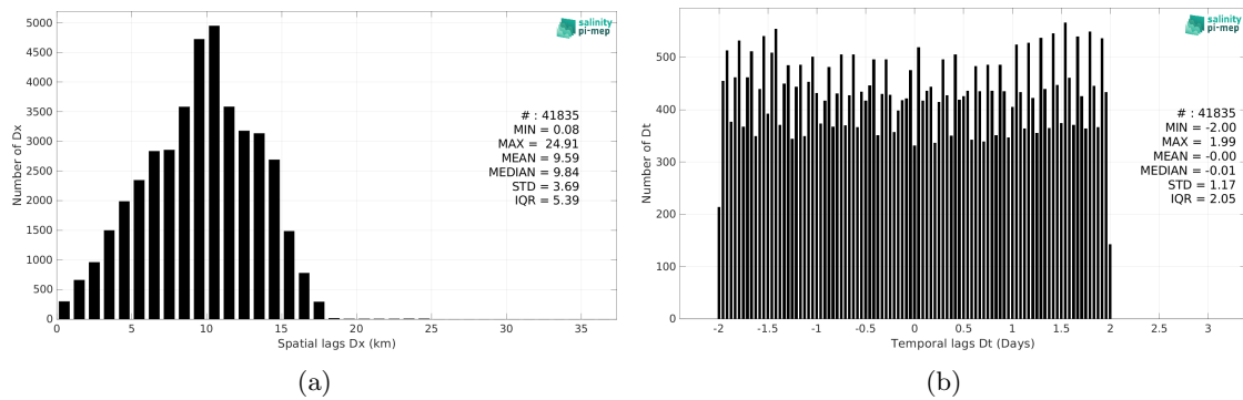
Figure 5: Histograms of the spatial (a) and temporal (b) lags between the location/time of the Saildrone measurement and the date of the corresponding SMOS SSS L3 v8 - 18 Days (CATDS-CEC-LOCEAN) SSS pixel.
