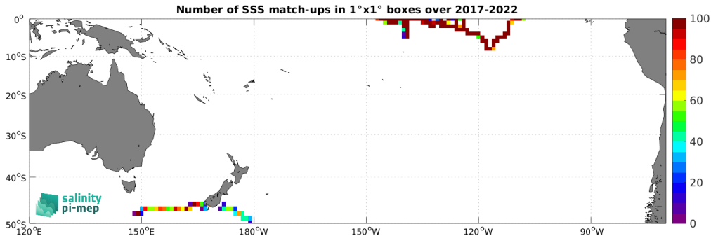
Figure 4: Number of SSS match-ups between Saildrone SSS and the SMOS SSS L3 v8 - 18 Days (CATDS-CEC-LOCEAN) SSS product for the South Pacific Ocean Pi-MEP region over 1^\circ \times 1^\circ boxes and for the full satellite product period.
