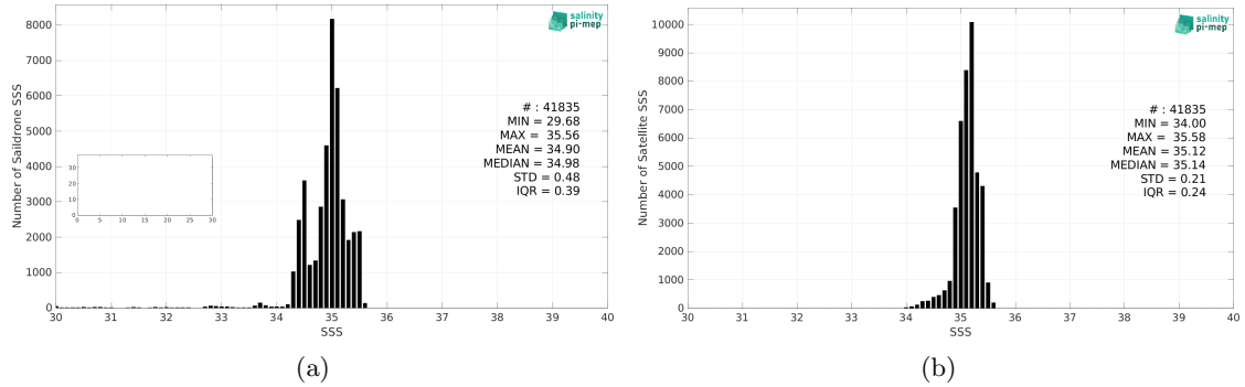
Figure 2: Histograms of SSS from Saildrone (a) and SMOS SSS L3 v8 - 18 Days (CATDS-CEC-LOCEAN) (b) considering all match-up pairs per bins of 0.1 over the South Pacific Ocean Pi-MEP region and for the full satellite product period.
