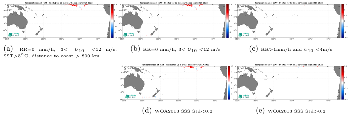
Figure 12: Temporal mean gridded over spatial boxes of size 1^\circ \times 1^\circ of \Delta SSS (SMOS SSS L3 v8 - 18 Days (CATDS-CEC-LOCEAN) - Sairdrone) for 5 different subdatasets corresponding to:RR=0 mm/h, 3 < U_{10} < 12 m/s, SST >5^\circ\text{C} , distance to coast > 800 km (a), RR=0 mm/h, 3 < U_{10} < 12 m/s (b), RR >1 mm/h and U_{10} < 4 m/s (c), WOA2013 SSS Std <0.2 (d), WOA2013 SSS Std >0.2 (e).
