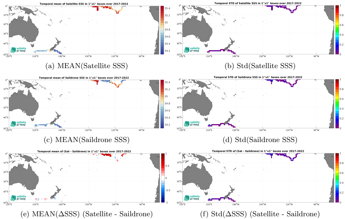
Figure 6: Temporal mean (left) and Std (right) of SSS from SMOS SSS L3 v8 - 18 Days (CATDS-CEC-LOCEAN) (top), Saildrone (middle), and of \Delta SSS (Satellite - Saildrone). Only match-up pairs are used to generate these maps.
