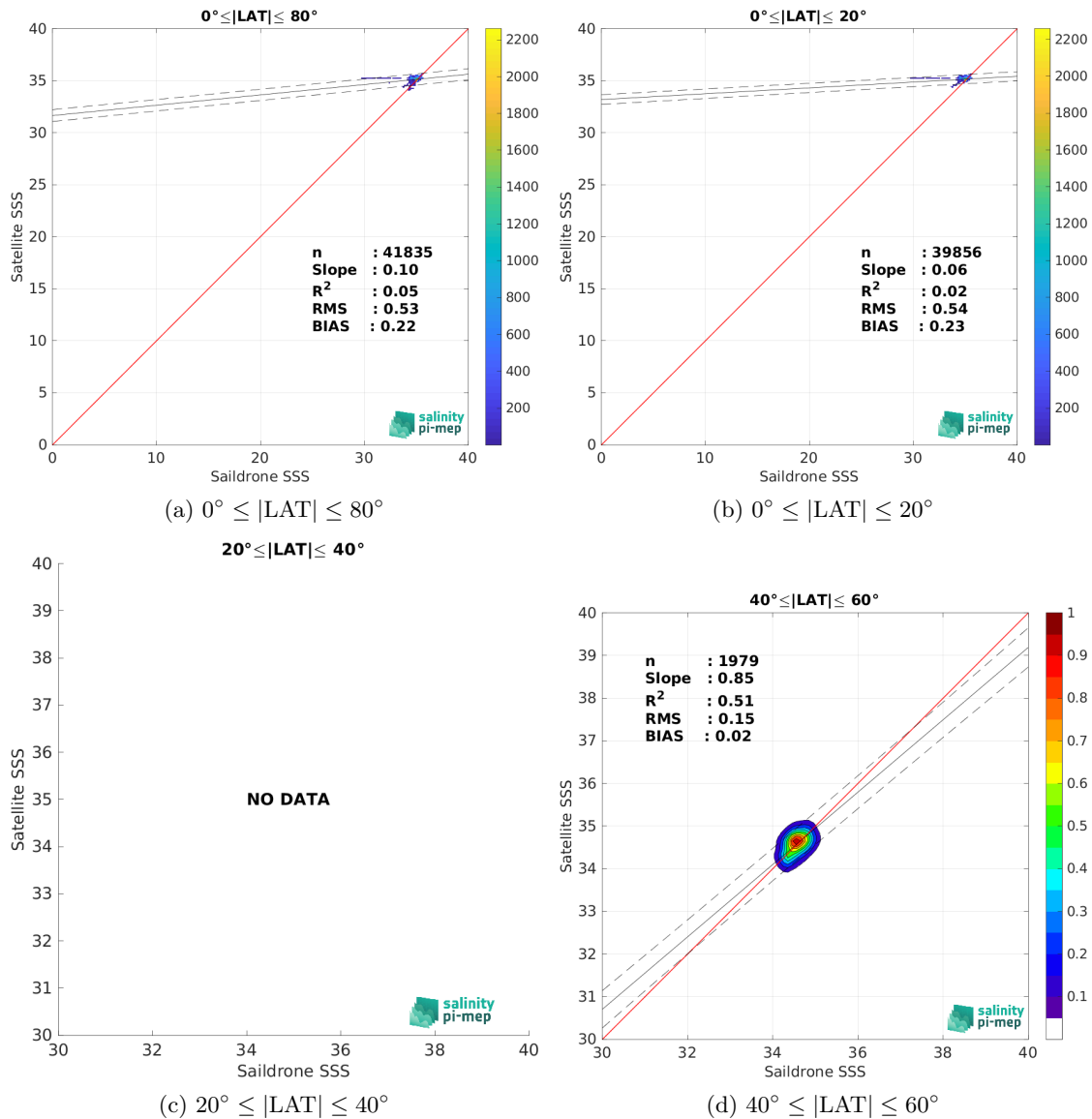
Figure 9: Contour maps of the concentration of SMOS SSS L3 v8 - 18 Days (CATDS-CEC-LOCEAN) SSS (y-axis) versus Saildrone SSS (x-axis) at match-up pairs for different latitude bands. For each plot, the red line shows x=y . The black thin and dashed lines indicate a linear fit through the data cloud and the \pm 95\% confidence levels, respectively. The number match-up pairs n , the slope and R^2 coefficient of the linear fit, the root mean square (RMS) and the mean bias between satellite and in situ data are indicated for each latitude band in each plots.
