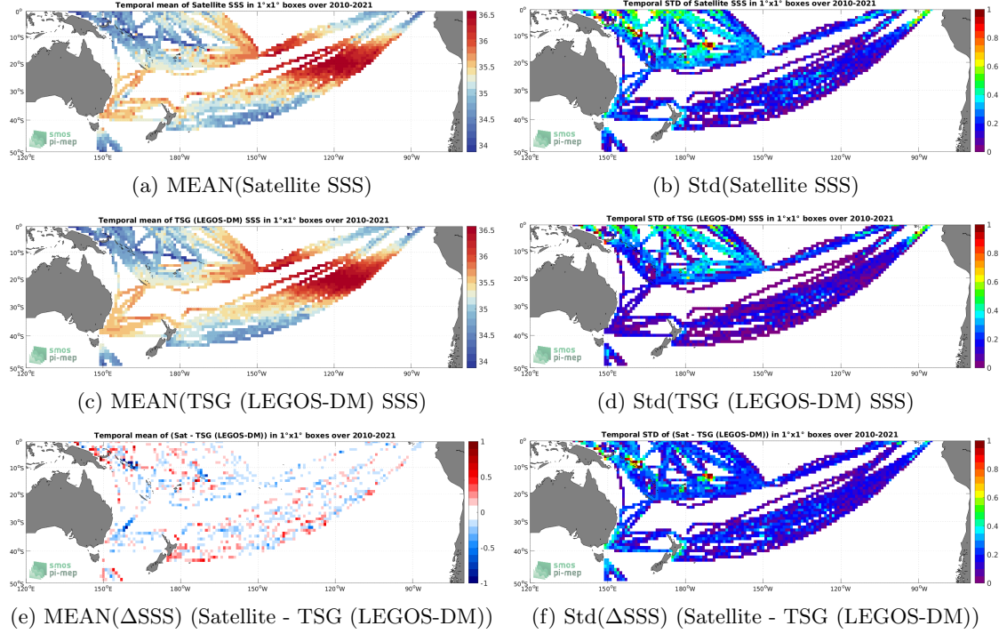
Figure 6: Temporal mean (left) and Std (right) of SSS from SMOS SSS L3 v7 - 9 Days (CATDS-CECOS-LOCEAN) (top), TSG (LEGOS-DM) ( in situ ) dataset (middle), and of \Delta SSS (Satellite - TSG (LEGOS-DM)). Only match-up pairs are used to generate these maps.
