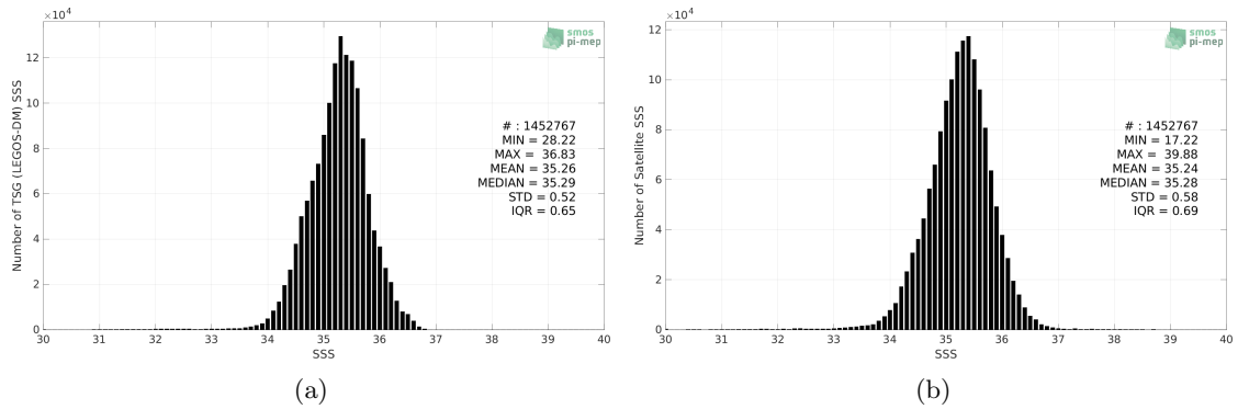
Figure 2: Histograms of SSS from TSG (LEGOS-DM) (a) and SMOS SSS L3 v7 - 9 Days (CATDS-CECOS-LOCEAN) (b) considering all match-up pairs per bins of 0.1 over the South Pacific Ocean Pi-MEP region and for the full satellite product period.
