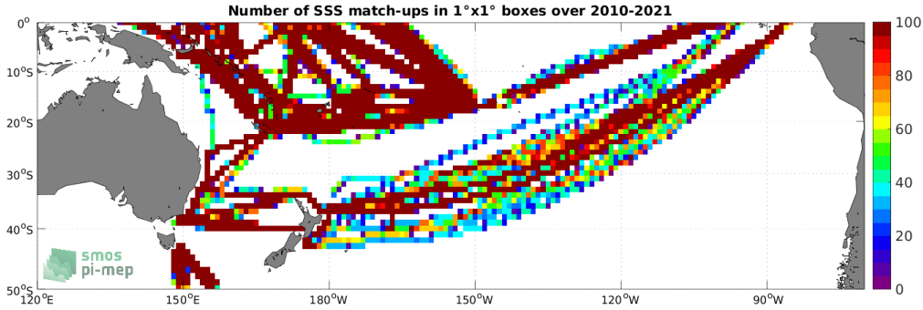
Figure 4: Number of SSS match-ups between TSG (LEGOS-DM) SSS and the SMOS SSS L3 v7 - 9 Days (CATDS-CECOS-LOCEAN) SSS product for the South Pacific Ocean Pi-MEP region over 1^\circ \times 1^\circ boxes and for the full satellite product period.
