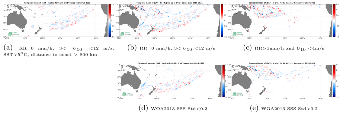
Figure 12: Temporal mean gridded over spatial boxes of size 1^\circ \times 1^\circ of \Delta SSS (SMOS SSS L3 v7 - 9 Days (CATDS-CECOS-LOCEAN) - TSG (LEGOS-DM)) for 5 different subdatasets corresponding to:RR=0 mm/h, 3 < U_{10} < 12 m/s, SST >5^\circ\text{C} , distance to coast > 800 km (a), RR=0 mm/h, 3 < U_{10} < 12 m/s (b), RR >1 mm/h and U_{10} < 4 m/s (c), WOA2013 SSS Std <0.2 (d), WOA2013 SSS Std >0.2 (e).
