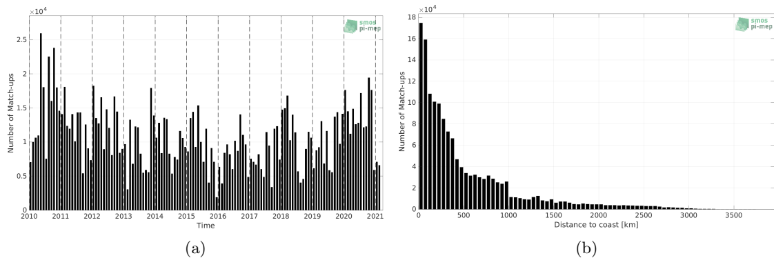
Figure 1: Number of match-ups between TSG (LEGOS-DM) and SMOS SSS L3 v7 - 9 Days (CATDS-CECOS-LOCEAN) SSS as a function of time (a) and as function of the distance to coast (b) over the South Pacific Ocean Pi-MEP region and for the full satellite product period.
