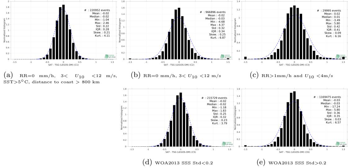
Figure 13: Normalized histogram of \Delta\text{SSS} (SMOS SSS L3 v7 - 9 Days (CATDS-CECOS-LOCEAN) - TSG (LEGOS-DM)) for 5 different subdatasets corresponding to: RR=0 mm/h, 3 < U_{10} < 12 m/s, SST>5°C, distance to coast > 800 km (a), RR=0 mm/h, 3 < U_{10} < 12 m/s (b), RR>1mm/h and U_{10} < 4 m/s (c), WOA2013 SSS Std<0.2 (d), WOA2013 SSS Std>0.2 (e).
