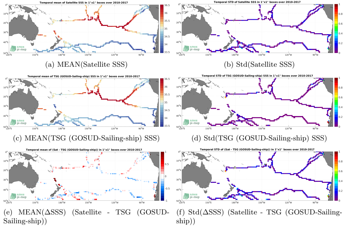
Figure 6: Temporal mean (left) and Std (right) of SSS from SMOS SSS L3 v7 - 9 Days (CATDS-CECOS-LOCEAN) (top), TSG (GOSUD-Sailing-ship) (middle), and of \Delta SSS (Satellite - TSG (GOSUD-Sailing-ship)). Only match-up pairs are used to generate these maps.
