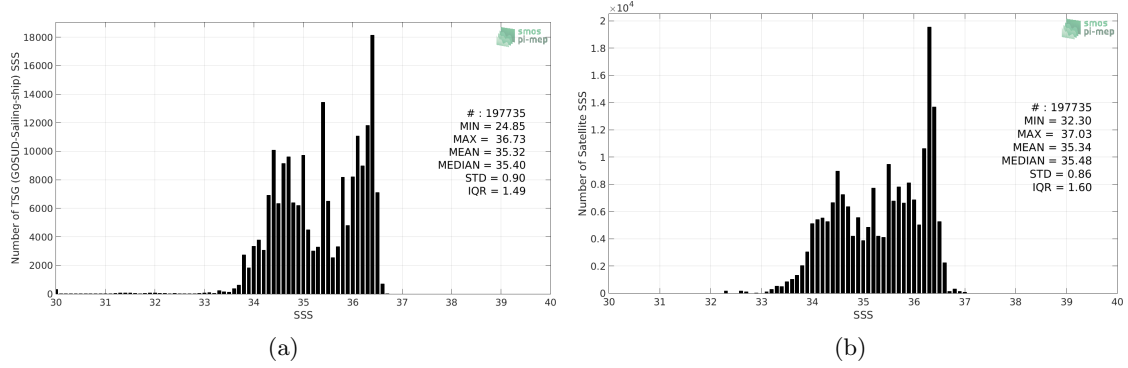
Figure 2: Histograms of SSS from TSG (GOSUD-Sailing-ship) (a) and SMOS SSS L3 v7 - 9 Days (CATDS-CECOS-LOCEAN) (b) considering all match-up pairs per bins of 0.1 over the South Pacific Ocean Pi-MEP region and for the full satellite product period.
