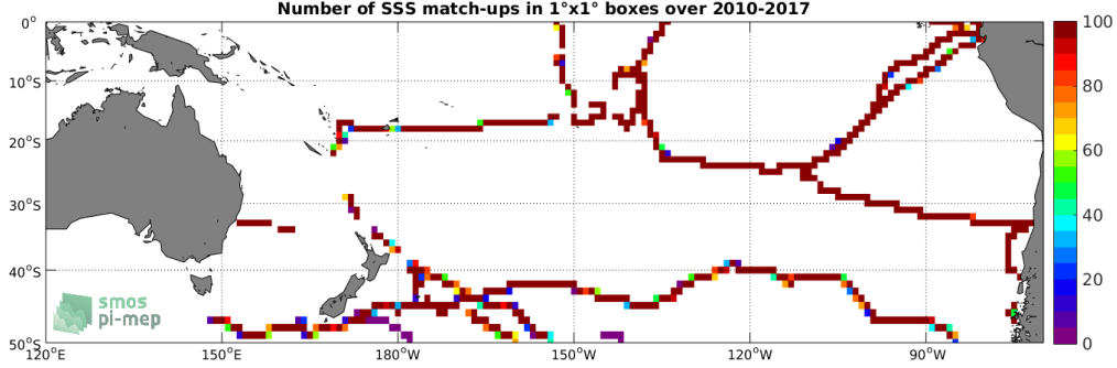
Figure 4: Number of SSS match-ups between TSG (GOSUD-Sailing-ship) SSS and the SMOS SSS L3 v7 - 9 Days (CATDS-CECOS-LOCEAN) SSS product for the South Pacific Ocean Pi-MEP region over 1^\circ \times 1^\circ boxes and for the full satellite product period.
