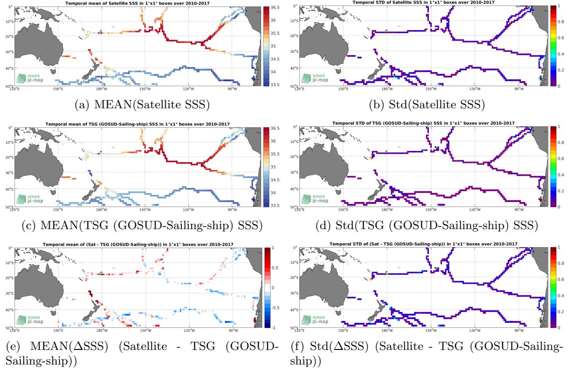
Figure 6: Temporal mean (left) and Std (right) of SSS from SMOS SSS L3 v7 - 9 Days (CATDS-CECOS-LOCEAN) (top), TSG (GOSUD-Sailing-ship) (middle), and of \Delta SSS (Satellite - TSG (GOSUD-Sailing-ship)). Only match-up pairs are used to generate these maps.
