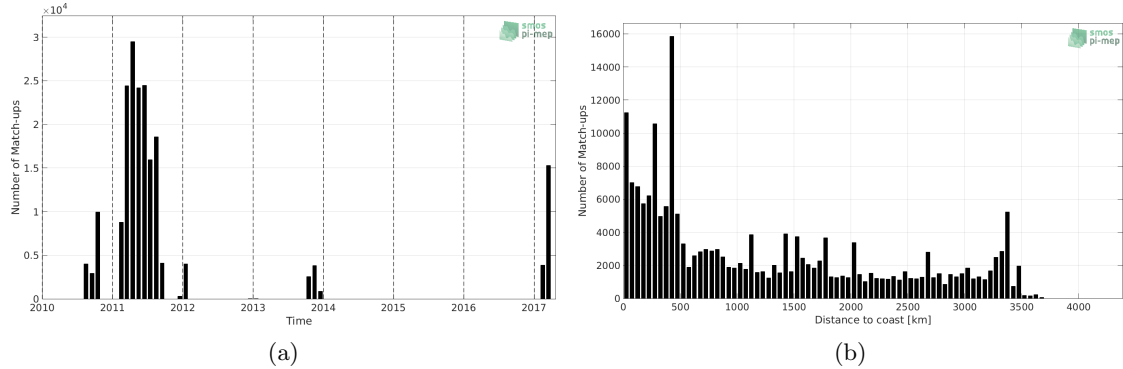
Figure 1: Number of match-ups between TSG (GOSUD-Sailing-ship) and SMOS SSS L3 v7 - 9 Days (CATDS-CECOS-LOCEAN) SSS as a function of time (a) and as function of the distance to coast (b) over the South Pacific Ocean Pi-MEP region and for the full satellite product period.
