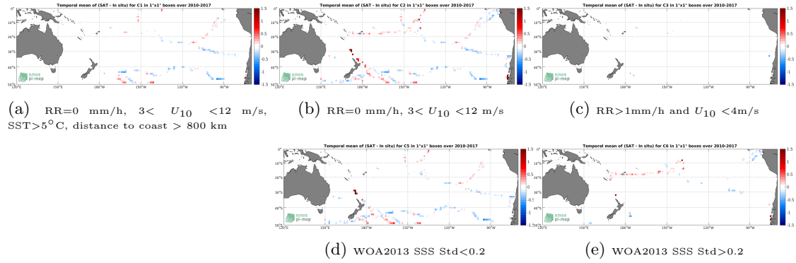
Figure 12: Temporal mean gridded over spatial boxes of size 1^\circ \times 1^\circ of \Delta SSS (SMOS SSS L3 v7 - 9 Days (CATDS-CECOS-LOCEAN) - TSG (GOSUD-Sailing-ship)) for 5 different subdatasets corresponding to: RR=0 mm/h, 3 < U_{10} < 12 m/s, SST >5^\circ\text{C} , distance to coast > 800 km (a), RR=0 mm/h, 3 < U_{10} < 12 m/s (b), RR>1\text{mm/h} and U_{10} < 4\text{m/s} (c), WOA2013 SSS Std <0.2 (d), WOA2013 SSS Std >0.2 (e).
