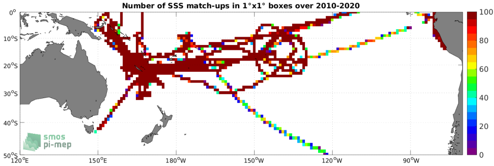
Figure 4: Number of SSS match-ups between TSG (GOSUD-Research-vessel) SSS and the SMOS SSS L3 v7 - 9 Days (CATDS-CECOS-LOCEAN) SSS product for the South Pacific Ocean Pi-MEP region over 1^\circ \times 1^\circ boxes and for the full satellite product period.
