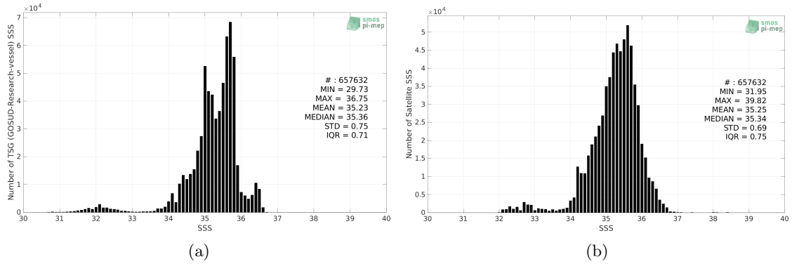
Figure 2: Histograms of SSS from TSG (GOSUD-Research-vessel) (a) and SMOS SSS L3 v7 - 9 Days (CATDS-CECOS-LOCEAN) (b) considering all match-up pairs per bins of 0.1 over the South Pacific Ocean Pi-MEP region and for the full satellite product period.
