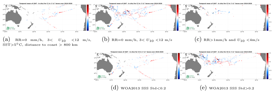
Figure 12: Temporal mean gridded over spatial boxes of size 1^\circ \times 1^\circ of \Delta\text{SSS} (SMOS SSS L3 v7 - 9 Days (CATDS-CECOS-LOCEAN) - TSG (GOSUD-Research-vessel)) for 5 different subdatasets corresponding to:RR=0 mm/h, 3 < U_{10} < 12 m/s, SST>5°C, distance to coast > 800 km (a), RR=0 mm/h, 3 < U_{10} < 12 m/s (b), RR>1mm/h and U_{10} < 4 m/s (c), WOA2013 SSS Std<0.2 (d), WOA2013 SSS Std>0.2 (e).
