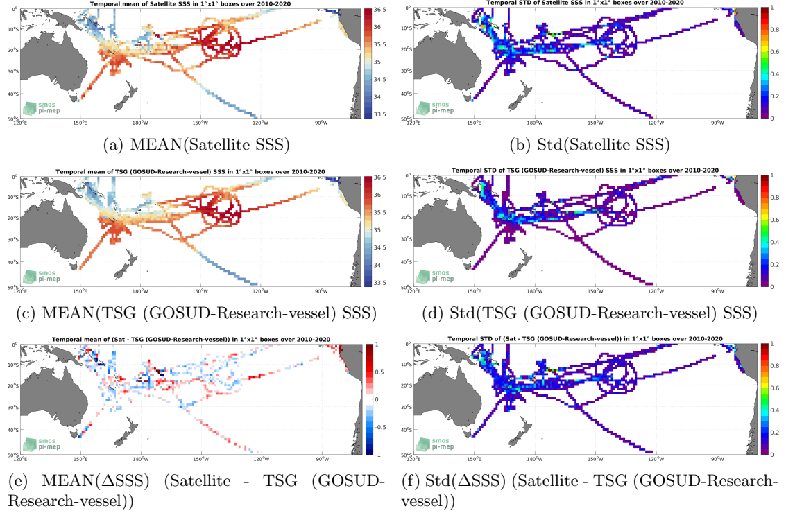
Figure 6: Temporal mean (left) and Std (right) of SSS from SMOS SSS L3 v7 - 9 Days (CATDS-CECOS-LOCEAN) (top), TSG (GOSUD-Research-vessel) (middle), and of \Delta SSS (Satellite - TSG (GOSUD-Research-vessel)). Only match-up pairs are used to generate these maps.
