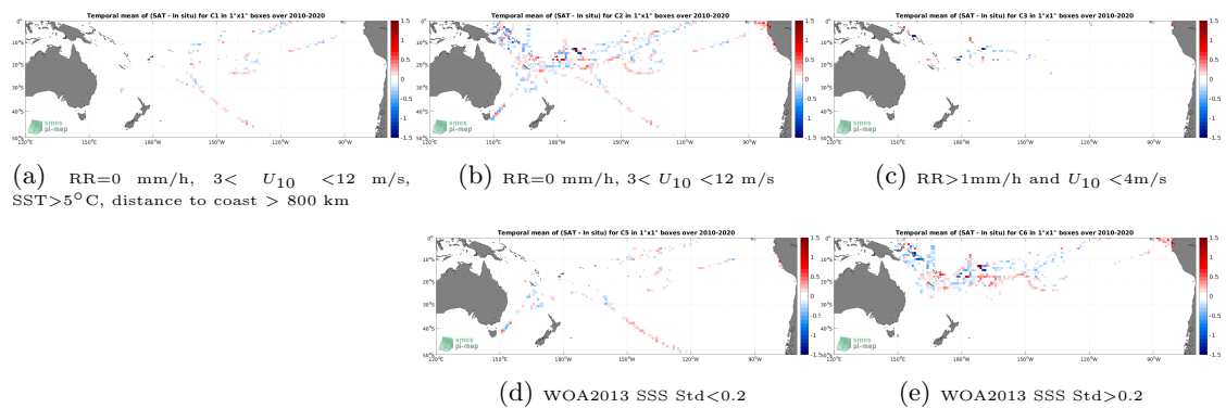
Figure 12: Temporal mean gridded over spatial boxes of size 1^\circ \times 1^\circ of \Delta SSS (SMOS SSS L3 v7 - 9 Days (CATDS-CECOS-LOCEAN) - TSG (GOSUD-Research-vessel)) for 5 different subdatasets corresponding to:RR=0 mm/h, 3 < U_{10} < 12 m/s, SST>5°C, distance to coast > 800 km (a), RR=0 mm/h, 3 < U_{10} < 12 m/s (b), RR>1mm/h and U_{10} < 4 m/s (c), WOA2013 SSS Std<0.2 (d), WOA2013 SSS Std>0.2 (e).
