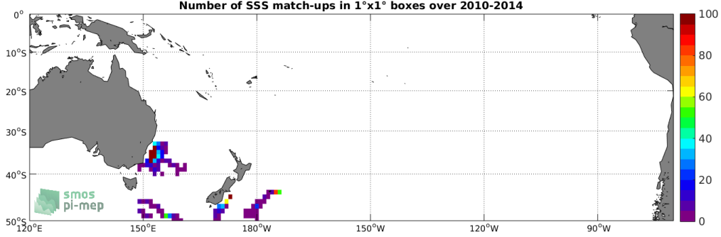
Figure 4: Number of SSS match-ups between Marine mammals SSS and the SMOS SSS L3 v7 - 9 Days (CATDS-CECOS-LOCEAN) SSS product for the South Pacific Ocean Pi-MEP region over 1^\circ \times 1^\circ boxes and for the full satellite product period.
