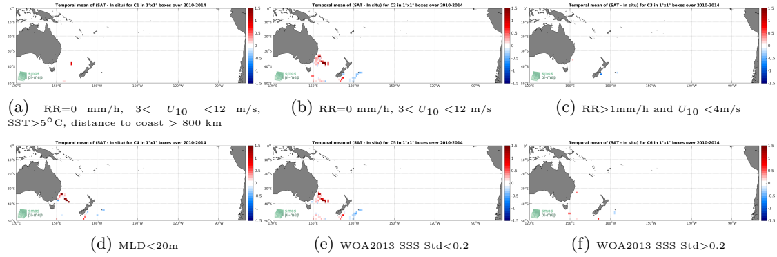
Figure 12: Temporal mean gridded over spatial boxes of size 1^{\circ}\times 1^{\circ} of \Delta\text{SSS} (SMOS SSS L3 v7 - 9 Days (CATDS-CECOS-LOCEAN) - Marine mammals) for 6 different subdatasets corresponding to: \text{RR}=0 mm/h, 3 < U_{10} < 12 m/s, \text{SST} > 5^{\circ}\text{C} , distance to coast > 800 km (a), \text{RR}=0 mm/h, 3 < U_{10} < 12 m/s (b), \text{RR} > 1\text{mm/h} and U_{10} < 4\text{m/s} (c), \text{MLD} < 20\text{m} (d), \text{WOA2013 SSS Std} < 0.2 (e), \text{WOA2013 SSS Std} > 0.2 (f).
