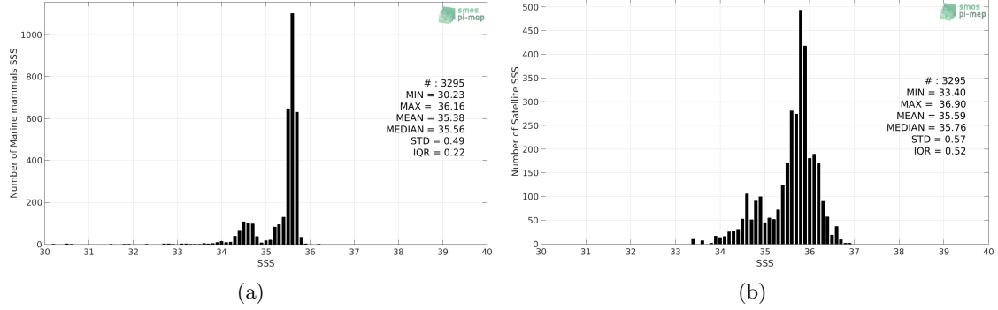
Figure 2: Histograms of SSS from Marine mammals (a) and SMOS SSS L3 v7 - 9 Days (CATDS-CECOS-LOCEAN) (b) considering all match-up pairs per bins of 0.1 over the South Pacific Ocean Pi-MEP region and for the full satellite product period.
