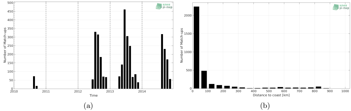
Figure 1: Number of match-ups between Marine mammals and SMOS SSS L3 v7 - 9 Days (CATDS-CECOS-LOCEAN) SSS as a function of time (a) and as function of the distance to coast (b) over the South Pacific Ocean Pi-MEP region and for the full satellite product period.
