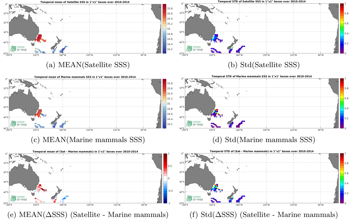
Figure 6: Temporal mean (left) and Std (right) of SSS from SMOS SSS L3 v7 - 9 Days (CATDS-CECOS-LOCEAN) (top), Marine mammals (middle), and of \Delta SSS (Satellite - Marine mammals). Only match-up pairs are used to generate these maps.
