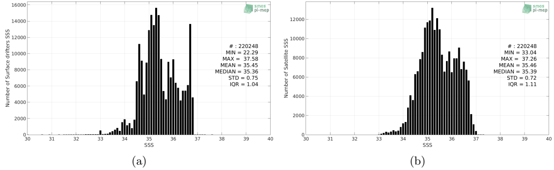
Figure 2: Histograms of SSS from Surface drifters (a) and SMOS SSS L3 v7 - 9 Days (CATDS-CECOS-LOCEAN) (b) considering all match-up pairs per bins of 0.1 over the South Pacific Ocean Pi-MEP region and for the full satellite product period.
