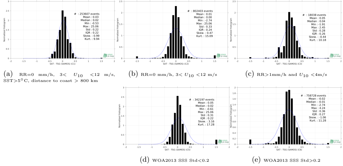
Figure 13: Normalized histogram of \Delta SSS (SMOS SSS L3 v7 - 18 Days (CATDS-CECOS-LOCEAN) - TSG (SAMOS)) for 5 different subdatasets corresponding to: RR=0 mm/h, 3 < U_{10} < 12 m/s, SST>5°C, distance to coast > 800 km (a), RR=0 mm/h, 3 < U_{10} < 12 m/s (b), RR>1mm/h and U_{10} < 4 m/s (c), WOA2013 SSS Std<0.2 (d), WOA2013 SSS Std>0.2 (e).
