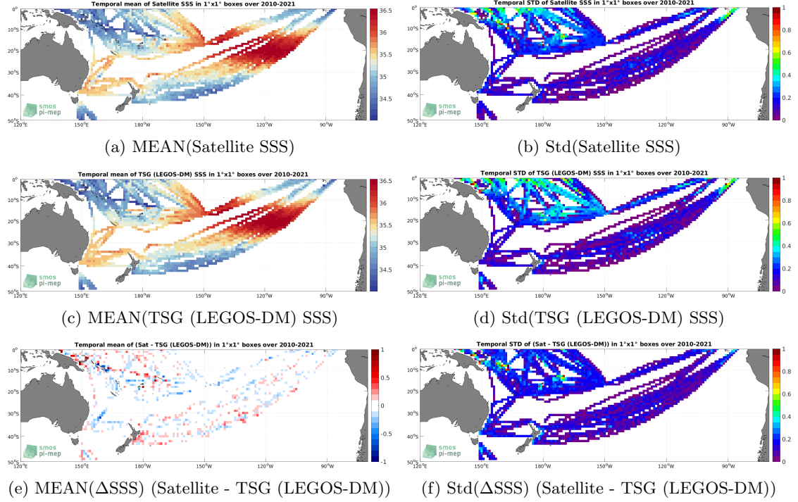
Figure 6: Temporal mean (left) and Std (right) of SSS from SMOS SSS L3 v7 - 18 Days (CATDS-CECOS-LOCEAN) (top), TSG (LEGOS-DM) ( in situ ) dataset (middle), and of \Delta SSS (Satellite - TSG (LEGOS-DM)). Only match-up pairs are used to generate these maps.
