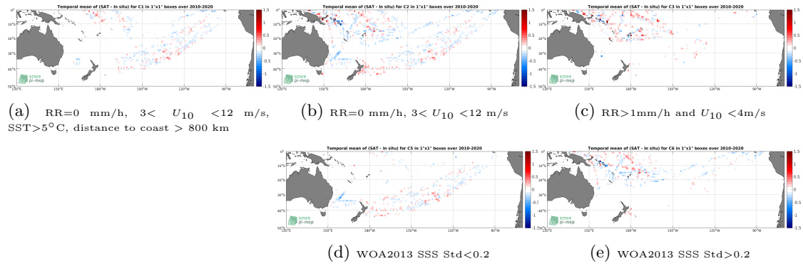
Figure 12: Temporal mean gridded over spatial boxes of size 1^\circ \times 1^\circ of \Delta SSS (SMOS SSS L3 v7 - 18 Days (CATDS-CECOS-LOCEAN) - TSG (LEGOS-DM)) for 5 different subdatasets corresponding to: RR=0 mm/h, 3 < U_{10} < 12 m/s, SST >5^\circ\text{C} , distance to coast > 800 km (a), RR=0 mm/h, 3 < U_{10} < 12 m/s (b), RR>1\text{mm/h} and U_{10} < 4\text{m/s} (c), WOA2013 SSS Std <0.2 (d), WOA2013 SSS Std >0.2 (e).
