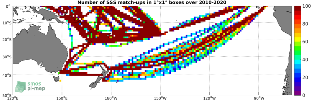
Figure 4: Number of SSS match-ups between TSG (LEGOS-DM) SSS and the SMOS SSS L3 v7 - 18 Days (CATDS-CECOS-LOCEAN) SSS product for the South Pacific Ocean Pi-MEP region over 1^\circ \times 1^\circ boxes and for the full satellite product period.
