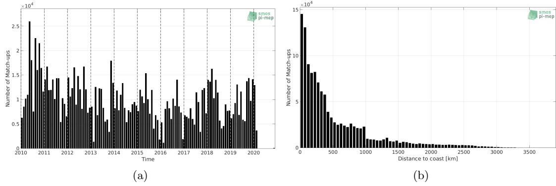
Figure 1: Number of match-ups between TSG (LEGOS-DM) and SMOS SSS L3 v7 - 18 Days (CATDS-CECOS-LOCEAN) SSS as a function of time (a) and as function of the distance to coast (b) over the South Pacific Ocean Pi-MEP region and for the full satellite product period.
