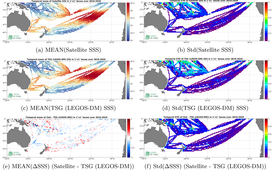
Figure 6: Temporal mean (left) and Std (right) of SSS from SMOS SSS L3 v7 - 18 Days (CATDS-CECOS-LOCEAN) (top), TSG (LEGOS-DM) (middle), and of \Delta\text{SSS} (Satellite - TSG (LEGOS-DM)). Only match-up pairs are used to generate these maps.
