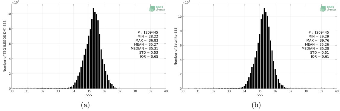
Figure 2: Histograms of SSS from TSG (LEGOS-DM) (a) and SMOS SSS L3 v7 - 18 Days (CATDS-CECOS-LOCEAN) (b) considering all match-up pairs per bins of 0.1 over the South Pacific Ocean Pi-MEP region and for the full satellite product period.
