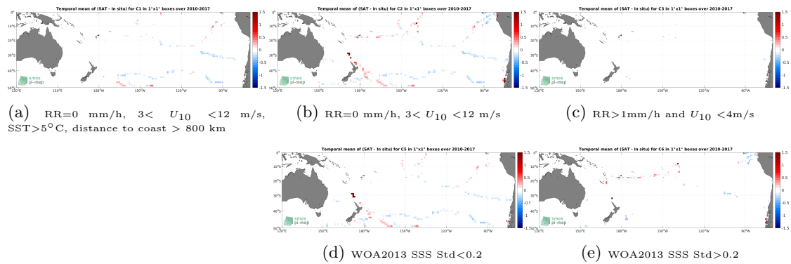
Figure 12: Temporal mean gridded over spatial boxes of size 1^\circ \times 1^\circ of \Delta SSS (SMOS SSS L3 v7 - 18 Days (CATDS-CECOS-LOCEAN) - TSG (GOSUD-Sailing-ship)) for 5 different subdatasets corresponding to:RR=0 mm/h, 3 < U_{10} < 12 m/s, SST >5^\circ C, distance to coast > 800 km (a), RR=0 mm/h, 3 < U_{10} < 12 m/s (b), RR >1 mm/h and U_{10} < 4 m/s (c), WOA2013 SSS Std <0.2 (d), WOA2013 SSS Std >0.2 (e).
