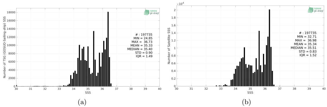
Figure 2: Histograms of SSS from TSG (GOSUD-Sailing-ship) (a) and SMOS SSS L3 v7 - 18 Days (CATDS-CECOS-LOCEAN) (b) considering all match-up pairs per bins of 0.1 over the South Pacific Ocean Pi-MEP region and for the full satellite product period.
