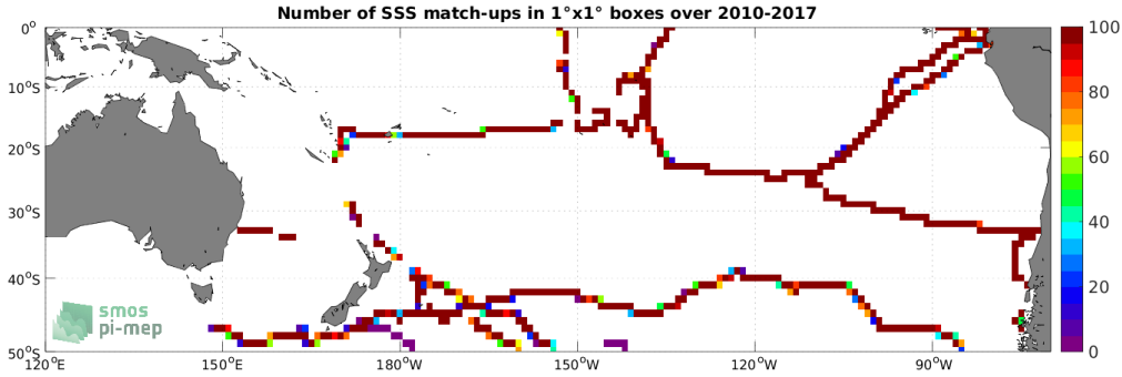
Figure 4: Number of SSS match-ups between TSG (GOSUD-Sailing-ship) SSS and the SMOS SSS L3 v7 - 18 Days (CATDS-CECOS-LOCEAN) SSS product for the South Pacific Ocean Pi-MEP region over 1^\circ \times 1^\circ boxes and for the full satellite product period.
