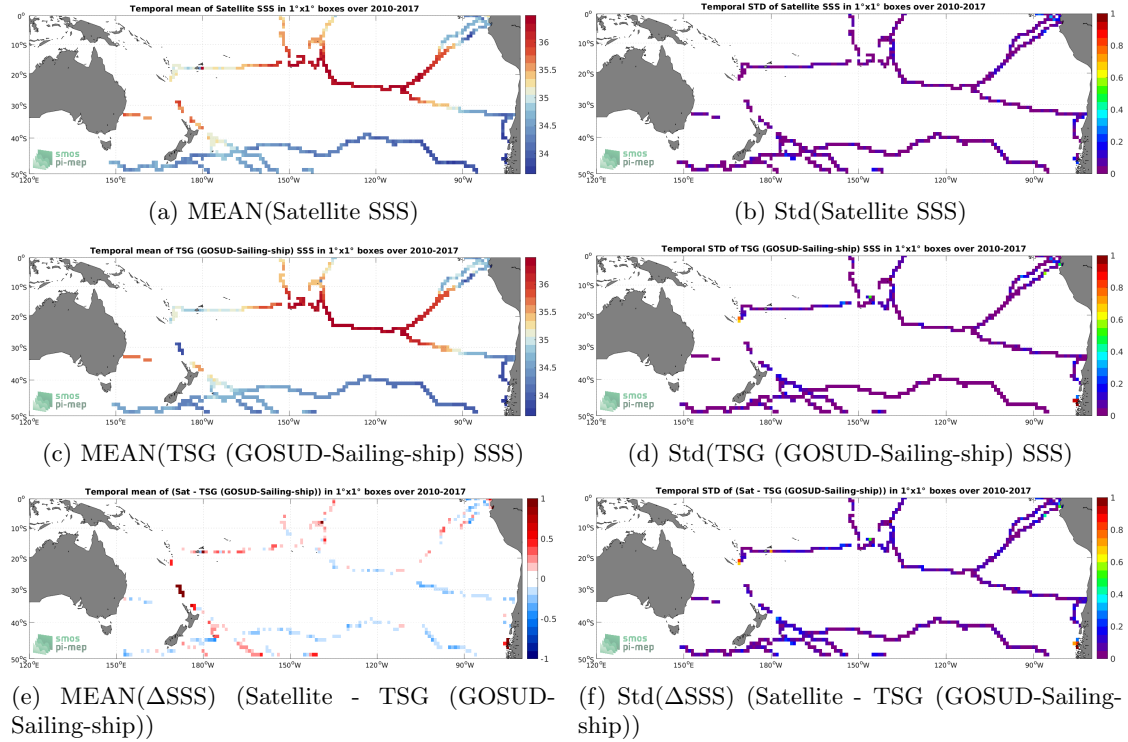
Figure 6: Temporal mean (left) and Std (right) of SSS from SMOS SSS L3 v7 - 18 Days (CATDS-CECOS-LOCEAN) (top), TSG (GOSUD-Sailing-ship) (middle), and of \Delta SSS (Satellite - TSG (GOSUD-Sailing-ship)). Only match-up pairs are used to generate these maps.
