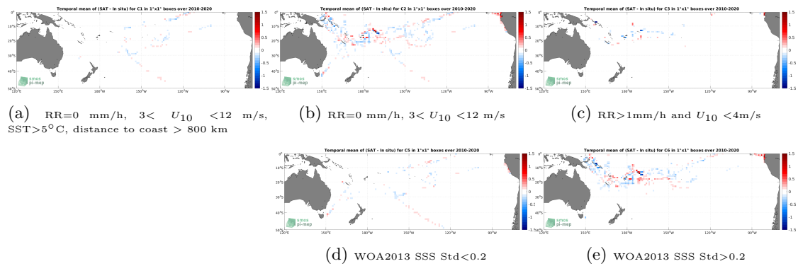
Figure 12: Temporal mean gridded over spatial boxes of size 1^\circ \times 1^\circ of \Delta\text{SSS} (SMOS SSS L3 v7 - 18 Days (CATDS-CECOS-LOCEAN) - TSG (GOSUD-Research-vessel)) for 5 different sub-datasets corresponding to:RR=0 mm/h, 3 < U_{10} < 12 m/s, SST>5°C, distance to coast > 800 km (a), RR=0 mm/h, 3 < U_{10} < 12 m/s (b), RR>1mm/h and U_{10} < 4 m/s (c), WOA2013 SSS Std<0.2 (d), WOA2013 SSS Std>0.2 (e).
