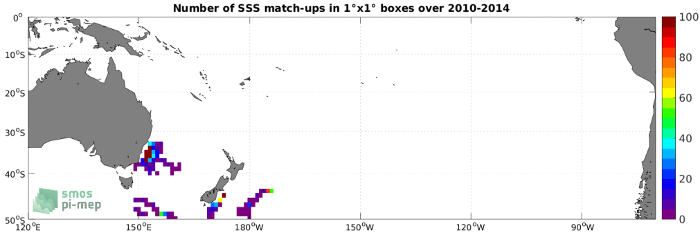
Figure 4: Number of SSS match-ups between Marine mammals SSS and the SMOS SSS L3 v7 - 18 Days (CATDS-CECOS-LOCEAN) SSS product for the South Pacific Ocean Pi-MEP region over 1^\circ \times 1^\circ boxes and for the full satellite product period.
