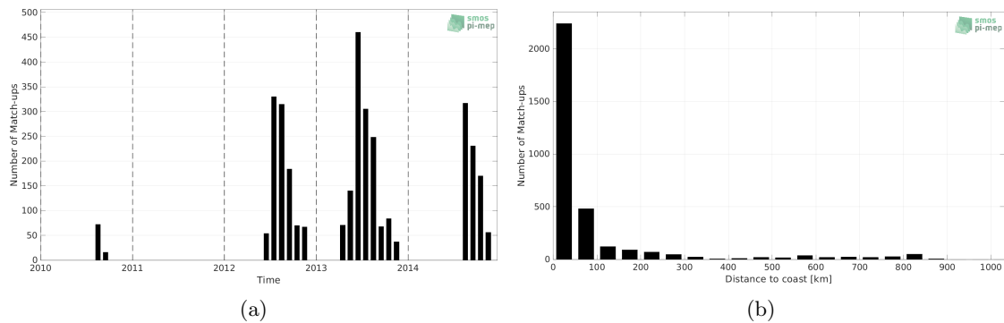
Figure 1: Number of match-ups between Marine mammals and SMOS SSS L3 v7 - 18 Days (CATDS-CECOS-LOCEAN) SSS as a function of time (a) and as function of the distance to coast (b) over the South Pacific Ocean Pi-MEP region and for the full satellite product period.
