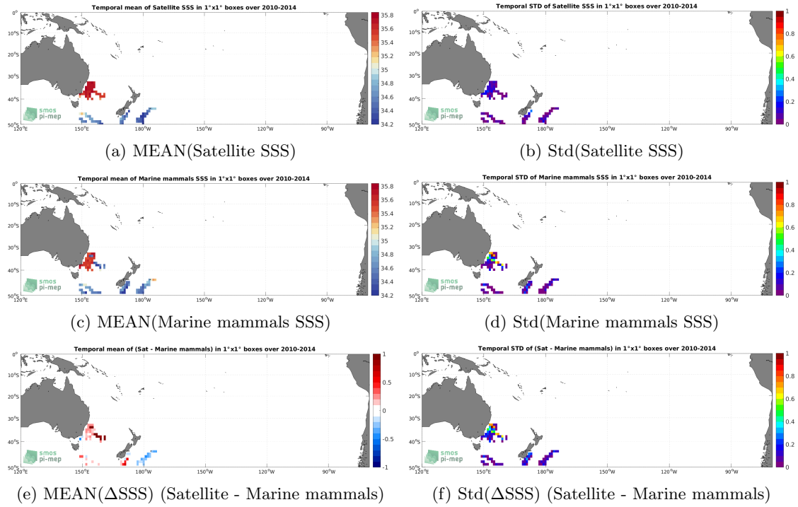
Figure 6: Temporal mean (left) and Std (right) of SSS from SMOS SSS L3 v7 - 18 Days (CATDS-CECOS-LOCEAN) (top), Marine mammals (middle), and of \Delta SSS (Satellite - Marine mammals). Only match-up pairs are used to generate these maps.
