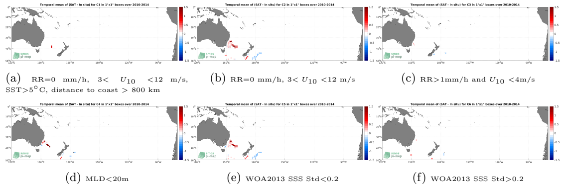
Figure 12: Temporal mean gridded over spatial boxes of size 1^{\circ}\times 1^{\circ} of \Delta\text{SSS} (SMOS SSS L3 v7 - 18 Days (CATDS-CECOS-LOCEAN) - Marine mammals) for 6 different subdatasets corresponding to:RR=0 mm/h, 3 < U_{10} < 12 m/s, SST >5^{\circ}\text{C} , distance to coast > 800 km (a), RR=0 mm/h, 3 < U_{10} < 12 m/s (b), RR >1\text{mm/h} and U_{10} < 4\text{m/s} (c),MLD <20\text{m} (d),WOA2013 SSS Std <0.2 (e),WOA2013 SSS Std >0.2 (f).
