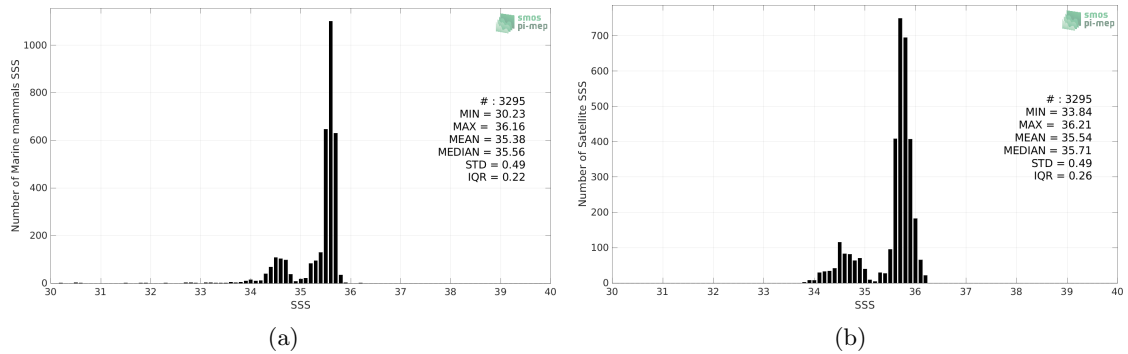
Figure 2: Histograms of SSS from Marine mammals (a) and SMOS SSS L3 v7 - 18 Days (CATDS-CECOS-LOCEAN) (b) considering all match-up pairs per bins of 0.1 over the South Pacific Ocean Pi-MEP region and for the full satellite product period.
