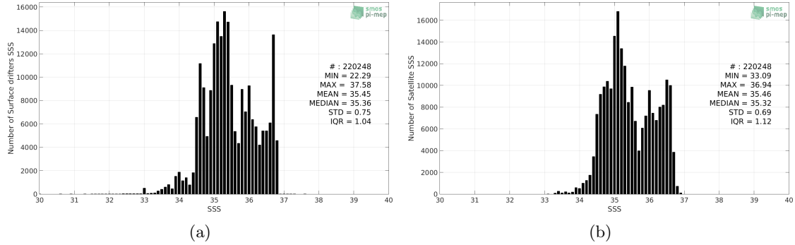
Figure 2: Histograms of SSS from Surface drifters (a) and SMOS SSS L3 v7 - 18 Days (CATDS-CECOS-LOCEAN) (b) considering all match-up pairs per bins of 0.1 over the South Pacific Ocean Pi-MEP region and for the full satellite product period.
