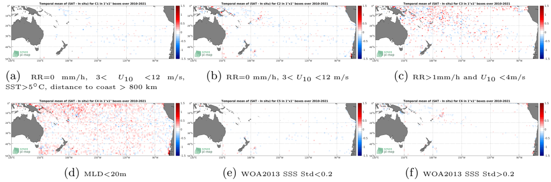
Figure 12: Temporal mean gridded over spatial boxes of size 1^\circ \times 1^\circ of \Delta SSS (SMOS SSS L3 v7 - 18 Days (CATDS-CECOS-LOCEAN) - Argo) for 6 different subdatasets corresponding to: RR=0 mm/h, 3 < U_{10} < 12 m/s, SST > 5^\circ C , distance to coast > 800 km (a), RR=0 mm/h, 3 < U_{10} < 12 m/s (b), RR > 1 mm/h and U_{10} < 4 m/s (c), MLD < 20 m (d), WOA2013 SSS Std < 0.2 (e), WOA2013 SSS Std > 0.2 (f).
