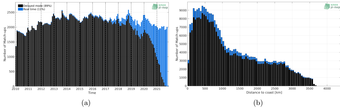
Figure 1: Number of match-ups between Argo and SMOS SSS L3 v7 - 18 Days (CATDS-CECOS-LOCEAN) SSS as a function of time (a) and as function of the distance to coast (b) over the South Pacific Ocean Pi-MEP region and for the full satellite product period.
