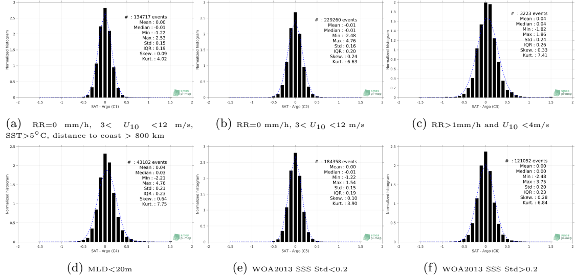
Figure 13: Normalized histogram of \Delta\text{SSS} (SMOS SSS L3 v7 - 18 Days (CATDS-CECOS-LOCEAN) - Argo) for 6 different subdatasets corresponding to: RR=0 mm/h, 3 < U_{10} < 12 m/s, SST>5°C, distance to coast > 800 km (a), RR=0 mm/h, 3 < U_{10} < 12 m/s (b), RR>1mm/h and U_{10} < 4 m/s (c), MLD<20m (d), WOA2013 SSS Std<0.2 (e), WOA2013 SSS Std>0.2 (f).
