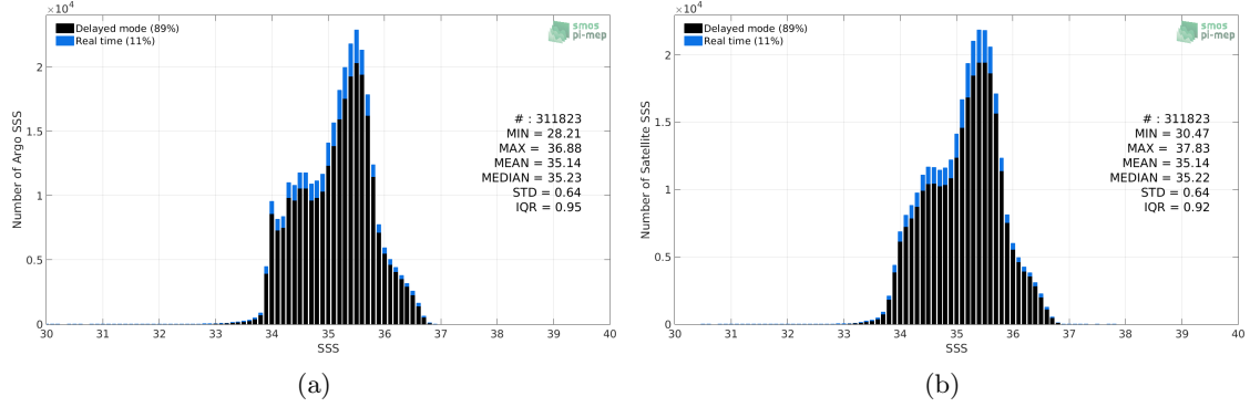
Figure 2: Histograms of SSS from Argo (a) and SMOS SSS L3 v7 - 18 Days (CATDS-CECOS-LOCEAN) (b) considering all match-up pairs per bins of 0.1 over the South Pacific Ocean Pi-MEP region and for the full satellite product period.
