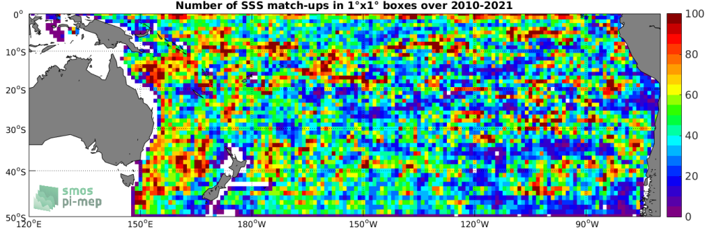
Figure 4: Number of SSS match-ups between Argo SSS and the SMOS SSS L3 v7 - 18 Days (CATDS-CECOS-LOCEAN) SSS product for the South Pacific Ocean Pi-MEP region over 1^\circ \times 1^\circ boxes and for the full satellite product period.
