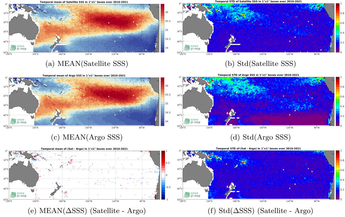
Figure 6: Temporal mean (left) and Std (right) of SSS from SMOS SSS L3 v7 - 18 Days (CATDS-CECOS-LOCEAN) (top), Argo (middle), and of \Delta SSS (Satellite - Argo). Only match-up pairs are used to generate these maps.
