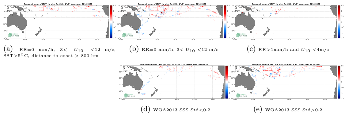
Figure 12: Temporal mean gridded over spatial boxes of size 1^\circ \times 1^\circ of \Delta SSS (SMOS SSS L3 v5 - 9 Days (CATDS-CECOS-LOCEAN) - TSG (SAMOS)) for 5 different subdatasets corresponding to:RR=0 mm/h, 3 < U_{10} < 12 m/s, SST >5^\circ\text{C} , distance to coast > 800 km (a), RR=0 mm/h, 3 < U_{10} < 12 m/s (b), RR >1 mm/h and U_{10} < 4 m/s (c), WOA2013 SSS Std <0.2 (d), WOA2013 SSS Std >0.2 (e).
