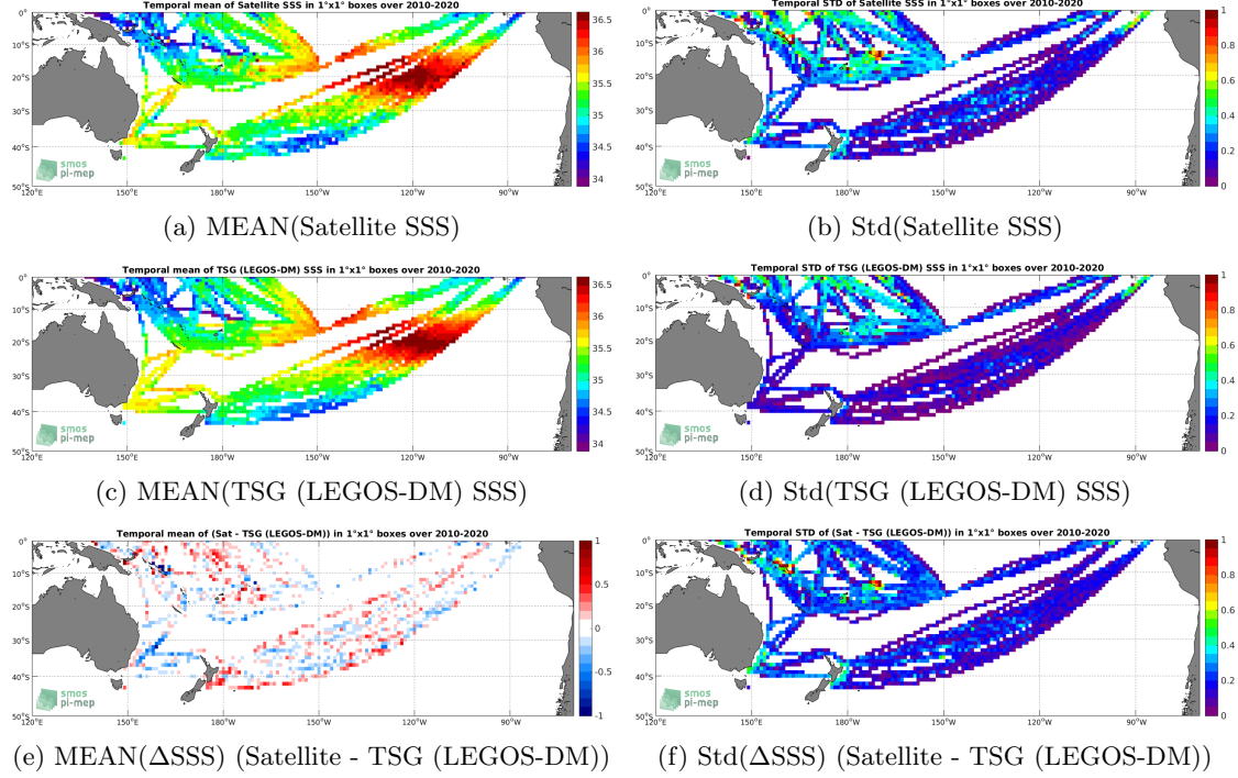
Figure 6: Temporal mean (left) and Std (right) of SSS from SMOS SSS L3 v5 - 9 Days (CATDS-CECOS-LOCEAN) (top), TSG (LEGOS-DM) (middle), and of \Delta\text{SSS} (Satellite - TSG (LEGOS-DM)). Only match-up pairs are used to generate these maps.
