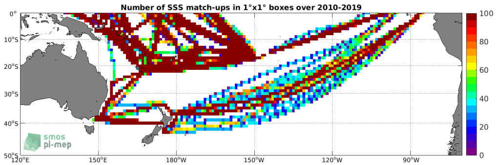
Figure 4: Number of SSS match-ups between TSG (LEGOS-DM) SSS and the SMOS SSS L3 v5 - 9 Days (CATDS-CECOS-LOCEAN) SSS product for the South Pacific Ocean Pi-MEP region over 1°x1° boxes and for the full satellite product period.
