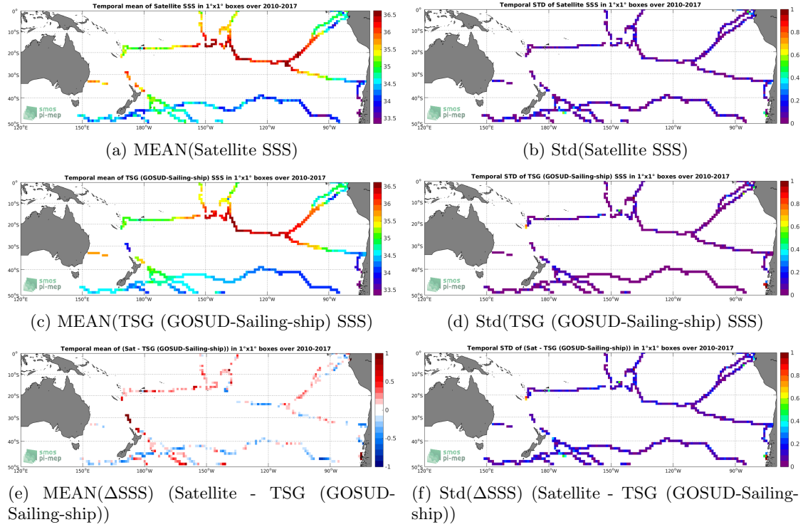
Figure 6: Temporal mean (left) and Std (right) of SSS from SMOS SSS L3 v5 - 9 Days (CATDS-CECOS-LOCEAN) (top), TSG (GOSUD-Sailing-ship) (middle), and of \Delta SSS (Satellite - TSG (GOSUD-Sailing-ship)). Only match-up pairs are used to generate these maps.
