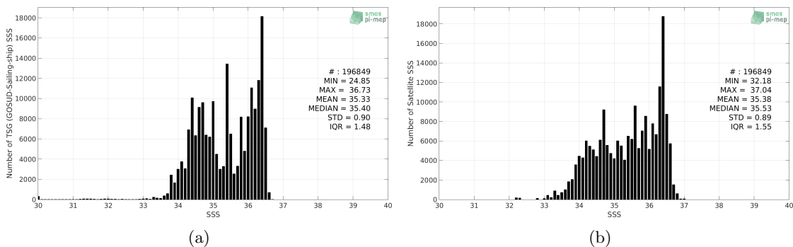
Figure 2: Histograms of SSS from TSG (GOSUD-Sailing-ship) (a) and SMOS SSS L3 v5 - 9 Days (CATDS-CECOS-LOCEAN) (b) considering all match-up pairs per bins of 0.1 over the South Pacific Ocean Pi-MEP region and for the full satellite product period.
