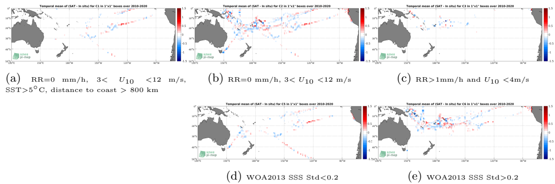
Figure 12: Temporal mean gridded over spatial boxes of size 1^\circ \times 1^\circ of \Delta\text{SSS} (SMOS SSS L3 v5 - 9 Days (CATDS-CECOS-LOCEAN) - TSG (GOSUD-Research-vessel)) for 5 different subdatasets corresponding to:RR=0 mm/h, 3 < U_{10} < 12 m/s, SST>5°C, distance to coast > 800 km (a), RR=0 mm/h, 3 < U_{10} < 12 m/s (b), RR>1mm/h and U_{10} < 4 m/s (c), WOA2013 SSS Std<0.2 (d), WOA2013 SSS Std>0.2 (e).
