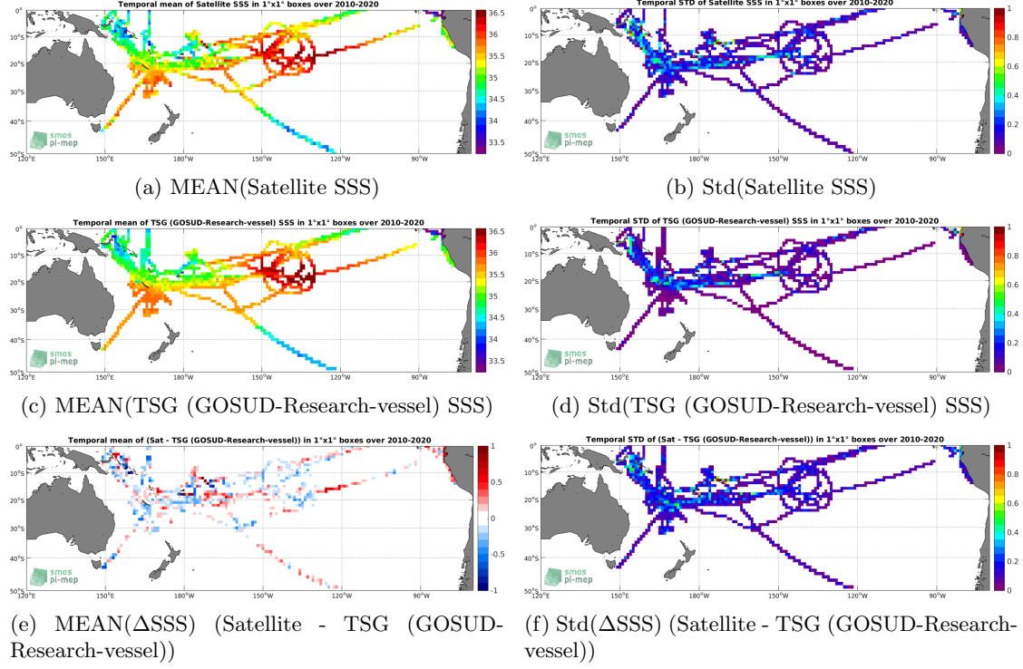
Figure 6: Temporal mean (left) and Std (right) of SSS from SMOS SSS L3 v5 - 9 Days (CATDS-CECOS-LOCEAN) (top), TSG (GOSUD-Research-vessel) (middle), and of \Delta SSS (Satellite - TSG (GOSUD-Research-vessel)). Only match-up pairs are used to generate these maps.
